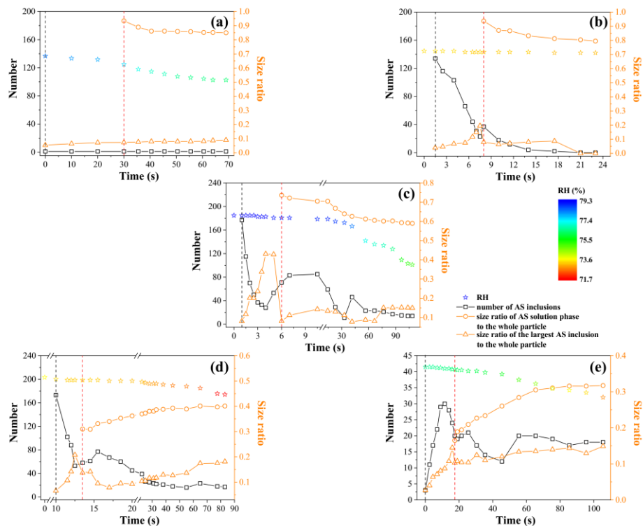
Figure 8: Temporal changes in number of AS inclusions, size ratios of AS solution phases and the largest AS inclusions to the whole particles, as well as corresponding RH during -LLPS for mixed 1, 2, 6-hexanetriol/AS particles with OIR = 1: 2-4 (a), 1: 4-2 (b), 1:1 (c), 2:1 (d) and 4:1 (e). The black dash line corresponds to the appearance of AS inclusions. The red dash line corresponds to the appearance of the AS solution phase.
