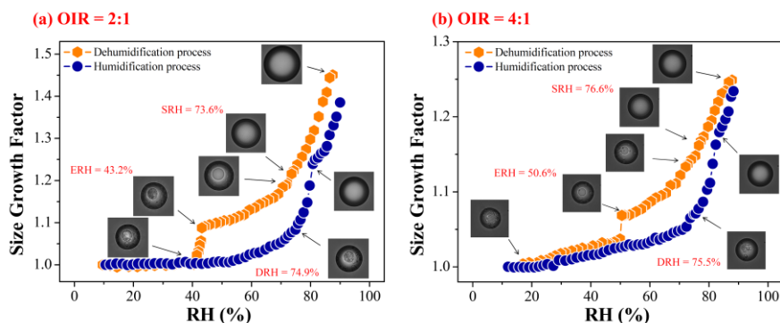
500 Figure 6: Hygroscopic cycles of mixed 1, 2, 6-hexanetriol/AS particles with OIR = 2:1 (a) and 4:1 (b). The panels show the optical images corresponding to the GFs at the certain RH. The SRH, ERH and DRH values are given in red.
