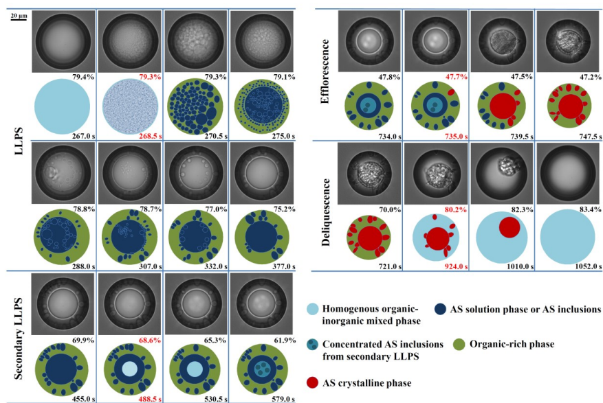
480 Figure 2: Optical images and corresponding illustrations of mixed 1, 2, 6-hexanetriol/AS particle with OIR = 1:1 during LLPS, secondary LLPS, efflorescence and deliquescence. Below the optical images are the illustrations. The corresponding RH and time are given in each frame. The RH and time in red indicate the occurrence of phase transitions.
