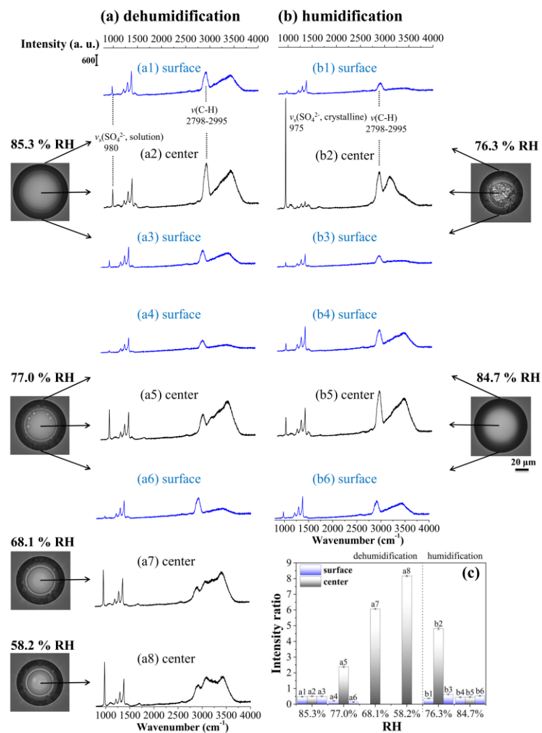
485 Figure 3: Raman spectra acquired on the surface (blue) and at the center (black) of the OIR = 1:1 particle during dehumidification (a) and humidification (b), as well as intensity ratios of \nu_3(\text{SO}_4^{2-}) band to \nu(\text{C-H}) band among all the spectra (c). Note that the value of b2 in (c) represents the intensity ratio of stretching vibration bands of crystalline \text{SO}_4^{2-} to C-H. The corresponding microscopic images are shown near the spectra.
