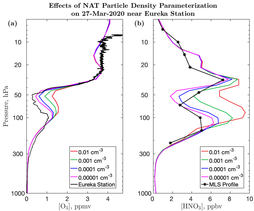
200 Figure 4. Comparison of ozone profiles (a) and nitric acid profiles (b) for four different SD-WACCM simulations at the gridpoint nearest Eureka Station for March 27 th , 2020, with ozonesonde data from Eureka Station shown for comparison in (a) and the nearest MLS profile on that day shown for comparison in (b). Note that MLS has very few levels in the lower stratosphere, shown by black points. This is the same date as shown in Figure 2b, and the magenta ozone profile corresponds to the dotted teal ozone profile shown in that figure.
