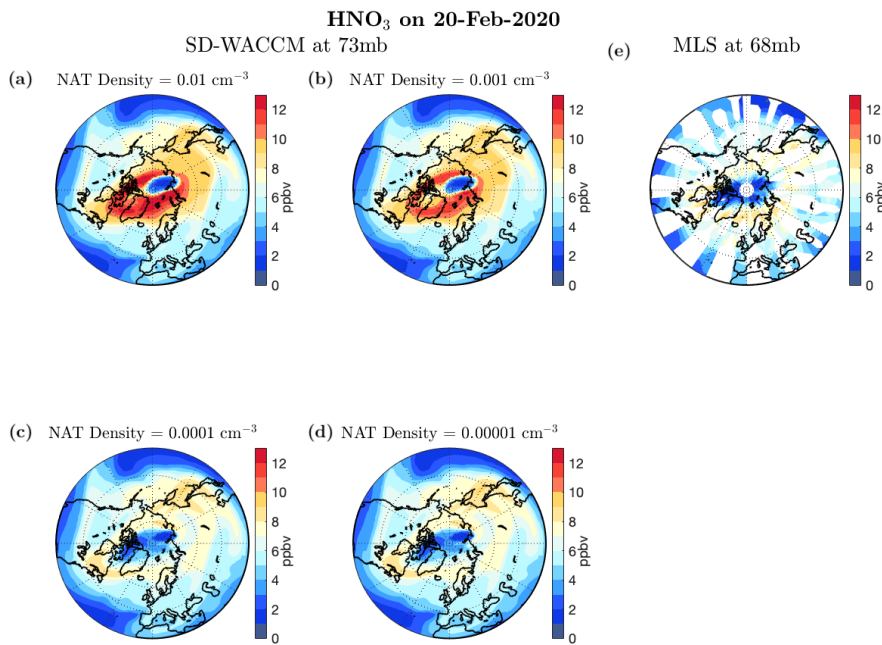
195 Figure 3. HNO 3 in ppbv for February 20 th , 2020, for different NAT parameterizations in SD-WACCM (a-d) compared to MLS (e). All SD-WACCM figures show the 73 mb level; MLS shows the 68 mb level. In order of increasing denitrification, the NAT density is (a) 0.01 cm -3 , (b) 0.001 cm -3 , (c) 0.0001 cm -3 , and (d) 0.00001 cm -3 . Panel (a) shows the previous
