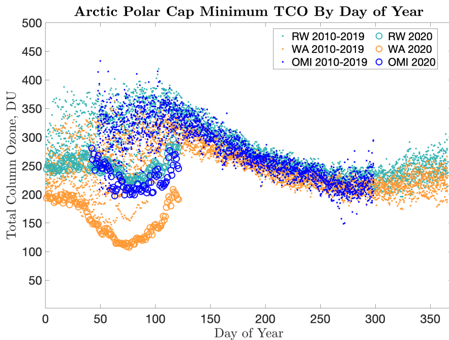
Figure 54. Minimum total column ozone simulated by SD-WACCM from 70° N to 90° N from January 2010 through the end of April 2020, plotted by day of the year. Teal markers refer to the reference run and orange markers to the world avoided run. Blue markers refer to observations by the OMI Satellite. Dots indicate days prior to 2020 from 2010-2019 and open circles indicate days in 2020.
