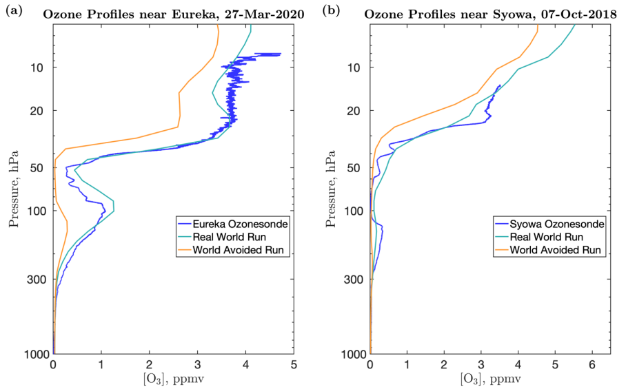
Figure 65. Comparison between the Real World (teal) and World Avoided (orange) ozone profiles in SD-WACCM at the gridpoint (a) nearest to Eureka station (80.04°N, -86.18°E) for March 27 th , 2020 and (b) nearest to Syowa station in the Antarctic (69.00°S, 39.58°E) for October 7 th , 2018. Ozone sonde profiles from the stations are shown for comparison in blue.
