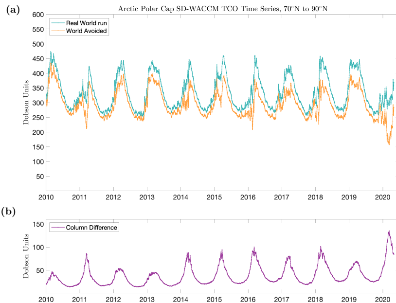
260 Figure 76. (a) Time series of mean SD-WACCM total column ozone across the polar cap for the Real World scenario (teal) and World Avoided scenario (orange) from January 2010 through April 2020. (b) The difference between the two.
