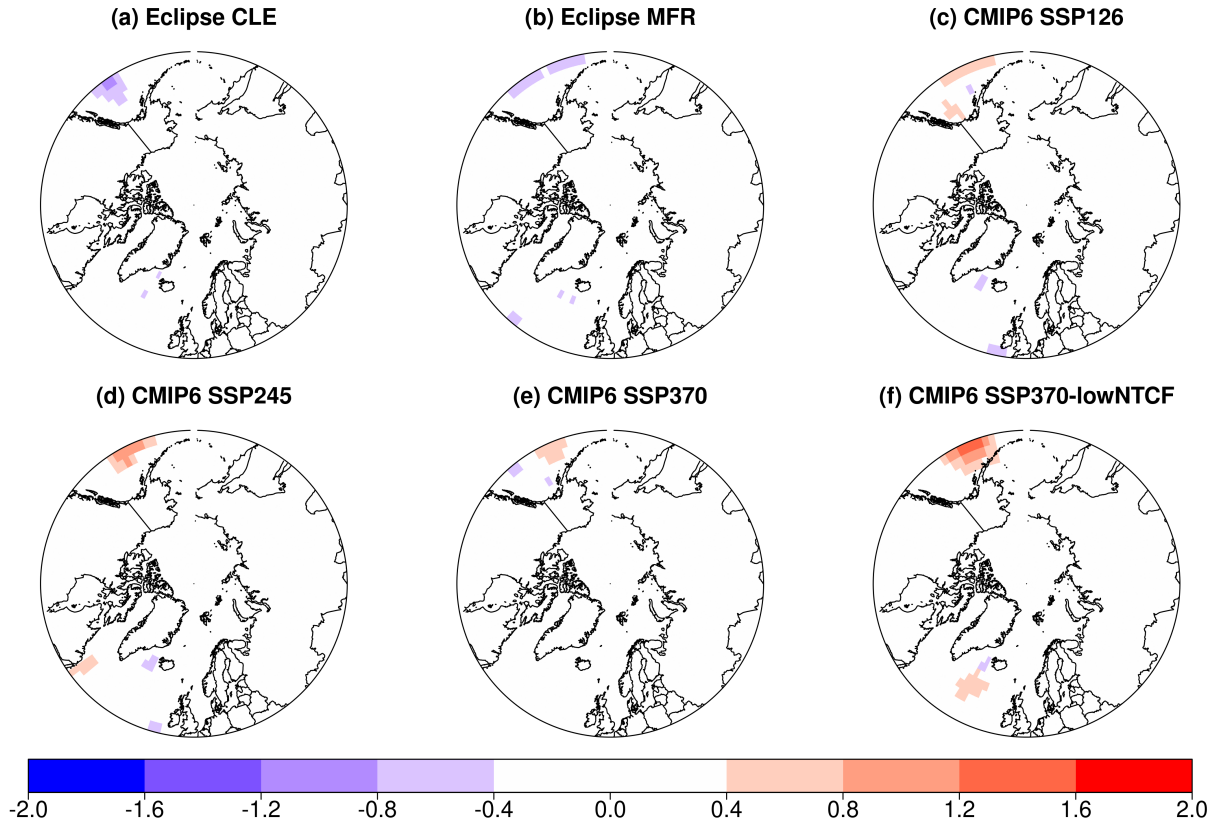
Figure S5. Spatial distribution of the September Arctic DMS emissions (Tg) change between the 1990-2010 mean and the 2030-2050 mean as calculated by the GISS-E2.1 ensemble.
