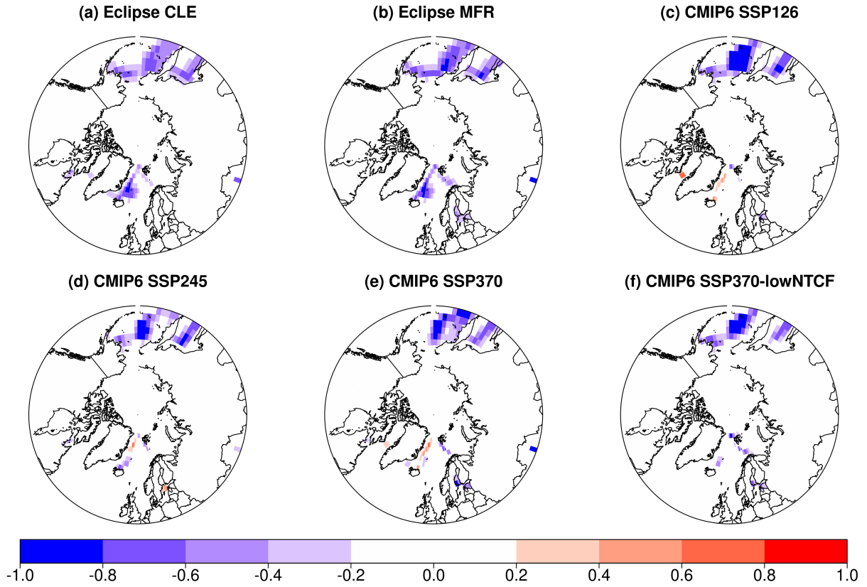
Figure S3. Spatial distribution of the March Arctic sea-ice fraction change between the 1990-2010 mean and the 2030-2050 mean as calculated by the GISS-E2.1 ensemble.
