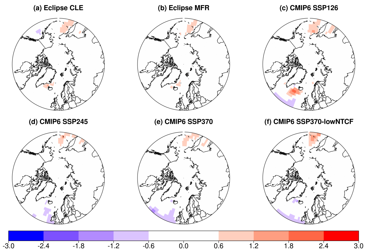
Figure S4. Spatial distribution of the March Arctic DMS emissions (Tg) change between the 1990-2010 mean and the 2030-2050 mean as calculated by the GISS-E2.1 ensemble.
