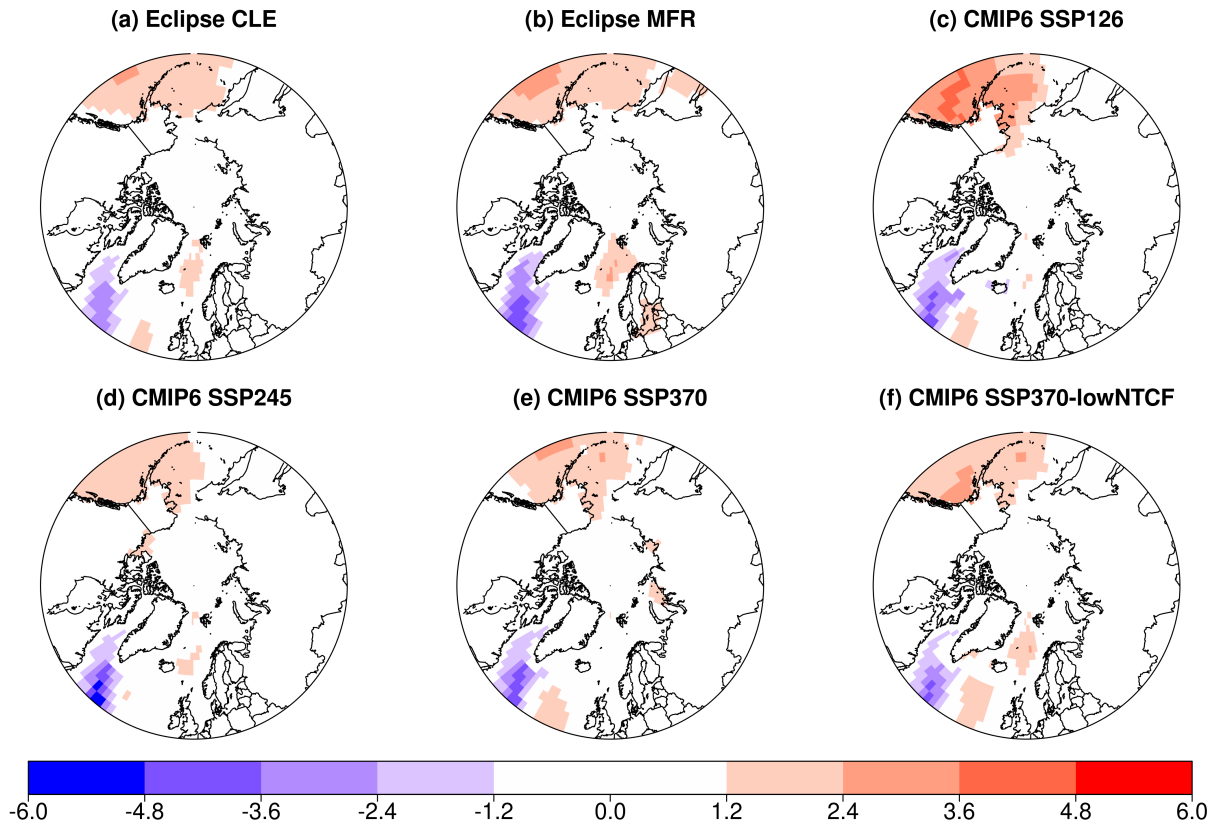
Figure S2. Spatial distribution of the annual mean Arctic sea surface temperature (°C) change between the 1990-2010 mean and the 2030-2050 mean as calculated by the GISS-E2.1 ensemble.
