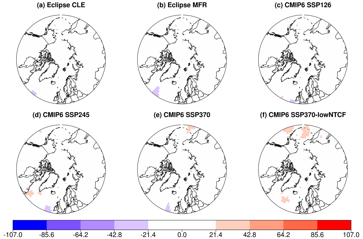
Figure S7. Spatial distribution of the September Arctic sea-salt emissions (Tg) change between the 1990-2010 mean and the 2030-2050 mean as calculated by the GISS-E2.1 ensemble.
