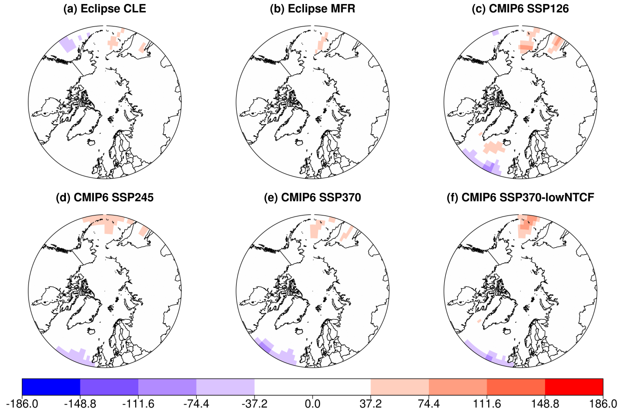
Figure S6. Spatial distribution of the March Arctic sea-salt emissions (Tg) change between the 1990-2010 mean and the 2030-2050 mean as calculated by the GISS-E2.1 ensemble.
