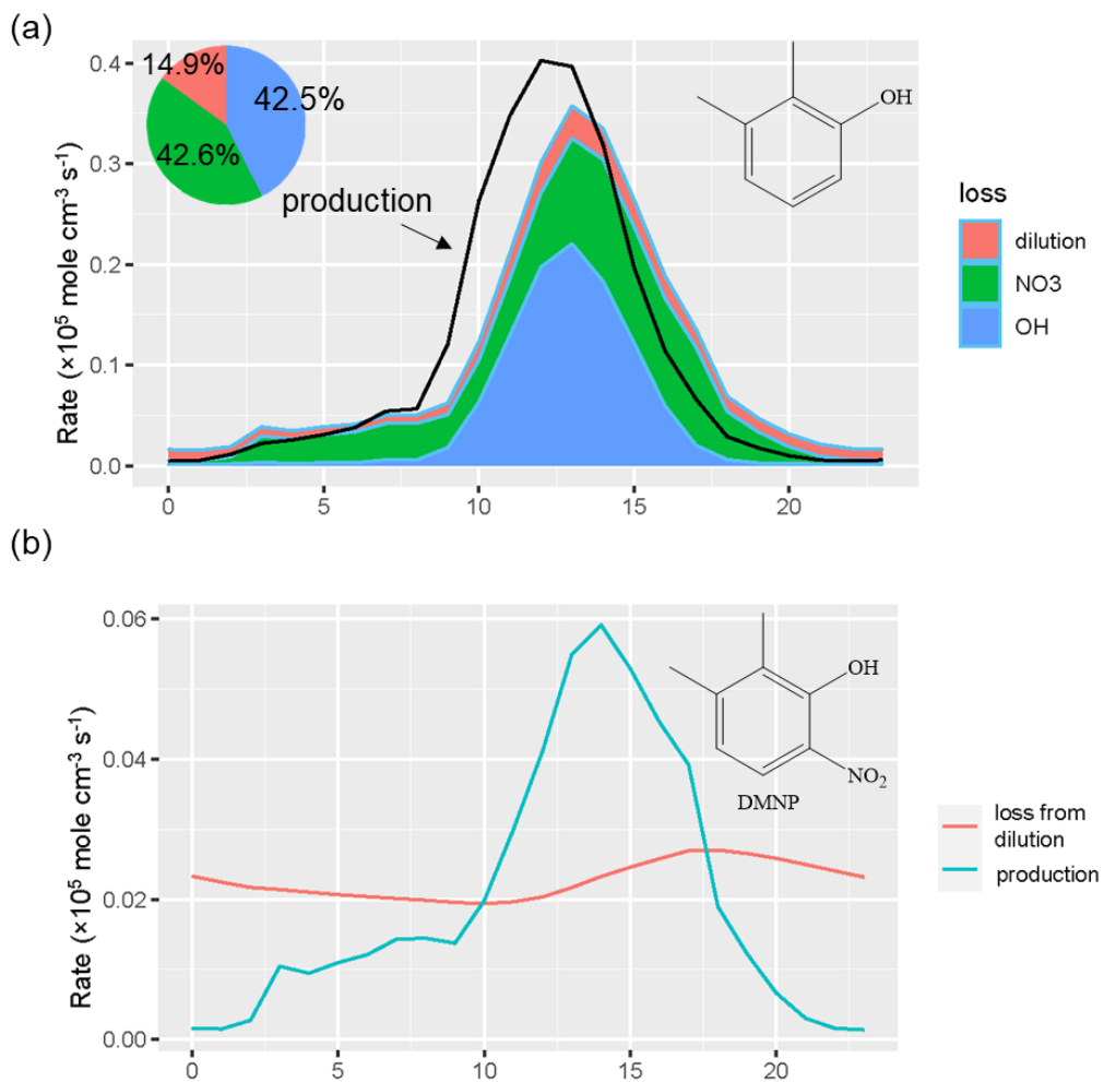
Figure 6. Production and loss of xylenol (a) and DMNP (b) during the sampling period.
