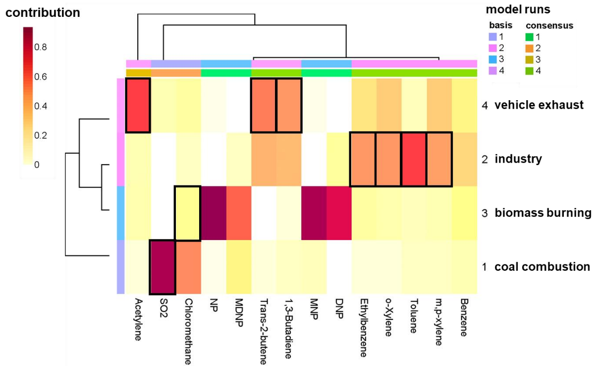
625 Figure 7. Mixture coefficients of the Kullback-Leibler (KL) algorithm with the factor number of four by non-negative matrix factorization (NMF). Factor 1: coal combustion; Factor 2: industry; Factor 3: biomass burning; Factor 4: vehicle exhaust. Basis and consensus in the legend were the model runs in which the latter one was consensus and the results were displayed in the heatmap.
