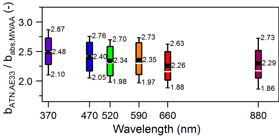
Figure A1. Wavelength-specific AE33 calibration coefficients, C(\lambda) , upon comparison of the loading-compensated AE33 attenuation with the MWAA absorption coefficient (Text 2.1.3; Text S3.1) for 27 quartz fiber filter samples from Magadino 2013 (PM 10 ) & Magadino 2014/Zurich 2013 (PM 2.5 ) [white line/box: median/IQR; black squares & whiskers: mean & 1 SD (labels)].
