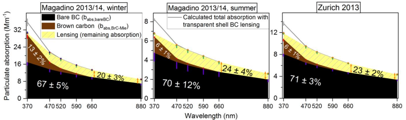
Figure 6: Optical closure results at six AE33 wavelengths (x-axis, linear scale), shown as cumulative contributions (labels) to total (calibrated) measured particulate absorption (y-axis) of the different carbonaceous aerosol species (bare BC, extractable BrC) and the filter-based BC absorption enhancement (lensing) defined as “remaining absorption”. The total measured absorption, b_{\text{abs,total}} , is indicated with the orange circles (uncertainty: upward blue error bars). Note the different ranges of b_{\text{abs}} values (y-axis) between the three cases. Orange arrows indicate the lensing contribution at longer wavelengths (660 nm, 880 nm) for the three cases, with filter-based E_{\text{abs,BC}} being equal to ( 1.35 \pm 0.10 , 1.33 \pm 0.10 ), ( 1.37 \pm 0.24 , 1.38 \pm 0.17 ) and ( 1.35 \pm 0.07 , 1.33 \pm 0.07 ) for Magadino winter, Magadino summer and Zurich, respectively. The error bars (minus direction shown; violet: BC; green: BC lensing; red: BrC) were computed by error propagation on the mean values [Eq. (C1)-(C3)] using the C_{\lambda} (Fig. A1), \text{MAC}_{\text{bareBC},660\text{nm}} (Fig. S14), \text{AAE}_{\text{bareBC}} (Fig. 4a) and b_{\text{abs,BrC-Mie}} (Text S5) relative errors (Appendix C). The gray line indicates calculated total absorption by adding the absorption by BrC and absorption by BC including transparent shell lensing (assumed to be wavelength-independent) extrapolated from 660 nm.
