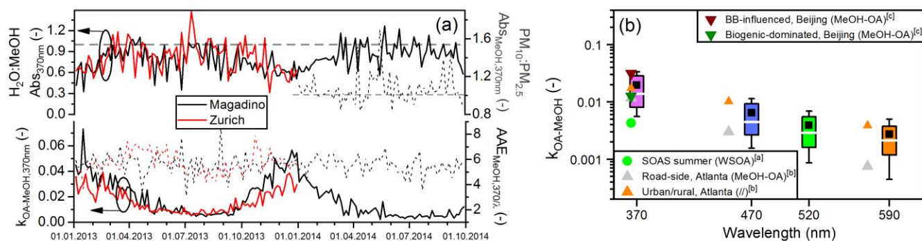
Figure 1: a) Time series at 370 nm of the water-to-methanol absorbance ( A , or Abs ) ratio (not corrected here for the solvent effect) and the \text{PM}_{10}\text{-to-PM}_{2.5} absorbance ratio in methanol (horizontal dashed lines indicate ratios of 1.0), as well as the imaginary part of refractive index ( k ) of the bulk methanol-extracted organics (Eq. (2)) and the \text{AAE}_{\text{MeOH},370/\lambda} ( \lambda=470/520/590 nm). The OA mass from AMS/PMF Solution 2 was used for all 2013 data, for a direct comparison between Magadino and Zurich. b) Box plots of the bulk mixed-source UV/Vis-based k_{\text{OA}} (total extractable OA, homogeneous and internally mixed without any inorganics or BC present) at four AE33 wavelengths, for all 245 \text{PM}_{10} samples measured from Magadino and Zurich [white line/box: median/IQR; black squares & whiskers: mean & 1 standard deviation (SD)], compared to selected literature values for bulk extracted OA [a: Washenfelder et al. (2015), b: Liu et al. (2013), c: Cheng et al. (2017); SOAS: “The Southern Oxidant and Aerosol Study”].
