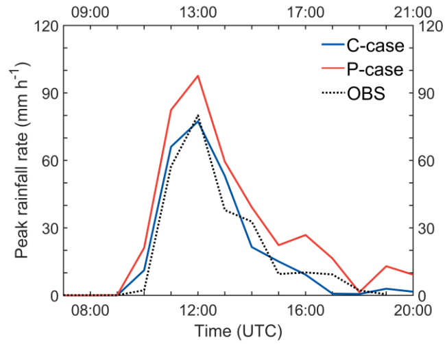
895 Figure 6 Temporal evolution of the peak rainfall rate for observation and simulations. The black dashed line represents the observation, the red line corresponds to the P-case, and the blue line corresponds to the C-case. The x-axis above is for the observation, the x-axis below is for the simulations.
