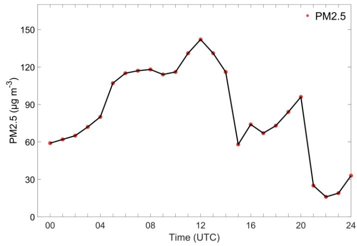
Figure 3 Hourly mass concentration of PM 2.5 on 11 August 2017 at Beijing urban area.
