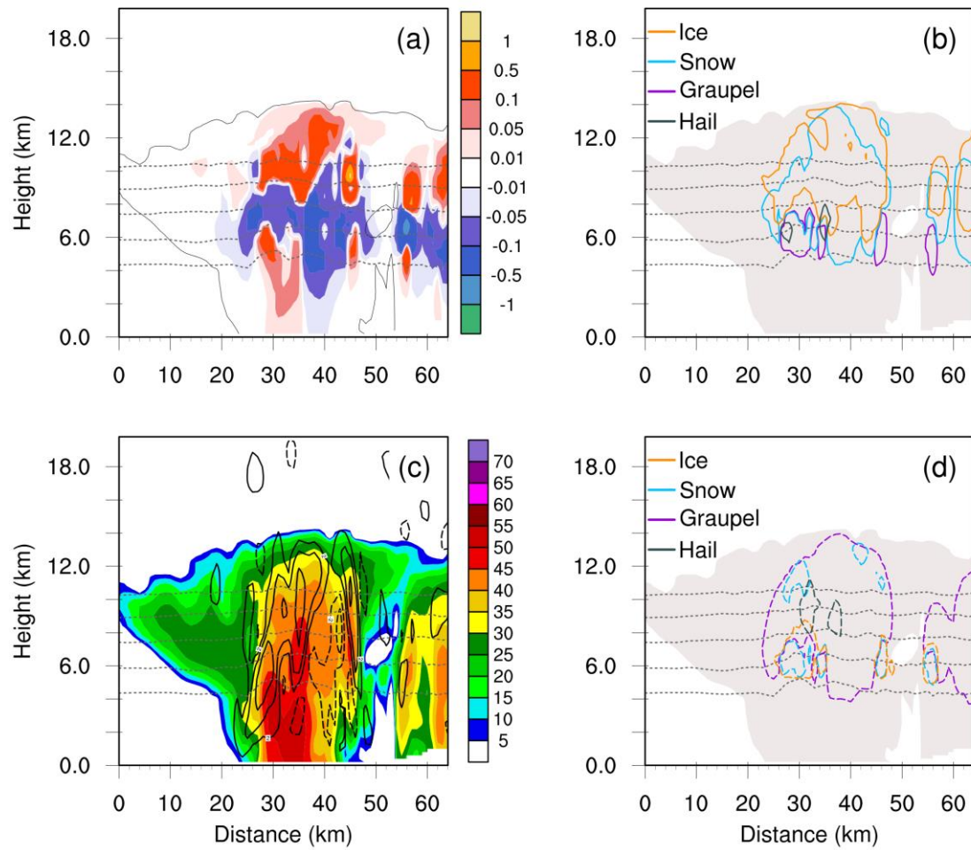
Figure 15 As in Fig. 14, but the vertical cross sections at the location shown in Fig. 4c of simulated variables at the mature stage of the thunderstorm (11:24 UTC) in the C-case.
