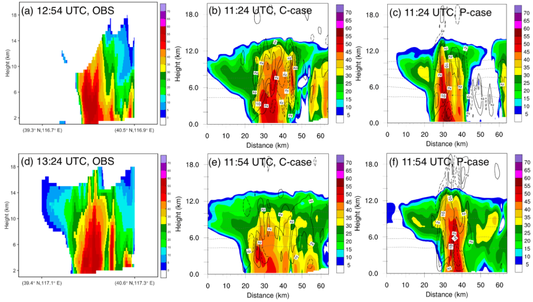
Figure 5 Comparison of vertical cross-section of radar reflectivity (unit: dBZ) along the black line shown in Fig. 4a-4f between observation and simulations. (a) Observation (black line shown in Fig.4a), (b) C-case (black line in Fig. 4c), (c) P-case (black line in Fig. 4e), (d) Observation (black line shown in Fig. 4b). (e) C-case (black line in Fig. 4d), and (f) P-case (black line in Fig. 4f).
