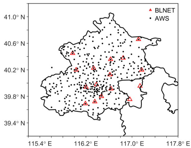
Figure 1 Spatial distributions of BLNET stations (red triangles), and ground-based automatic weather stations (black dots) in the Beijing region.
