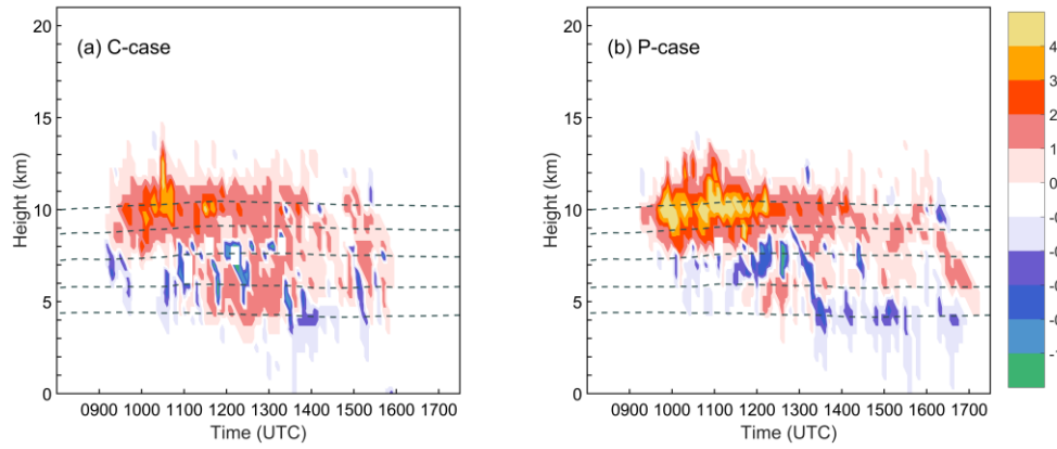
940 Figure 13 Temporal variation of the vertical profiles of peak positive (negative) charge density ( \text{nC m}^{-3} , shaded) of (a) C-case, and (b) P-case. The 0\text{ }^{\circ}\text{C} , -10\text{ }^{\circ}\text{C} , -20\text{ }^{\circ}\text{C} , -30\text{ }^{\circ}\text{C} and -40\text{ }^{\circ}\text{C} isotherms are shown by the dashed gray lines in (a)-(b).
