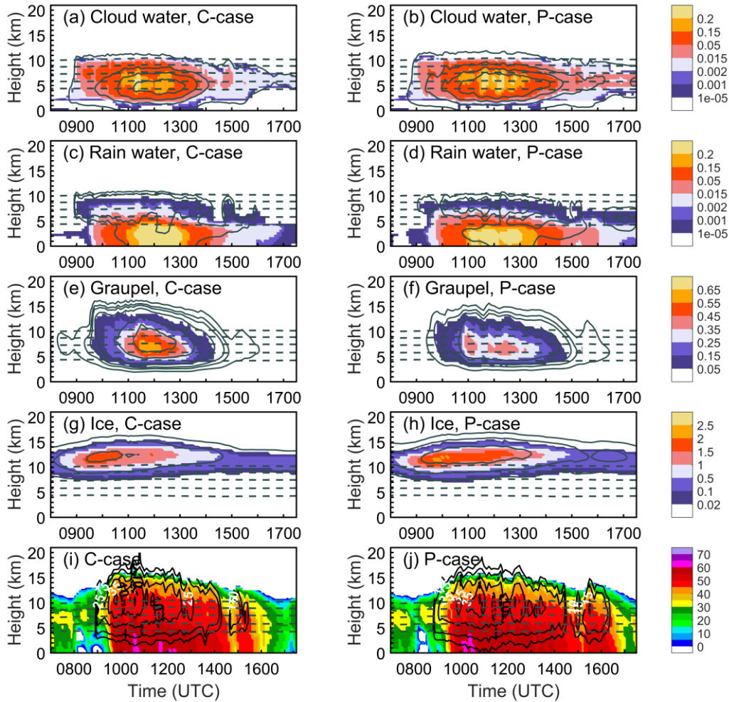
Figure 10 (a)-(h) Temporal variation of the vertical profiles of domain-averaged mass mixing ratio ( \text{g kg}^{-1} , shaded) and number concentration ( \text{kg}^{-1} , solid lines) of (a) cloud water in the C-case, (b) cloud water in P-case, (c) rain water in the C-case, (d) rain water in the P-case, (e) graupel in the C-case, (f) graupel in the P-case, (g) ice in the C-case, (h) ice in the P-case. Contour levels in (a)-(h) for cloud water number concentration are 10^6 , 2 \times 10^7 , 5 \times 10^7 , 10^8 \text{ kg}^{-1} , and for rain water are 100, 300 \text{kg}^{-1} , and for graupel are 10, 30, 50, 100, 300, 500, 700, 1000 \text{kg}^{-1} , and for ice are 0.1 \times 10^7 , 1 \times 10^7 , 5 \times 10^7 \text{ kg}^{-1} . (i)-(j) Time-height maximum simulated radar reflectivity (color shading, unit: dBZ) and maximum vertical velocities (solid line and white label: 10, 15, 25, 35, 45 \text{m s}^{-1} ; dashed line and black label: -10, -15 \text{m s}^{-1} ) for (i) the C-case and (j) the P-case. The 0 °C, -10 °C, -20 °C, -30 °C and -40 °C isotherms are shown by the dashed gray lines in (a)-(j).
