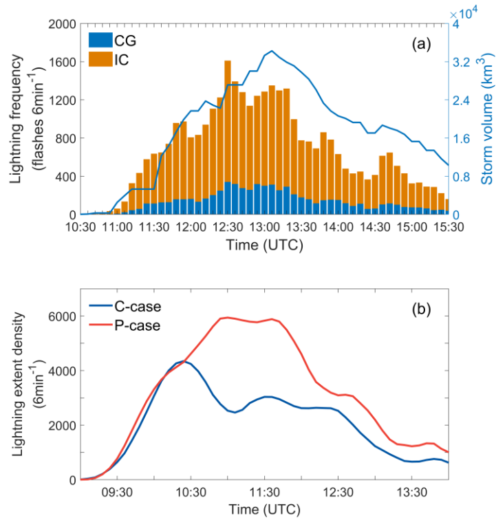
Figure 8 Temporal variation in (a) observed total lightning frequency and (b) simulated flash extent density (FED). In (a), orange represents IC lightning and blue represents CG lightning. The solid line represents the storm volume associated with radar reflectivity exceeding 30 dBZ. In (b), red line represents the P-case and blue line represents the C-case.
