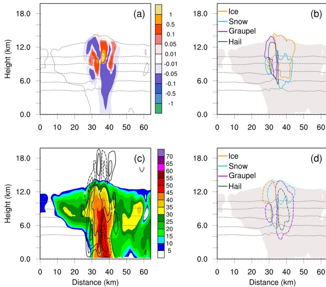
Figure 14 Vertical cross sections (south to north) at the location shown in Fig. 4f of simulated variables at the mature stage of the thunderstorm (11:54 UTC) in the P-case. (a) Total net space charge ( \text{nC m}^{-3} , shaded). The 0^\circ\text{C} , -10^\circ\text{C} , -20^\circ\text{C} , -30^\circ\text{C} and -40^\circ\text{C} isotherms are shown by dashed gray lines in (a)-(d). (b) +0.1 \text{ nC m}^{-3} space charge density contours for cloud ice (orange), snow (blue), graupel (purple), and hail (black). The cloud outline (reflectivity echoes \geq 5 \text{ dBZ} ) is denoted by the gray shaded contour. (c) Radar reflectivity (unit: \text{dBZ} ), black lines for vertical velocities (solid line: 2, 5, 10 \text{m s}^{-1} ; dashed line: -2 \text{ m s}^{-1} ). (d) As in (b), but for -0.1 \text{ nC m}^{-3} charge density.
