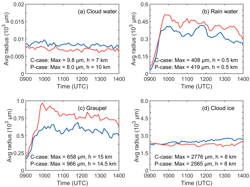
930 Figure 11 Temporal variation of domain-averaged effective radius for the different hydrometeors. (a) cloud water, (b) rainwater, (c) graupel, (d) ice. The red lines represent the P-case and the blue lines represent the C-case.
