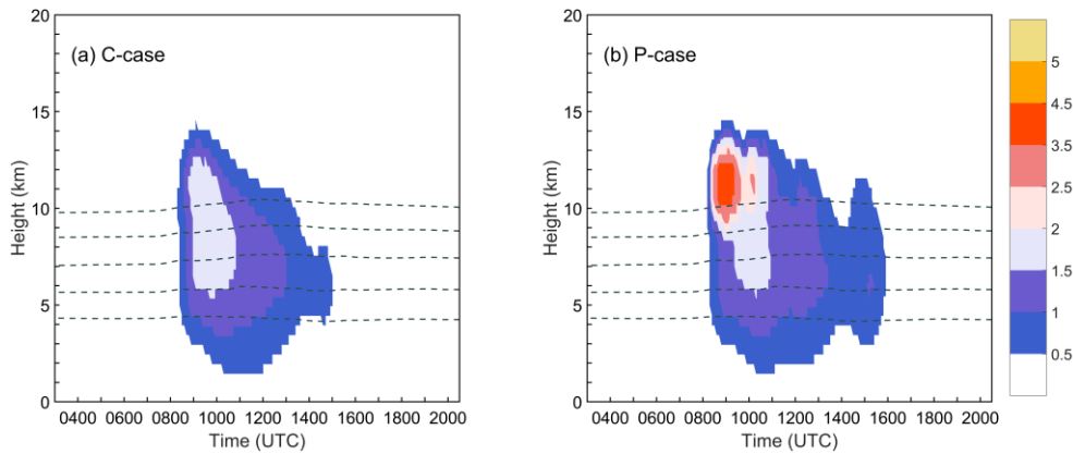
935 Figure 12 Temporal variation of the vertical profiles of peak latent heating ( \text{K h}^{-1} , shaded) of (a) C-case, and (b) P-case. The 0\text{ }^{\circ}\text{C} , -10\text{ }^{\circ}\text{C} , -20\text{ }^{\circ}\text{C} , -30\text{ }^{\circ}\text{C} and -40\text{ }^{\circ}\text{C} isotherms are shown by the dashed gray lines in (a)-(b).
