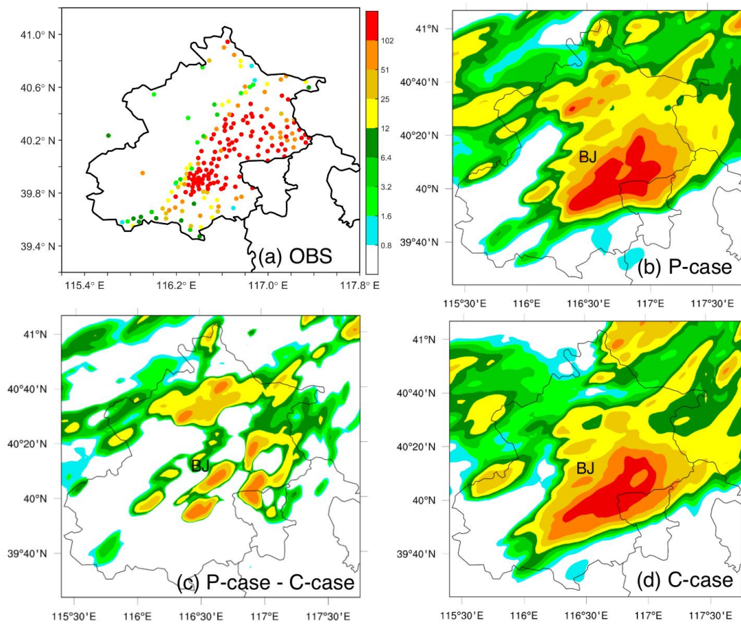
Figure 7 Comparison of accumulated precipitation (units: mm) between observation (11:00-17:00 UTC) and simulations (10:00-16:00 UTC). (a) Observation. (b) P-case, and (d) C-case. And (c) difference of accumulated precipitation (units: mm) between the P- and C-cases.
