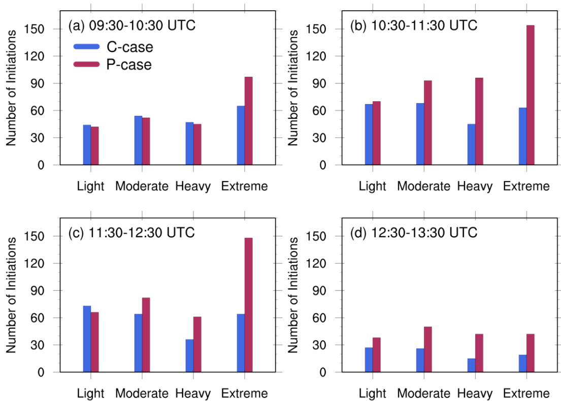
Figure 9 Number of initiations for different lightning intensity categories in different time, i.e. light (50-100 grid points), moderate (100-200 grid points), heavy (200-300 grid points) and extreme (>300 grid points), simulated for the P- and C-cases.
