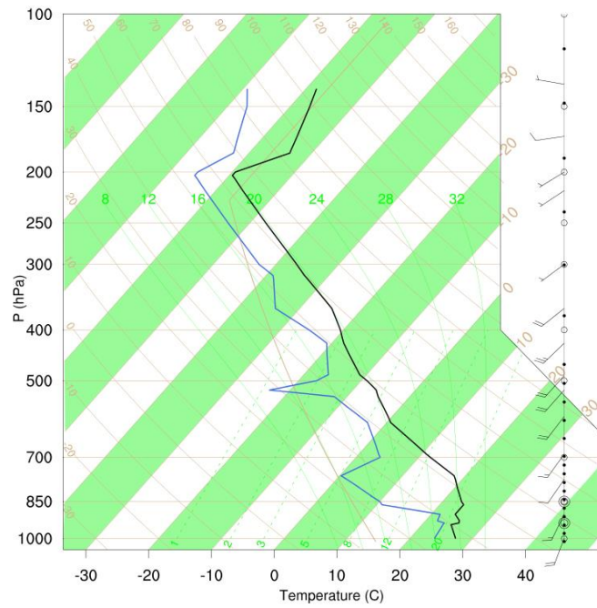
Figure 2 Sounding profiles for Beijing at 00:00 UTC on 11 August 2017. The black and blue solid lines represent temperature and dew point, respectively.
