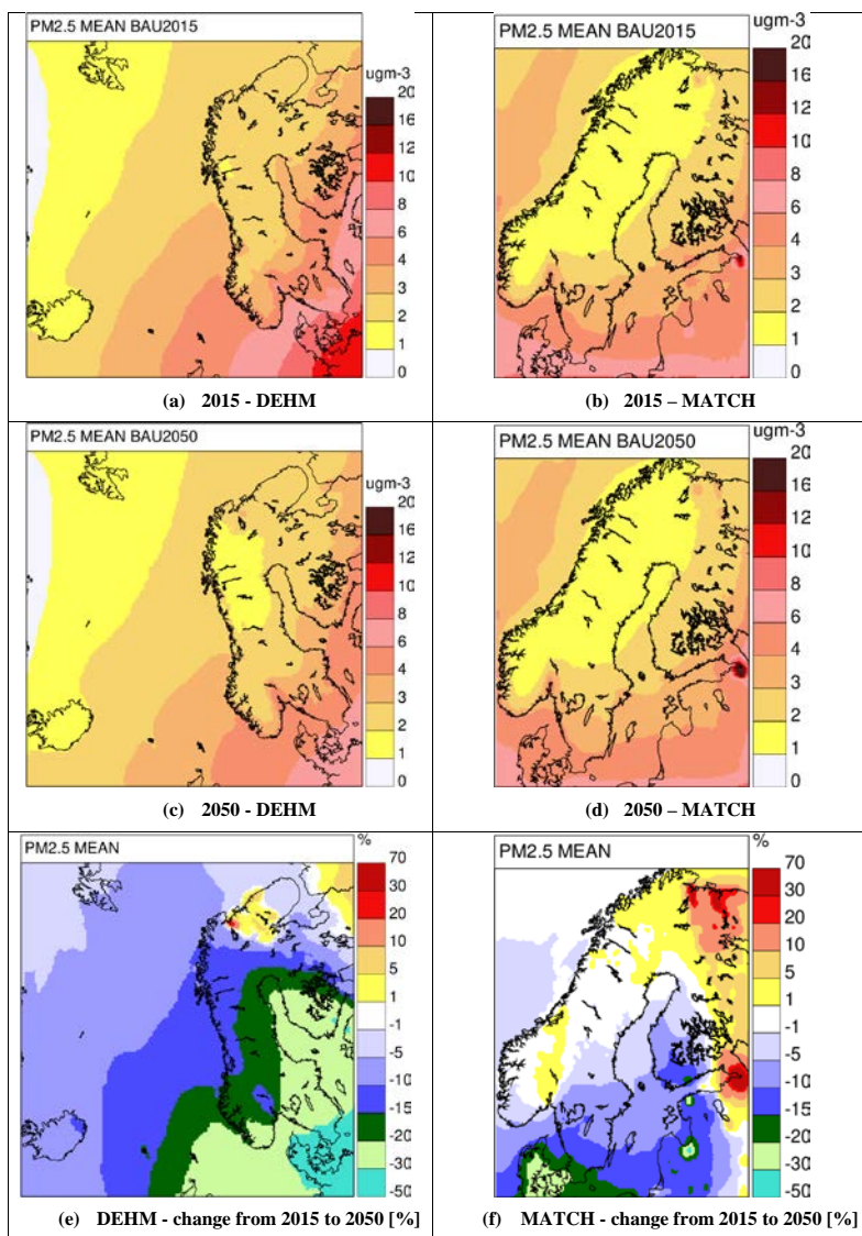
400 Figure 46: The annual mean surface PM 2.5 concentration [ \mu\text{g}/\text{m}^3 ] for 2015, 2050 and the % change as simulated by the two models.
