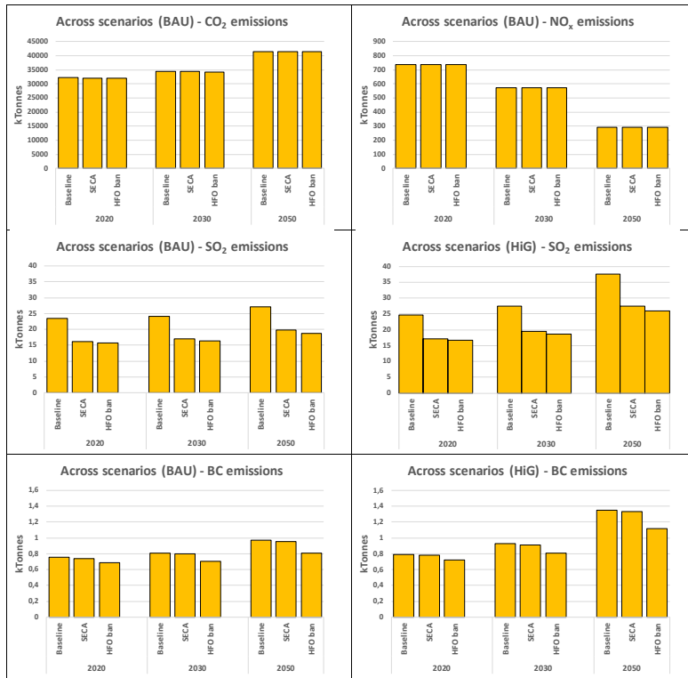
340 Figure 34: Emissions for domain d03 calculated in the Baseline, SECA and HFO ban BAU scenarios (CO 2 , NO x , SO 2 and BC) and the HiG scenarios (SO 2 and BC).
