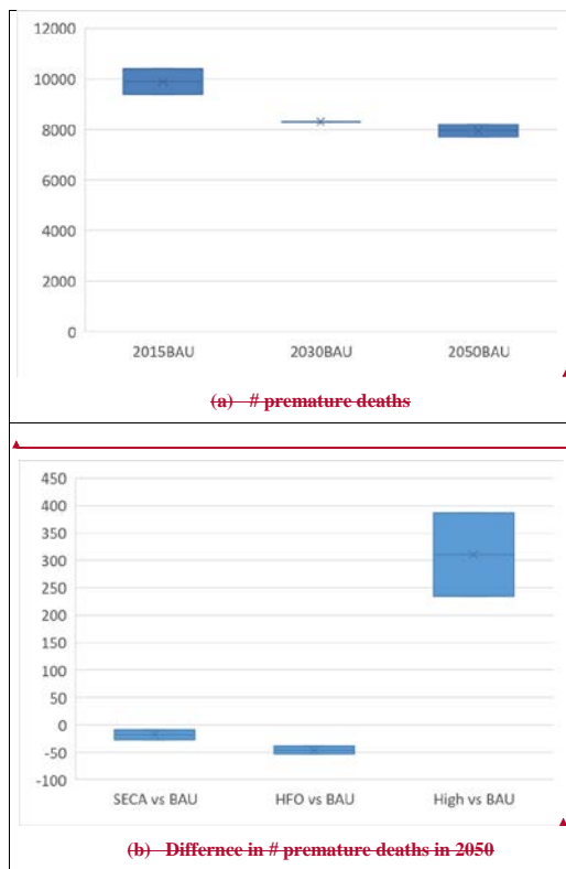
490 Figure 10: (a) The estimated total number of premature deaths due to air pollution (sum for the largest four Nordic countries) for 2015 and the projected numbers for 2030 (based on DEHM-EVA alone) and 2050. (b) The difference in the number of premature deaths between the ship emission scenarios for 2050.
