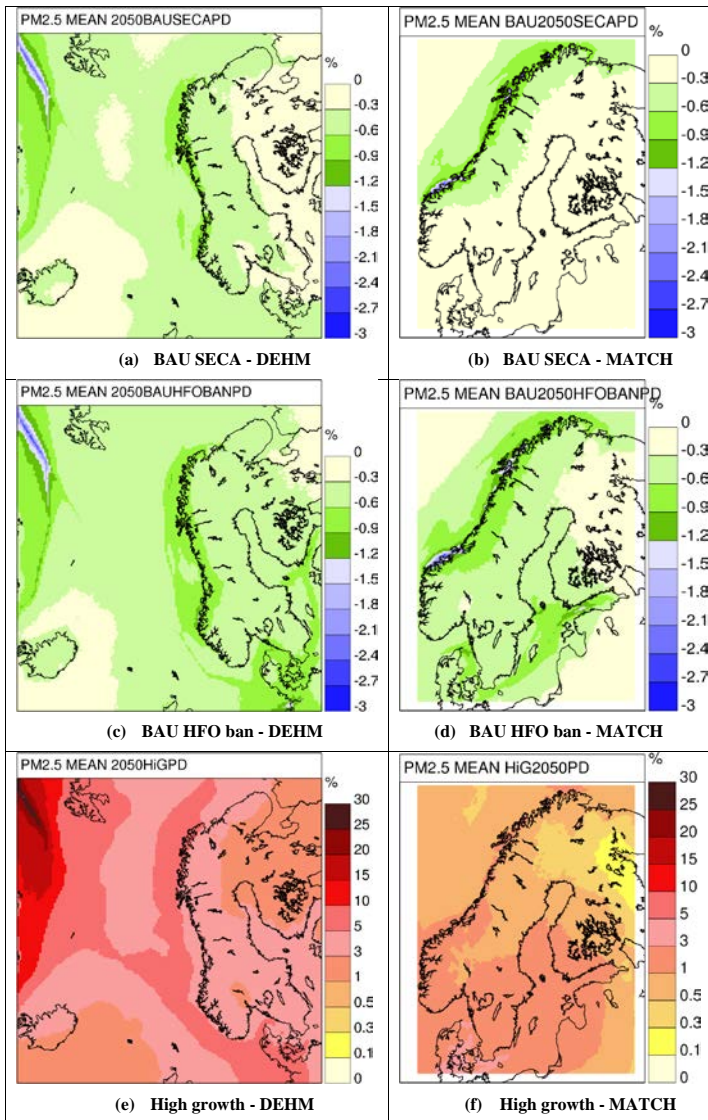
Figure 79: The % difference between the BAU baseline 2050 simulation and the three different ship emission scenarios (including the polar diversion route). As simulated by the two models DEHM (left) and MATCH (right). Calculated as e.g. (2050BAU\_SECA - 2050BAU)/2050BAU * 100\% .
