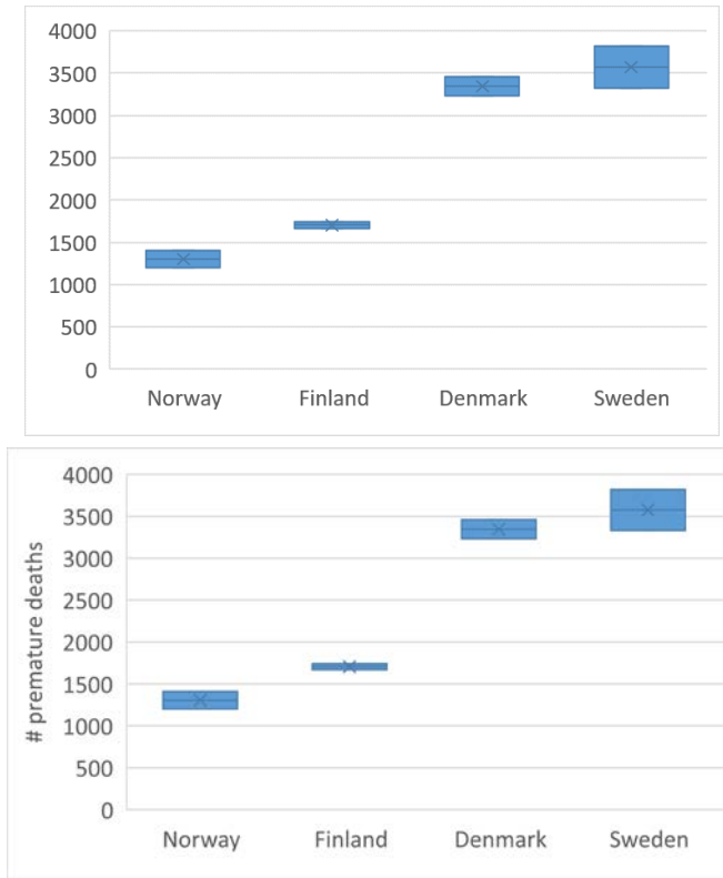
Figure 57: Premature deaths attributable to NO 2 , O 3 , SO 2 and PM 2.5 exposure in the four largest Nordic countries in the base case for 2015 (including all main anthropogenic emission sources). The results are given as box plots, where the 'x' indicates the central estimate and the size of the box show the difference between the DEHM-EVA and MATCH-EVA assessments.
