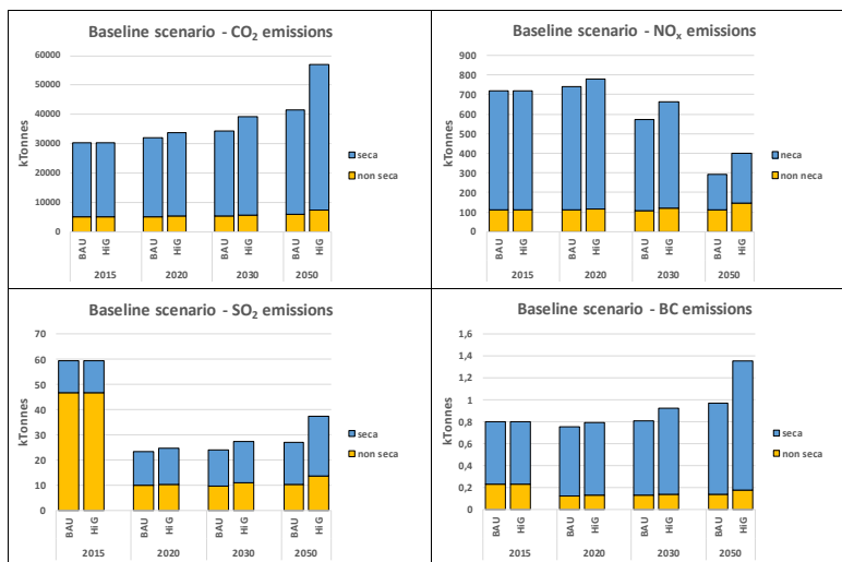
325 Figure 23: CO 2 , NO x , SO 2 and BC emissions for 2015 and Baseline scenario results for 2020, 2030 and 2050, split into SECA and non SECA parts of domain d03.
