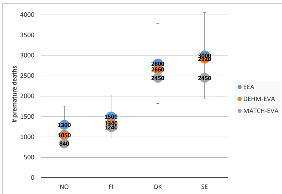
Figure 68: Comparison between the assessment of premature deaths reported by EEA for 2015 and the current assessment (base case 2015) for effects related to PM 2.5 exposure. The EEA number includes an error bar displaying the assumed uncertainty (±35%).
