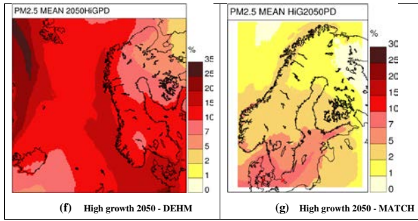
Figure 814: The contribution from shipping to the PM 2.5 annual levels as simulated by the two models for the present day and three different shipping emission scenarios for 2050. (Calculated as e.g. (2015BAU - 2015BAU_{70\%/0.3}) / 2015BAU * 100\% , where 2015BAU_70 is a run where the shipping emissions have been reduced to 70%).
