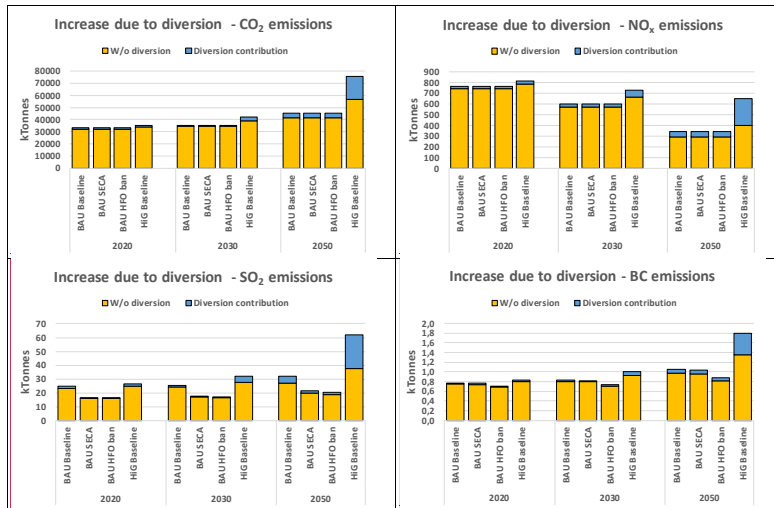
Figure 5: Estimated emissions of CO 2 , SO 2 , NO x and BC in domain d03 without polar diversion traffic and for polar diversion traffic for the scenarios in 2020, 2030 and 2050.
