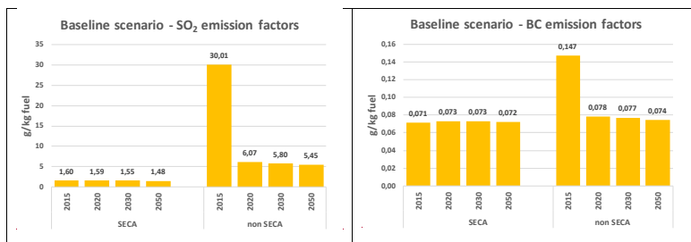
315 Figure 2: Fuel related emission factors of CO 2 , NO x , SO 2 and BC for 2015, 2020, 2030 and 2050 split into SECA and non SECA.
