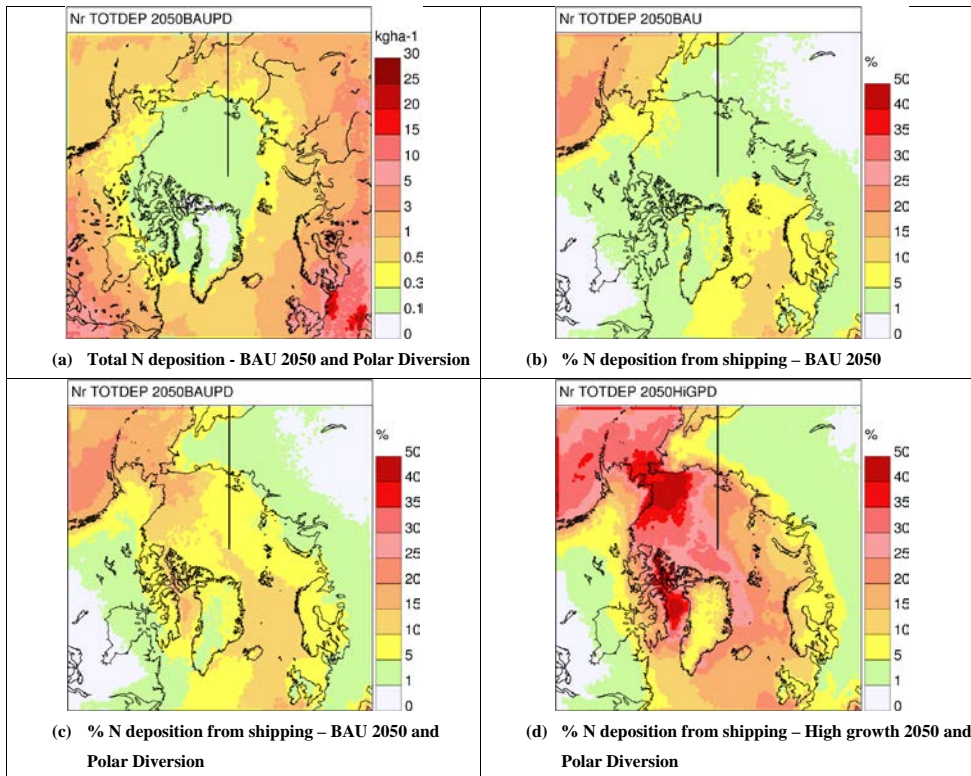
Figure 114: (a) The total Nitrogen deposition across the Arctic and Nordic region in the BAU 2050 Polar diversion scenario in the DEHM d02 domain. (b) and (c) displays the contribution from shipping without and with the polar diversion, while (d) displays the contribution in the High growth traffic scenario (including the polar diversion).
