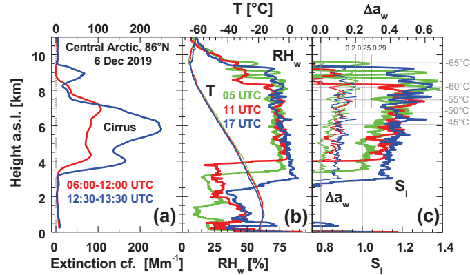
Figure 15. (a) Temporally averaged (mean) cirrus extinction coefficient \sigma (532 nm) for two observational periods from 6-12 UTC (red) and from 12:30-13:30 UTC (blue, see Fig. 3c), (b) profiles of temperature T and relative humidity RH_w (over water) observed with radiosondes launched at 5, 11, and 17 UTC on 6 December 2019, and (c) water activation criterium \Delta a_w and ice supersaturation S_i computed from the temperature and water vapour observations shown in (b). The water activation criterium \Delta a_w is the difference between the observed RH_w (in decimal numbers) and the ice-saturation-related RH_w value (for the observed temperature). In (c), different temperature levels are indicated by thin horizontal lines and \Delta a_w values of 0.2, 0.25, and 0.29, required to initiate ice nucleation, are shown as vertical line segments.
