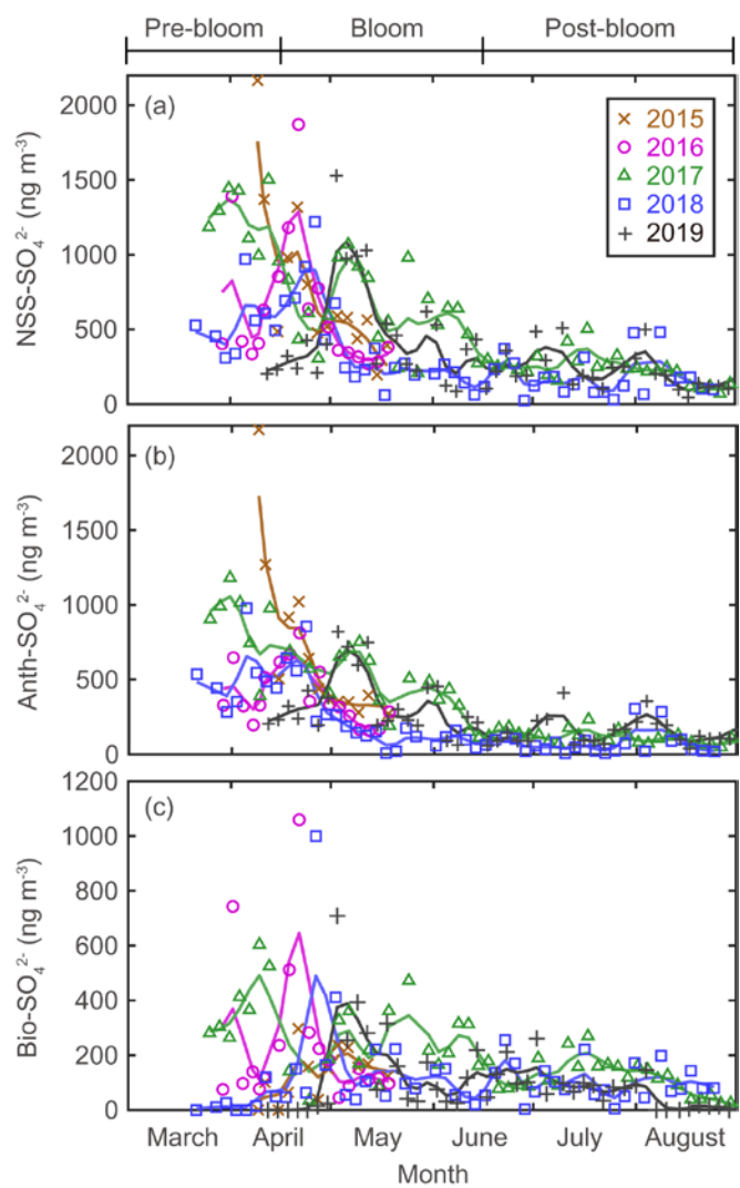
Figure 4: Aerosol concentrations for: (a) NSS-SO 4 2- (total SO 4 2- minus ss-SO 4 2- ); (b) Anth-SO 4 2- , and (c) Bio-SO 4 2- . The colored solid lines indicate 15-day moving average values.
