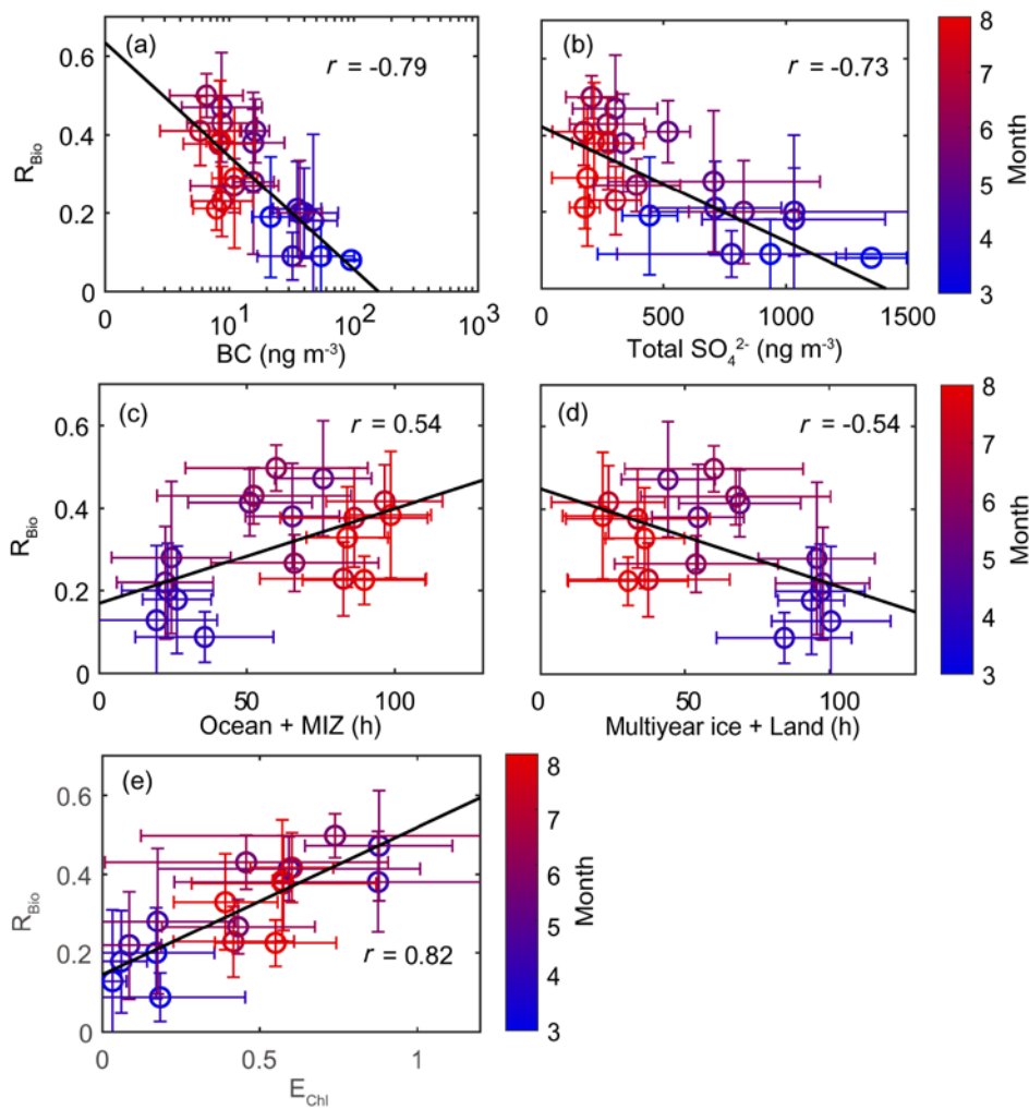
Figure 9: Scatter plot of (a) monthly mean black carbon (BC) concentration versus monthly mean R_{Bio} and (b) monthly mean Total SO_4^{2-} concentration versus monthly mean R_{Bio} . Error bars and black solid line represent 1\sigma and the best fit, respectively.
