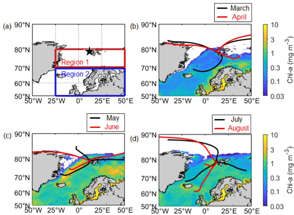
790 Figure 1: (a) Location of the aerosol sampling site (black pentagram; Gruevbadet observatory; 78.9° N, 11.9° E) and the ocean domains (70° N–80° N, 25° W–50° E for Region 1; 50° N–70° N, 25° W–50° E for Region 2) defined for this study. Mean Chl- a concentration for (b) March and April, (c) May and June, and (d) July and August over the period of 2015–2019, overlaid with air mass trajectory clusters that represent the dominant pathways of air masses reaching to the observation site.
