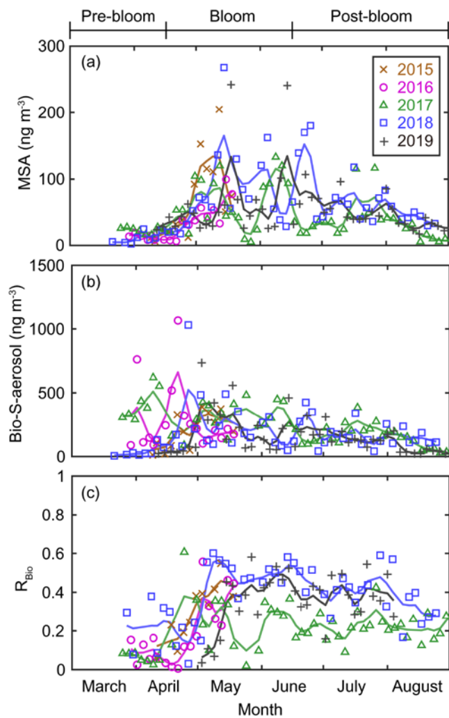
Figure 5: Aerosol concentrations of (a) MSA and (b) Bio-aerosol ( \text{MSA} + \text{Bio-SO}_4^{2-} ). (c) Variations in the ratio of MSA to Bio-aerosol ( R_{\text{Bio}} ). The colored solid lines indicate 15-day moving mean values.
