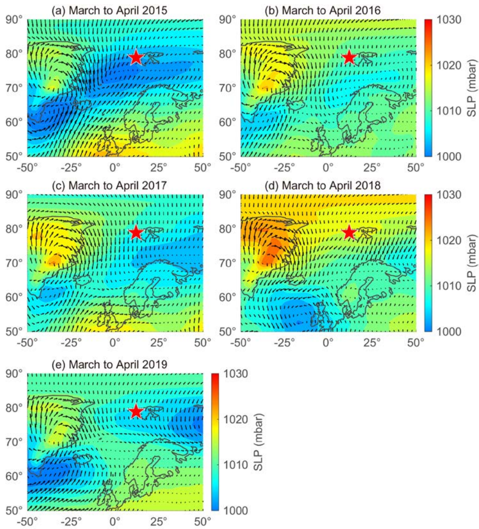
Figure 6: Sea level pressure (SLP) overlaid with wind vectors during March to April in (a) 2015, (b) 2016, (c) 2017, (d) 2018, and (e) 2019. Red stars indicate the location of the sampling site (Gruevbadet observatory; 78.9° N, 11.9° E).
