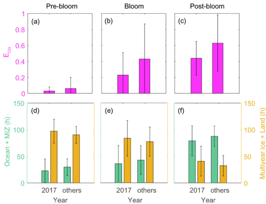
810 Figure 11: Air mass exposure to chlorophyll ( E_{Ch} ) (a–c) and the air mass residence times over the ocean and marginal ice zone (MIZ) and the multi-year ice and land areas (d–f) during pre-bloom, bloom, post-bloom periods. Error bars represent 1\sigma .
