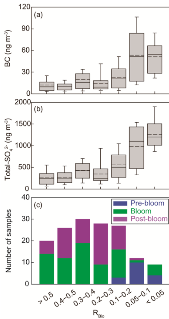
Figure 8: Plots of the seasonal (a) black carbon (BC) concentration versus R_{Bio} , (b) the total SO_4^{2-} concentration versus R_{Bio} , and (c) the number of samples included in each R_{Bio} group. The solid and dotted lines represent the median and mean values of the data in the box plots, respectively.
