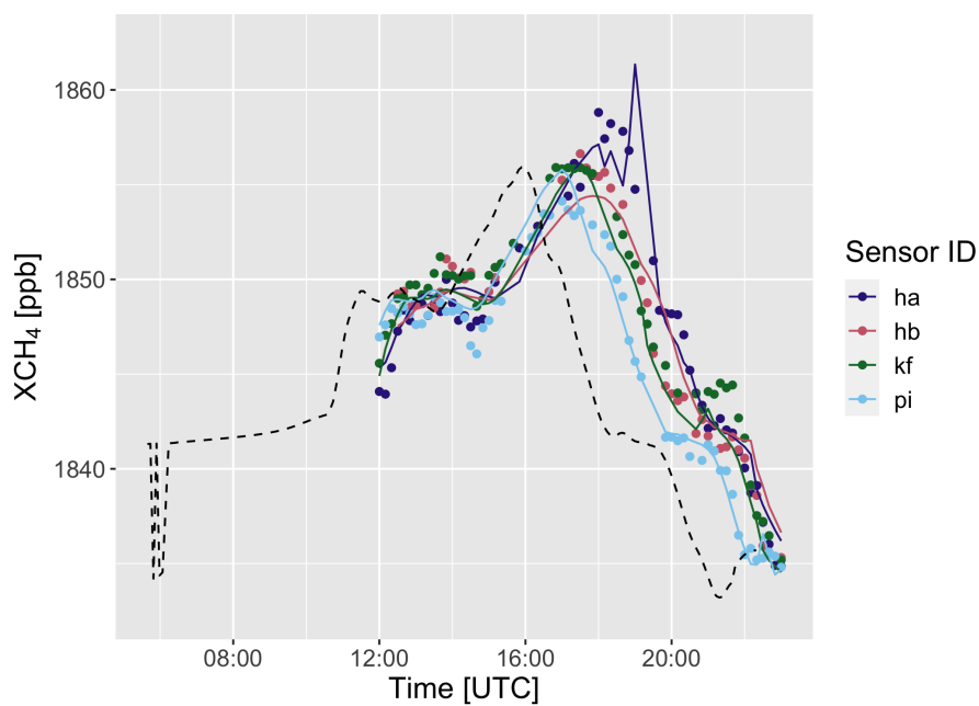
Figure 11. Observed XCH 4 values for May 13 (shown in points). Optimized background values (gray, dashed) and optimized total column values, including urban emissions (colored lines) also shown.
