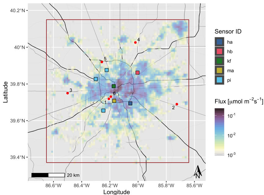
Figure 1. Prior estimate of emissions due to natural gas infrastructure. EM27/SUN deployment locations are shown with squares. Locations of known point sources are also shown (red circles, summarized in Table 1). Map tiles by Stamen Design, under CC BY 3.0. Data by OpenStreetMap, © OpenStreetMap contributors 2020. Distributed under a Creative Commons BY-SA License.
