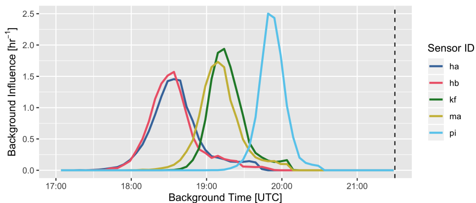
Figure 5. Fraction of background influence for all sites on May 13 at 21:30 UTC. These are residence time PDFs, and therefore the integrals over the graphs are equal to 1.
