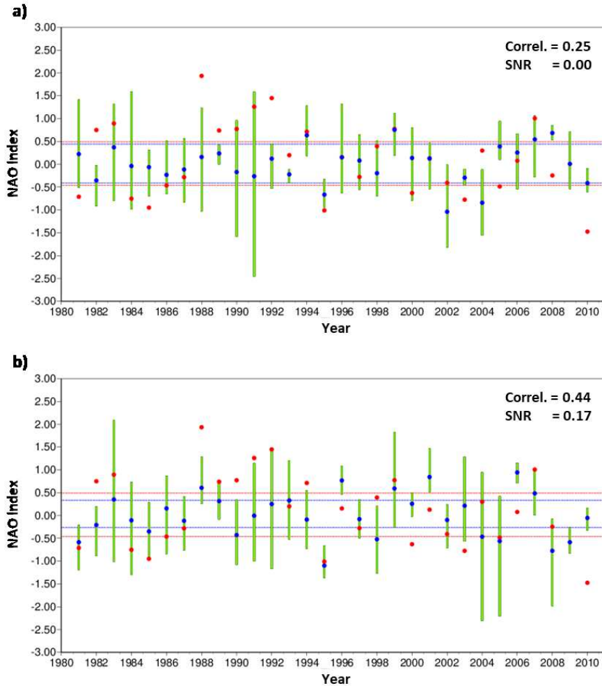
Figure 16. Time series of the winter (DJF) NAO index for the long-range experiment using (a) the default configuration (top) and the one, and (b) the experiment using the new BMS ozone (bottom). This plot shows the correlation between the model experiments and, together with NAO index values from the ERA-Interim reanalysis. Red dots represent the NAO index value from ERA-Interim reanalysis, while blue dots correspond to the ensemble mean of the corresponding model runs; the green bars show the ensemble variability for each year NAO index. The NAO index is calculated as the first empirical orthogonal function (EOF) of the geopotential height Z500 over the North Atlantic sector. The correlation value between the ensemble mean NAO index and the reanalysis NAO index time series is also included in each panel, together with the signal to noise ratio (SNR) value for each case. The horizontal lines delimit the main tercile interval for the ensemble mean time series of the model experiments (blue) and ERA-Interim (red).
