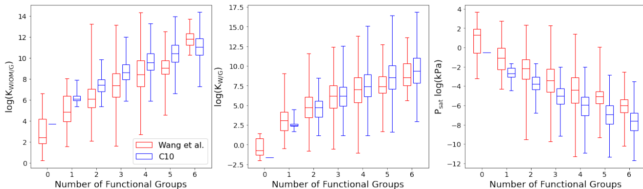
Figure 8. Box plot comparing C10 (in blue) with Wang’s dataset (in red) for K_{\text{WIOM/G}} , K_{\text{W/G}} and P_{\text{sat}} for different numbers of functional groups. Shown are the minimum, maximum, median, first and third quartile.
