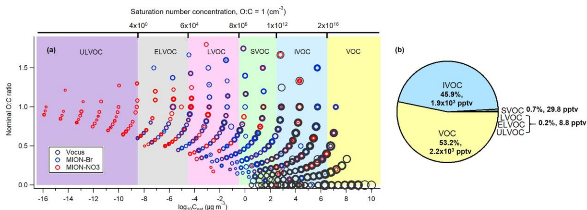
Figure 7. (a) Combined 2-dimensional volatility distribution for all measured organic compounds (with the approach described in section 2.2.1) parameterized with the modified Li et al. (2016) approach (Daumit et al., 2013; Isaacman-VanWertz and Aumont, 2020). Markers were sized by the logarithm of their corresponding concentrations, and marker color represents that either the compound was only measured by that instrument or the maximum concentration of the compound observed in common was detected by that instrument; (b) resulting pie chart for the contributions of VOC, IVOC, SVOC, LVOC, ELVOC, and ULVOC.
