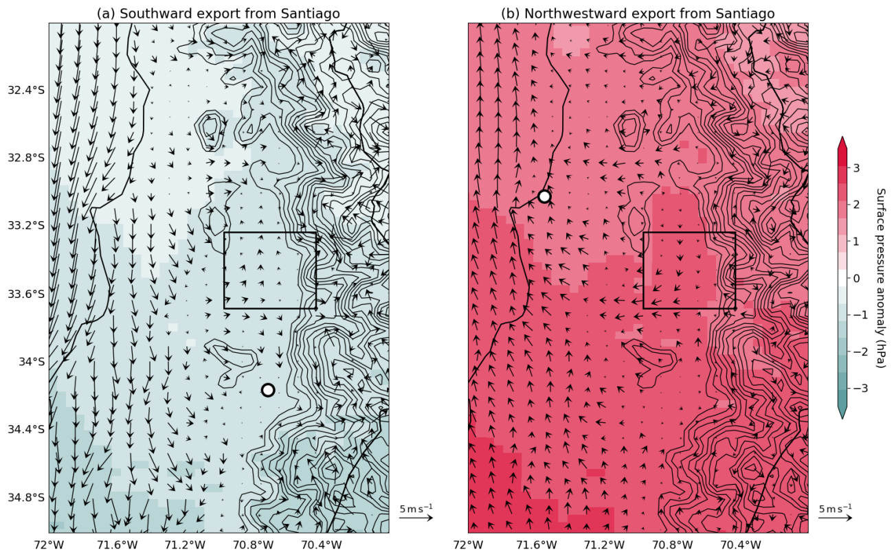
Figure A4. (a) Composite of surface wind (arrows) and pressure (colormap) anomalies with respect to the wintertime average, for hours of southward transport episodes, defined as hours when the concentration of \text{PM}_{2.5} from Santiago (black rectangle) in Rancagua (white dot) is greater or equal to its 90 th percentile for the period. Contours show terrain elevation in excess of 1000 m every 250 m. (b) same as (a) but during hours of northwestward transport, defined in the same manner but with respect to concentrations in Viña del Mar (white dot).
