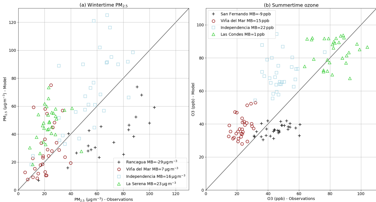
Figure 2. Comparison between observation and simulation for (a) wintertime daily average PM_{2.5} concentrations, (b) summertime daily maximum O_3 mixing ratio. Wintertime and summertime correspond to the periods defined in Section 2.1, respectively. MB is the mean bias.
