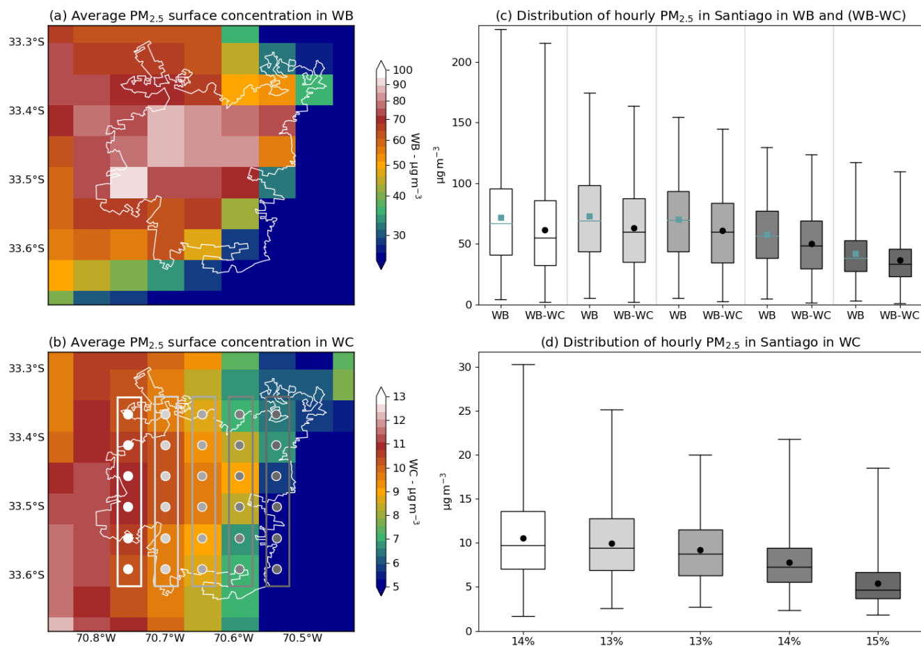
Figure 6. (a) Average ground-level PM_{2.5} concentration in scenario WB. White contour shows the limits-boundaries of the Santiago Metropolitan-Areacity . (b) same as (a) for scenario WC, (c) Distribution of hourly PM_{2.5} surface concentration in WB and (WB-WC). Boxes show the average, median, minimum, maximum, first and third quartiles. Shades of gray correspond to the zones defined in (b) on which an average is made, (d) same as (c) for scenario WC. Percentages indicate the relative average contribution of transport.
