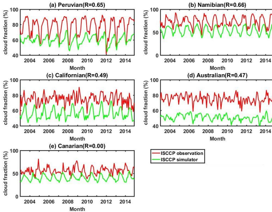
Figure R9: Monthly mean time series of cloud fraction from ISCCP simulator outputs MEM (green lines) during 2003-2014 compared with satellite observations (ISCCP, red lines), over the (a) Peruvian, (b) Namibian (c) Californian, (d) Australian and (e) Canarian regions. The R indicate the temporal correlations between satellite observations and ISCCP simulator outputs.
