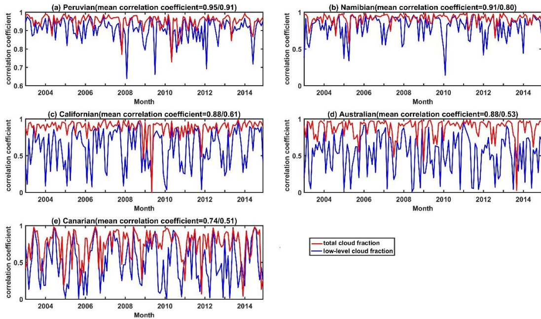
Figure R10: Monthly mean time series of correlation coefficients between total cloud fraction (red lines) and low-level cloud fraction (blue lines) and planetary albedo from CERES observations during 2003-2014, over the (a) Peruvian, (b) Namibian (c) Californian, (d) Australian and (e) Canarian regions. The monthly mean correlation coefficients are given in the title. The left side of the slash ('/') is the monthly mean correlation coefficients of the total cloud fraction, and the right side of the slash ('/') is that of low-level cloud fraction.
