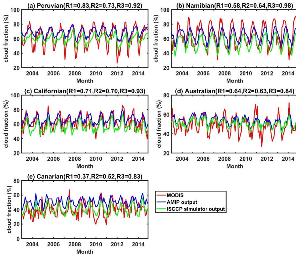
Figure R8: Monthly mean time series of cloud fraction from AMIP6 MEM outputs and ISCCP simulator outputs MEM during 2003-2014 compared with satellite observations (MODIS), over the (a) Peruvian, (b) Namibian (c) Californian, (d) Australian and (e) Canarian regions. The R1 and R2 indicate the temporal correlations between satellite observations and AMIP6 outputs and ISCCP simulator outputs, respectively. The R3 indicates the temporal correlations between AMIP6 outputs and ISCCP simulator outputs. Here, the ISCCP MEM is calculated based on 11 model outputs (see the Table R1 below).
