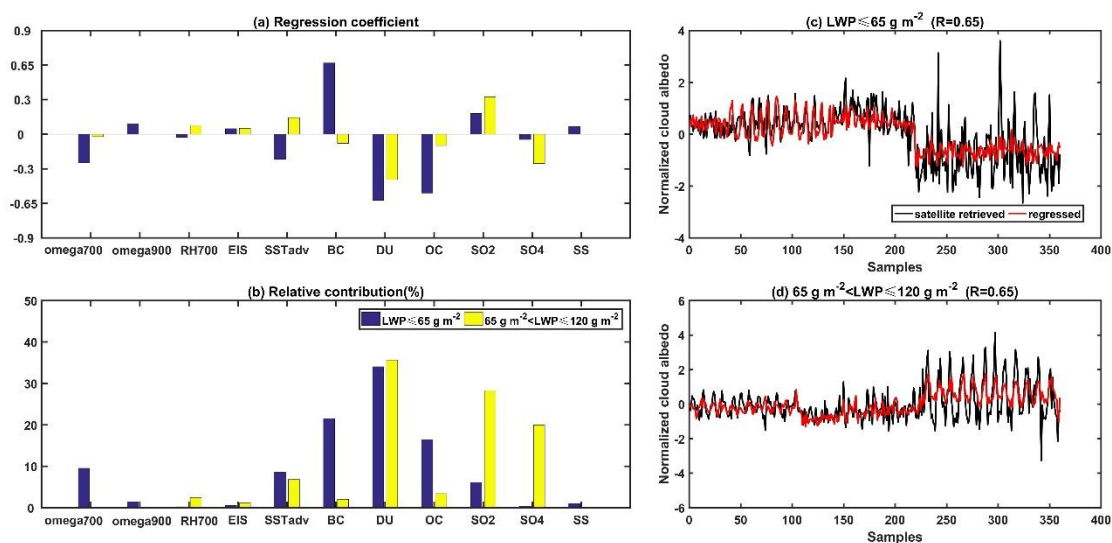
Figure R14 (Fig. 6 in the revised manuscript): Similar to Figure R13, but for MODIS LWP (LWP threshold: 65 \text{ g m}^{-2} ).
