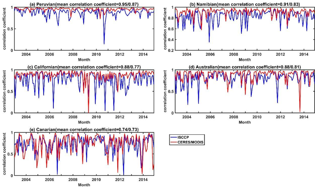
Figure R11: Monthly mean time series of correlation coefficients between cloud fraction and planetary albedo from CERES/MODIS observations (red lines) and ISCCP observations (blue lines) during 2003-2014, over the (a) Peruvian, (b) Namibian (c) Californian, (d) Australian and (e) Canarian regions. The monthly mean correlation coefficients are given in the title. The left side of the slash (‘/’) is the monthly mean correlation coefficients of CERES/MODIS observation, and the left side of the slash (‘/’) is that of ISCCP.
