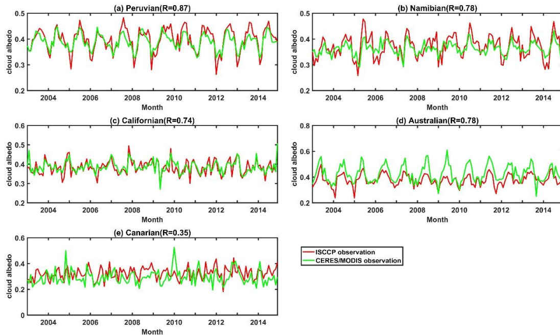
Figure R12: Monthly mean time series of cloud albedo based on ISCCP observation (red lines) during 2003-2014 compared with that of CERES/MODIS observations (green lines), over the
