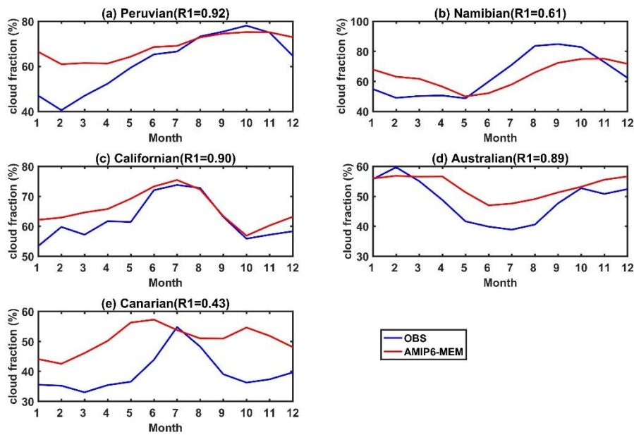
Figure R6: Seasonal cycles of cloud fraction from AMIP6 MEM outputs (red line) and during 2003-2014 compared with satellite observations (blue line), over the (a) Peruvian, (b) Namibian (c) Californian, (d) Australian and (e) Canarian regions. The R1 indicate the temporal correlations between satellite observations and AMIP6-MEM.
