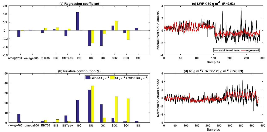
Figure R16: Similar to Figure R14, but the threshold of 60 \text{ g m}^{-2} for LWP is used.
