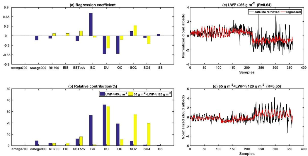
Figure R15: Similar to Figure R14, but for ERA5.
