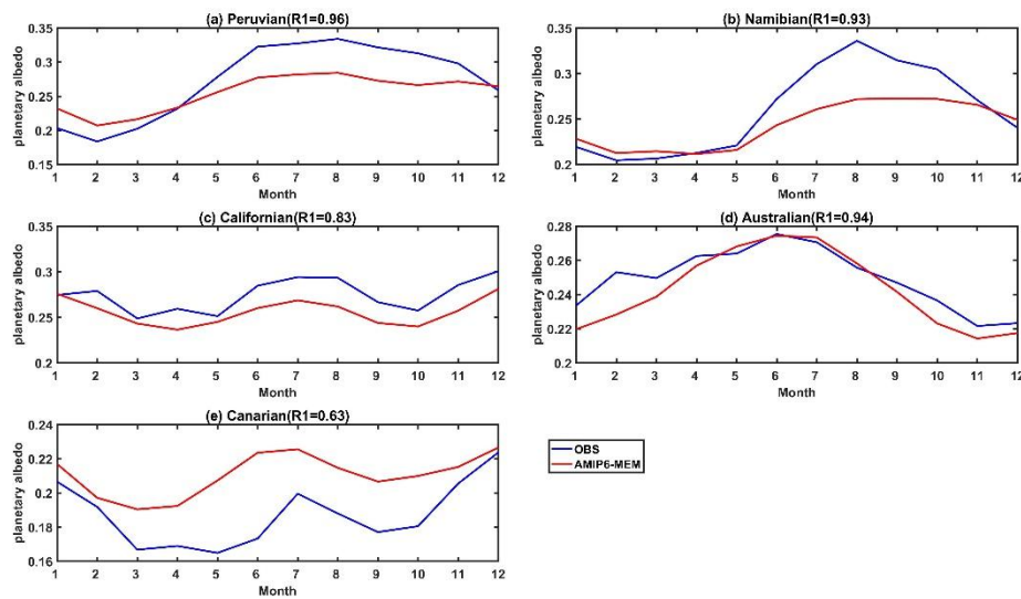
Figure R7: Similar to Figure R6, but for planetary albedo.
