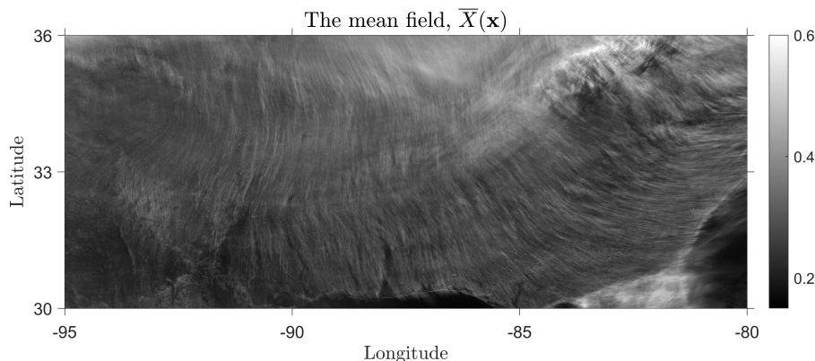
Figure 2. The time-averaged corrected reflectance field \bar{X}(\mathbf{x}) . Note the clear stripes in \bar{X}(\mathbf{x}) , marking the cloud streets along the mean CBL wind direction.
