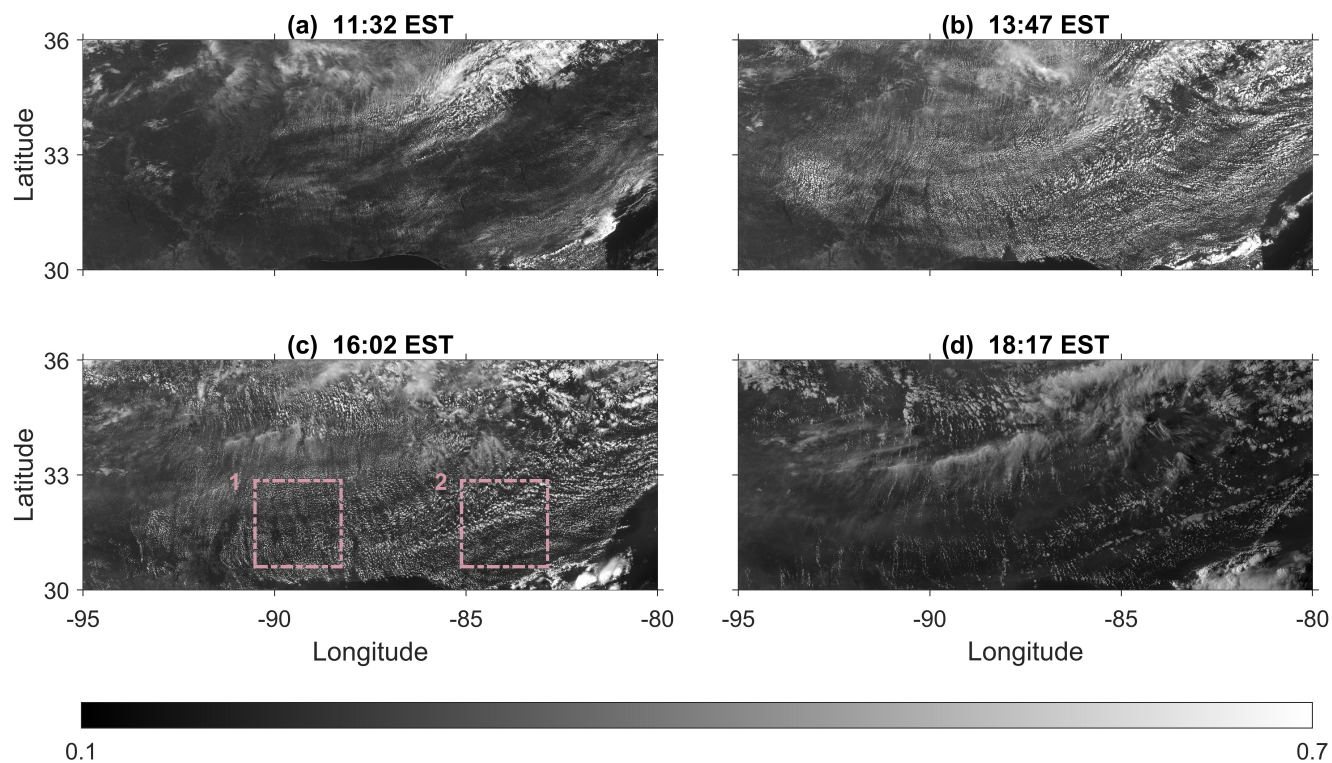
Figure 1. Corrected reflectance field of the diurnal cloud evolution as obtained from GOES–16 ABI’s “Red” visible band (channel 2; 0.64\ \mu\text{m} ). Snapshots taken at 11:32 (a), 13:47 (b), 16:02 (c), and 18:17 (d) EST. Dashed boxes in (c) represent two subdomains analysed in Fig. 3.
