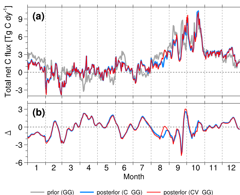
Figure 10: Time series of posterior total net carbon fluxes (a) and their differences from prior ( \Delta ) (b) for 2015. Posterior fluxes of C_{GG} (blue) and CV_{GG} (red) and their prior flux (grey) are presented.
