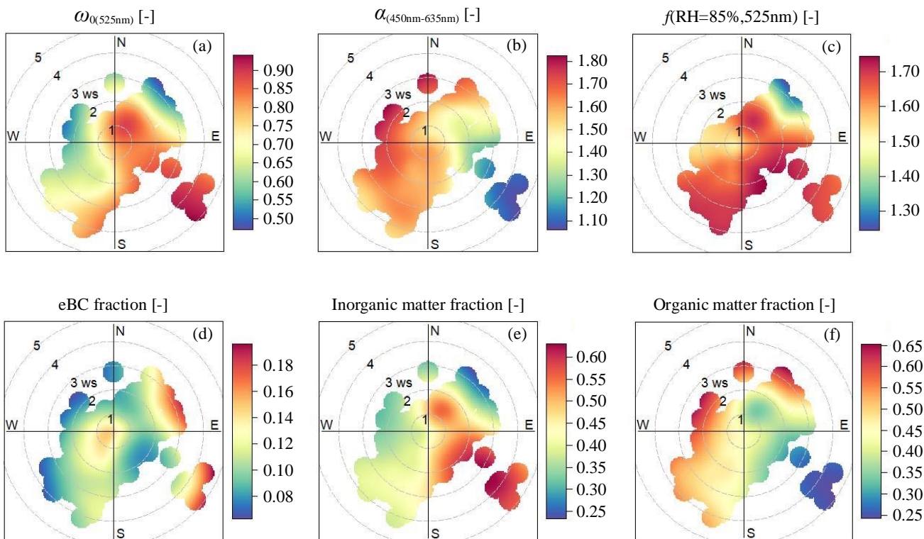
Figure 2: Wind dependence of (a) the single-scattering albedo ( \omega_{0(525nm)} ), (b) the scattering Ångström exponent ( \alpha_{(450nm-635nm)} ), (c) the particle light scattering enhancement factor at RH = 85% ( f(RH = 85\%, 525nm) ), (d) the mass fraction of eBC, (e) the mass fraction of inorganic matter, and (f) the mass fraction of organic matter. The circular contours show the average change in wind speed and direction.
