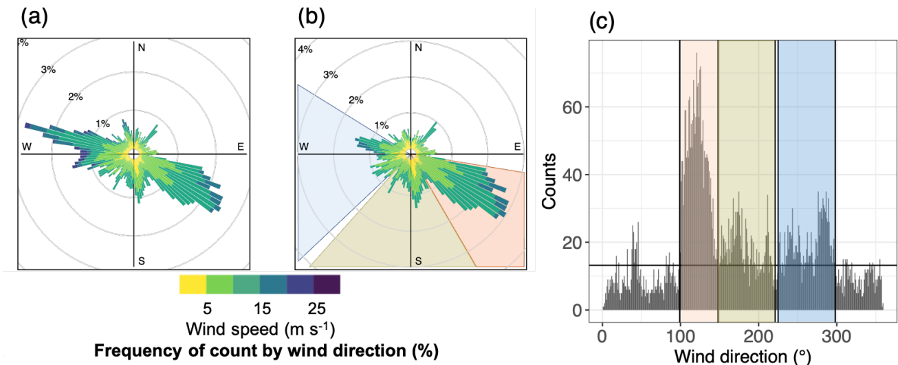
265 Figure 2 (a): Wind rose for the entire analysed PCAN voyage (February 6-March 4, 2017). (b): Wind rose for wind measurements south of 56.5° S (excluding measurements from the homeward transit to Hobart Tasmania, the Transit category), showing selected sectors. There are three areas demonstrating a higher density of wind measurements, from the WNW (Ferrel, sector: 225-298°, width 73°), from the SE (Polar, sector 99-148°, width 49°) and from the S (Southerly, 148-217°, width 69°). These sectors, capturing 76% of available wind measurements, are shaded in blue (Ferrel, 22%), grey (Southerly, 20%) and orange (Polar, 34%) respectively. (c): Frequency histogram of wind measurements plotted in 2b with 1° bin size. Ferrel (blue), Southerly (grey) and Polar (orange) sectors are highlighted.
