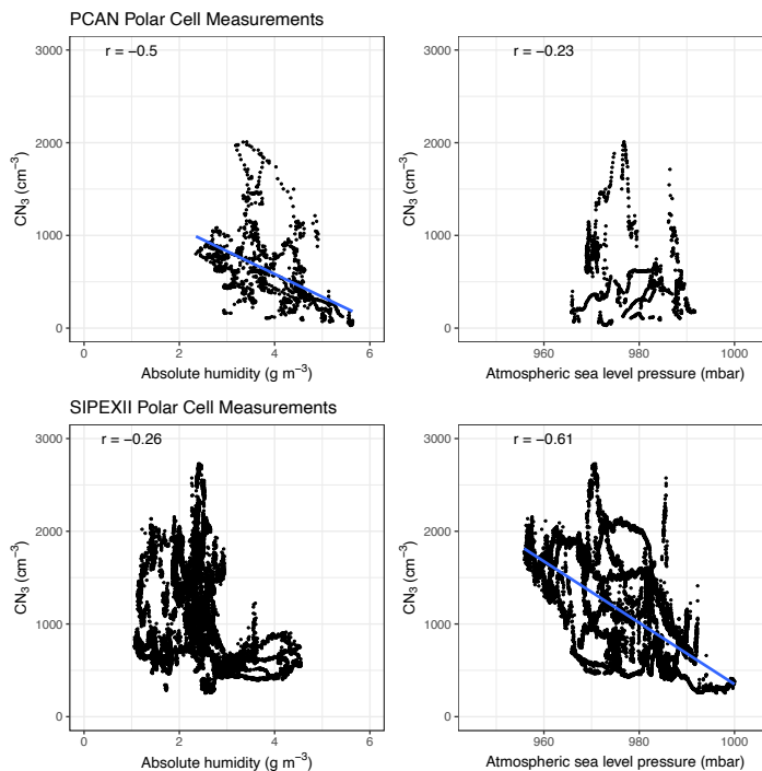
605 Figure 6: Comparison of PCAN (top row) and SIPEXII (bottom row) AH and atmospheric sea level pressure measurements plotted against CN_3 measurements in the Polar cell. Linear regression lines are plotted on the stronger relationship for each voyage. Pearson's r values are plotted on each facet.
