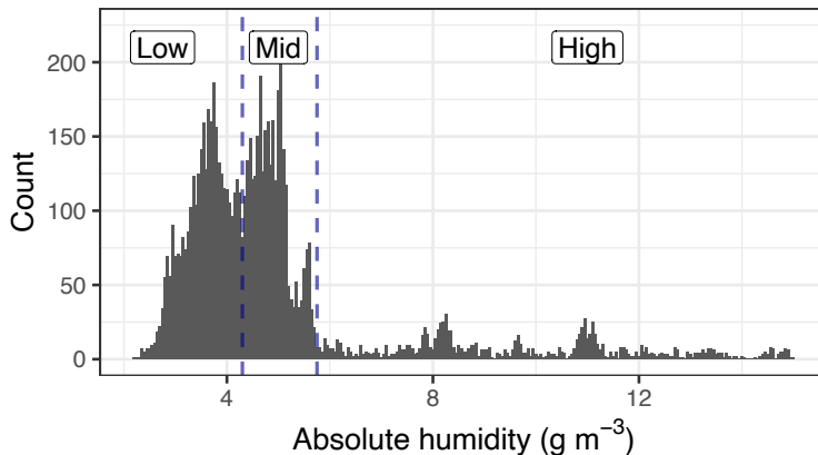
350 Figure 3: Frequency histogram of absolute humidity measurements including absolute humidity categories used for data analysis. The Low-Mid boundary is at 4.30 \text{ g}_{H_2O} \text{ m}^{-3} , and the Mid-High boundary at 5.75 \text{ g}_{H_2O} \text{ m}^{-3} .
