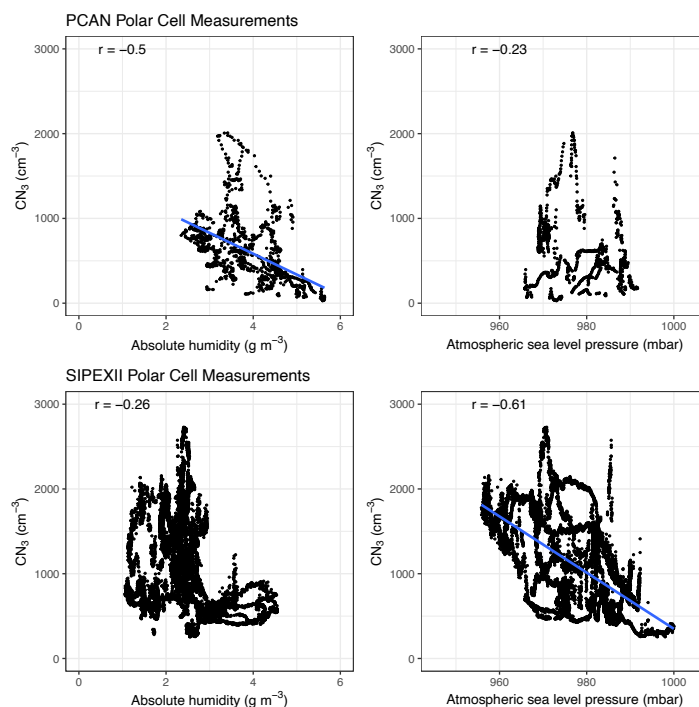
585 Figure 6: Comparison of PCAN (top row) and SIPEXII (bottom row) AH and atmospheric sea level pressure measurements plotted against CN_3 measurements in the Polar cell. Linear regression lines are plotted on the stronger relationship for each voyage. Pearson's r values are plotted on each facet.
