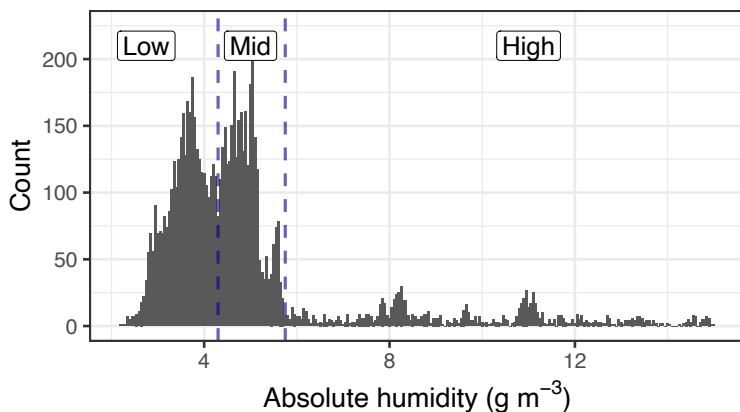
Figure 4: Frequency histogram of absolute humidity measurements including absolute humidity categories used for data analysis. The Low-Mid boundary is at 4.30\ g_{H_2O}\ m^{-3} , and the Mid-High boundary at 5.75\ g_{H_2O}\ m^{-3} .
