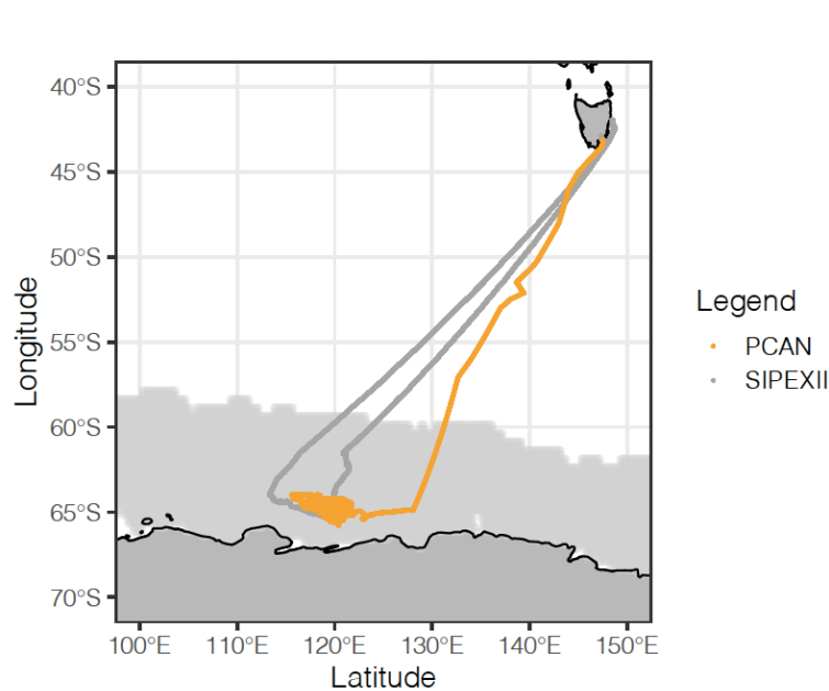
140 Figure 1: Voyage tracks of the SIPEX-II and PCAN voyages. Voyage tracks of the SIPEX-II (spring 2012, grey) and periods of the PCAN voyage (summer 2017, orange) for which measurements were analysed: measurements from the southward transit are excluded due to instrument malfunction. indicates the voyage period for which measurements were analysed. Measurements from the southward transit are excluded due to instrument malfunction. Grey shading represents the sea ice area observed at the midpoint of the SIPEXII voyage as detected by the Nimbus-7 satellite (National Snow and Ice Data Centre, 2021). No sea ice was present in the plotted region at the midpoint of the PCAN voyage. An interactive map of RV Investigator voyage tracks can be found here: https://www.cmar.csiro.au/data/underway/?survey=in2017_v01 .
