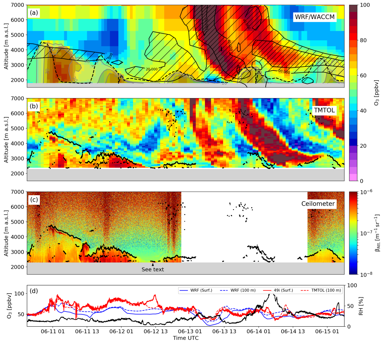
Figure 16. Overview of the model outputs and measurements over TMF between 10 June 15:20 and 15 June 7:10 UTC. Panel descriptions are the same as the ones shown for Fig. 1310.
