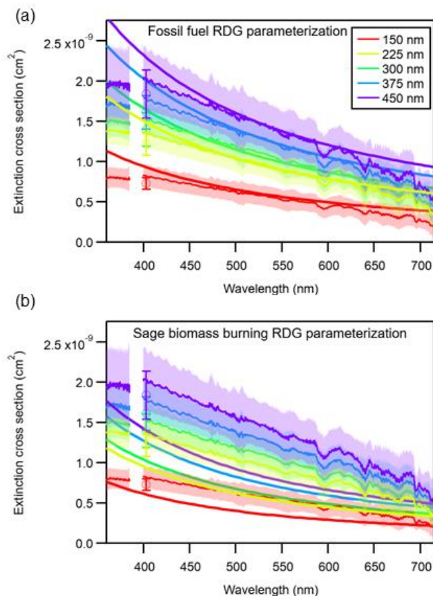
605 Figure 6. Measured extinction cross section of thermodenuded black carbon dominated aerosol in Fire B are shown in the thin solid lines. Calculated extinction cross section for different RDG parameters (Eq. (4)) are shown in each panel. (a) Fossil fuel RDG parameters from Sorensen et al (2001); (b) Biomass burning RDG parameters for sage from Chakrabarty (2006). The measurement lies between these two parameterizations, thereby constraining the RDG prefactor and fractal dimension, but is closer to the fossil fuel parameterization.
