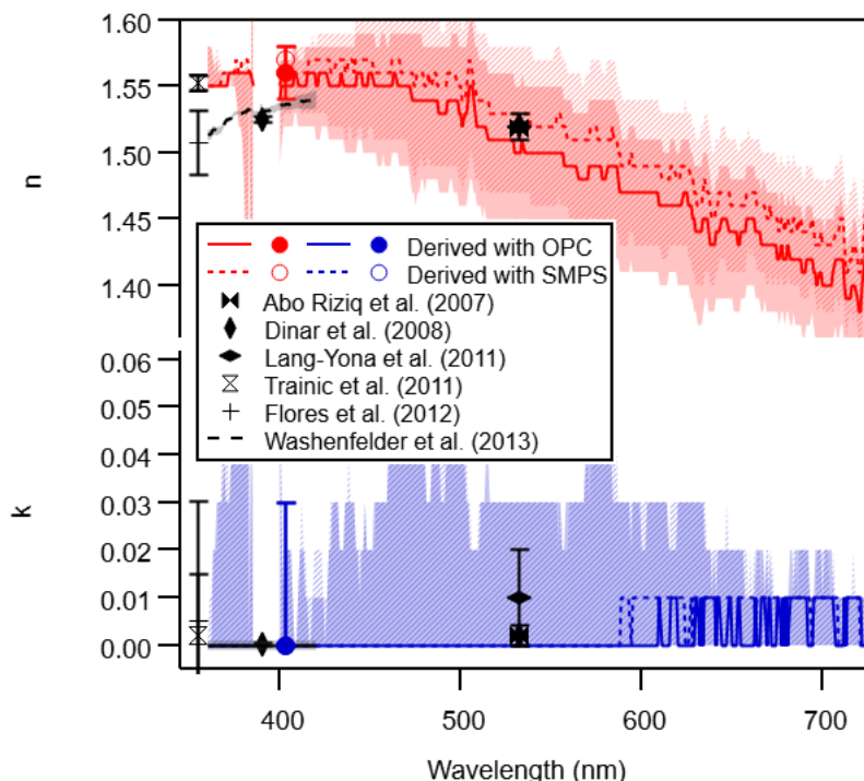
Figure 4. The RI retrieved for ammonium sulfate aerosol, using two particle size distribution methods: an OPC (LAS 3340) and a DMA operating in SMPS mode. Both retrievals agree well with literature values for ammonium sulfate between 350 and 550 nm. As in Fig 3, the RI is retrieved to the nearest 0.01, and an absence of a visible error bar implies that the calculated error is smaller than 0.01.
