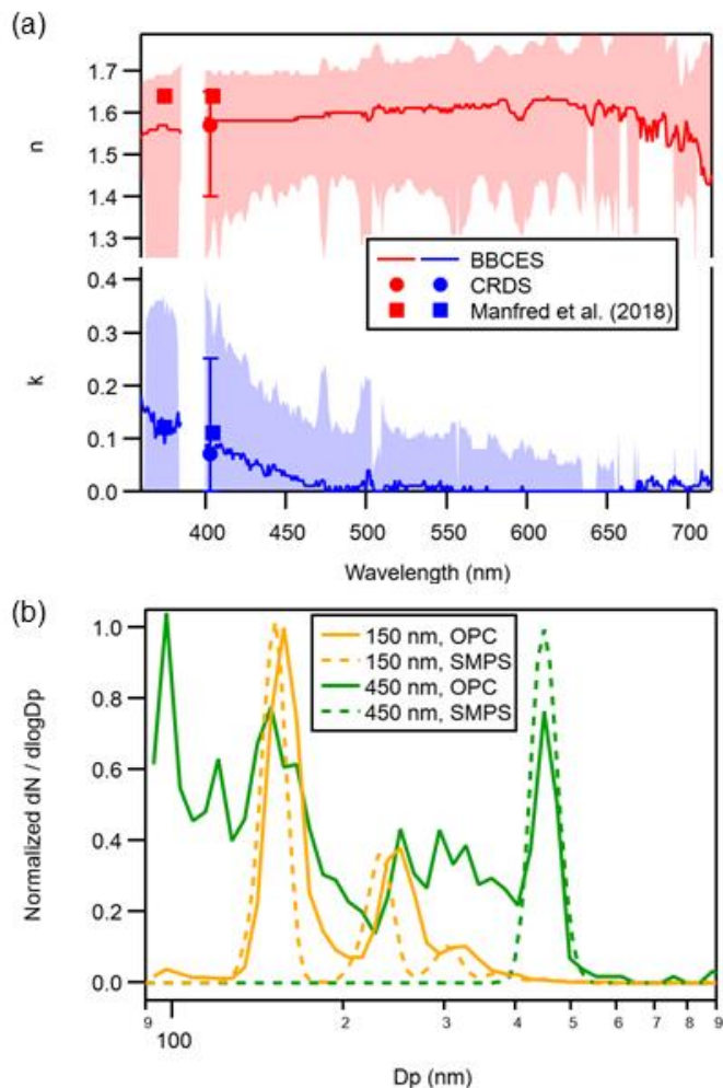
Figure 5. (a) Retrieved RI of undeneded smoke during Fire A, a primarily brown carbon fire. The BBCES and CRDS retrievals are shown in solid line and circular markers. The squares indicate the assumed RI in Manfred et al. (2018) for this fire. The increase in the scattering component, k , with decreasing wavelength is characteristic of brown carbon aerosol. (b) The normalized size distribution of the aerosol from the OPC and the SMPS for two size set points, 150 and 450 nm. The 150 nm OPC measurement has a small peak near 100 nm but otherwise shows reasonable agreement with the SMPS, while the 450 nm setpoint OPC distribution shows a significant fraction of the aerosol is smaller than 450 nm, which is not reflected in the SMPS estimate. The other size setpoints lie in between these two extremes.
