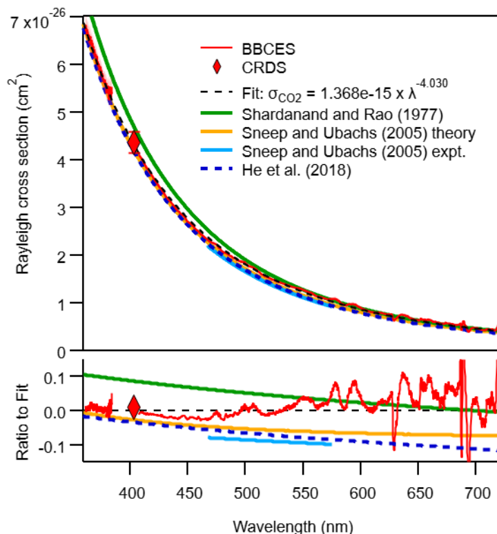
Figure 2. The measured Rayleigh scattering cross section of CO 2 . The red solid line and filled diamond show the measurement by BBCES and CRDS, respectively, with black dashed line showing the power-law fit to the measured data. Several other literature parameterizations are shown in solid colored lines, and discussed further in the text. The ratio of each trace relative to the power-law fit derived here is shown at the bottom, and all are within 10% of the fit derived here. The small peaks and valleys observed in the experimental fit are due to imperfect subtraction of peaks from O 2 and the O 4 oxygen dimer.
