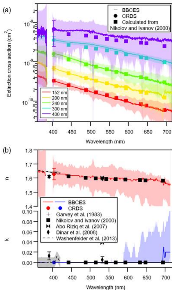
Figure 3. (a) Measured extinction cross sections for five diameters of PSL spheres are shown as solid lines, with 2\sigma error bars designated by shaded regions. The theoretical extinction cross section calculated from the RI of Nikolov and Ivanov (2000) and the measured aerosol size distribution is shown as filled squares for each diameter set point. (b) The retrieved RI of PSL spheres derived from the measurement in (a) and the size distribution measured by the OPC. The RI is retrieved to the nearest 0.01, and the absence of a visible upper or lower error bar implies the calculated error is less than 0.01. The RI retrieved by Nikolov and Ivanov (2000) is shown in black squares. The error increases at longer wavelengths due to increased uncertainty in the \text{CO}_2 Rayleigh scattering spectrum.
