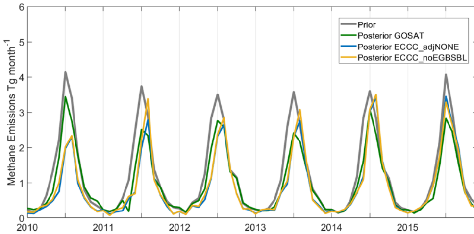
Figure AR2: Sensitivity analysis of inversion results depending on the inclusion of sites EGB and SBL which are sensitive to cross-border transport from the United States. Similar to AR1, the prior emissions (gray) are compared to the posterior results using GOSAT (green), and the posterior using ECCC data including all sites (blue) and ECCC data excluding EGB and SBL (yellow).
