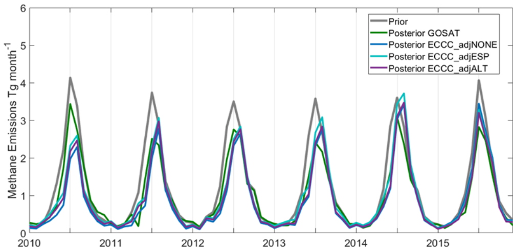
Figure AR1: Sensitivity analysis of inversion results depending on the use of background correction for ECCC data. Referred to as the monthly inversion, this approach optimizes annual total Canadian anthropogenic emissions (top) and monthly total natural emissions (bottom) in an n = 78 state-vector element setup. The prior emissions (gray) are compared to the posterior results using GOSAT (green), and the posterior using ECCC data with an unadjusted background error (blue), ECCC data using a background adjusted according to the yearly difference at ESP (teal) and ALT (purple) from Table AR1.
