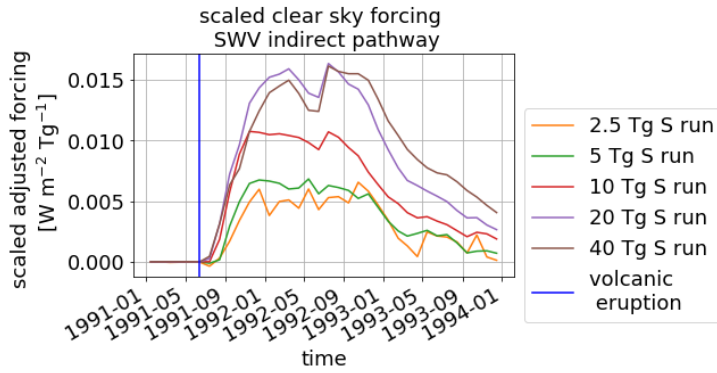
Figure A5. Scaled time evolution of the adjusted clear sky SW-forcing in the tropical region [-5,5]^\circ latitude for all eruption strengths. The blue line marks the eruptions time. All clear sky forcings are divided by the mass of emitted sulfur. Incoming fluxes are defined positive, outgoing fluxes are defined negative
