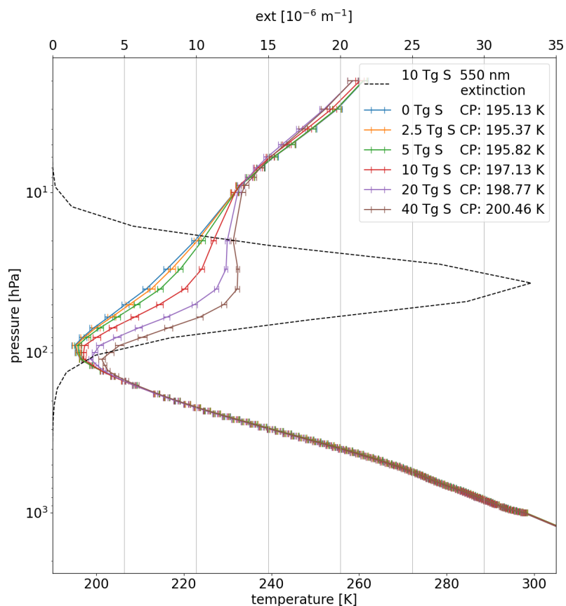
Figure 3. Inner tropical average of the temperature profiles for the five volcanically perturbed EVAens runs (2.5 Tg S, 5 Tg S, 10 Tg S, 20 Tg S and 40 Tg S) in September 1991 (three months after the eruption). The temperature of the respective cold point (CP) is indicated in the legend. The solid line represents the ensemble mean, the error bars symbolize the ensemble standard deviations. The 550 nm extinction values for the 10 Tg S aerosol profile are shown with a dashed black line.
