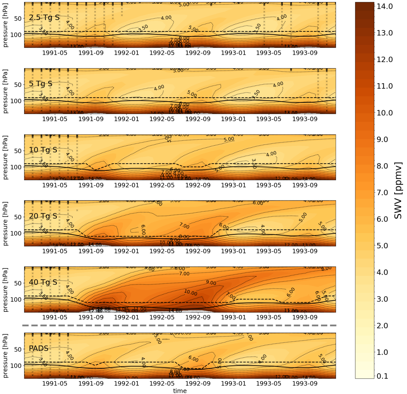
Figure 6. Tropical average in [-23,23]^{\circ} latitude of WV above 140 hPa for sulfur injections of 2.5 Tg S, 5 Tg S, 10 Tg S, 20 Tg S and 40 Tg S as well as the PADS dataset. The WMO-tropopause pressure is indicated by a black line and the cold point pressure is shown as black dashed line. Absolute values are shown. In regions not covered by black crosses statistical significant difference between water vapour values of the perturbed and unperturbed runs (t-test at p=0.05 ) were found. 14
