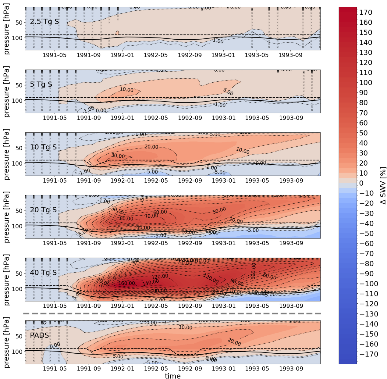
Figure B1. Percentual difference in water vapour above 140 hPa in the tropical average over [-23,23]^{\circ} latitude for the pure sulfur injections of the EVAens (2.5 Tg S, 5 Tg S, 10 Tg S, 20 Tg S and 40 Tg S). The lowermost panel shows the MPI-GE historical simulations for Mt. Pinatubo using the PADS forcing data set. The height of the WMO-tropopause is indicated by a black line, the cold point pressure is shown as black dashed line. In regions not covered by black crosses statistical significant difference between stratospheric water vapour values of the perturbed and unperturbed runs (t-test at p=0.05 ) were found.
