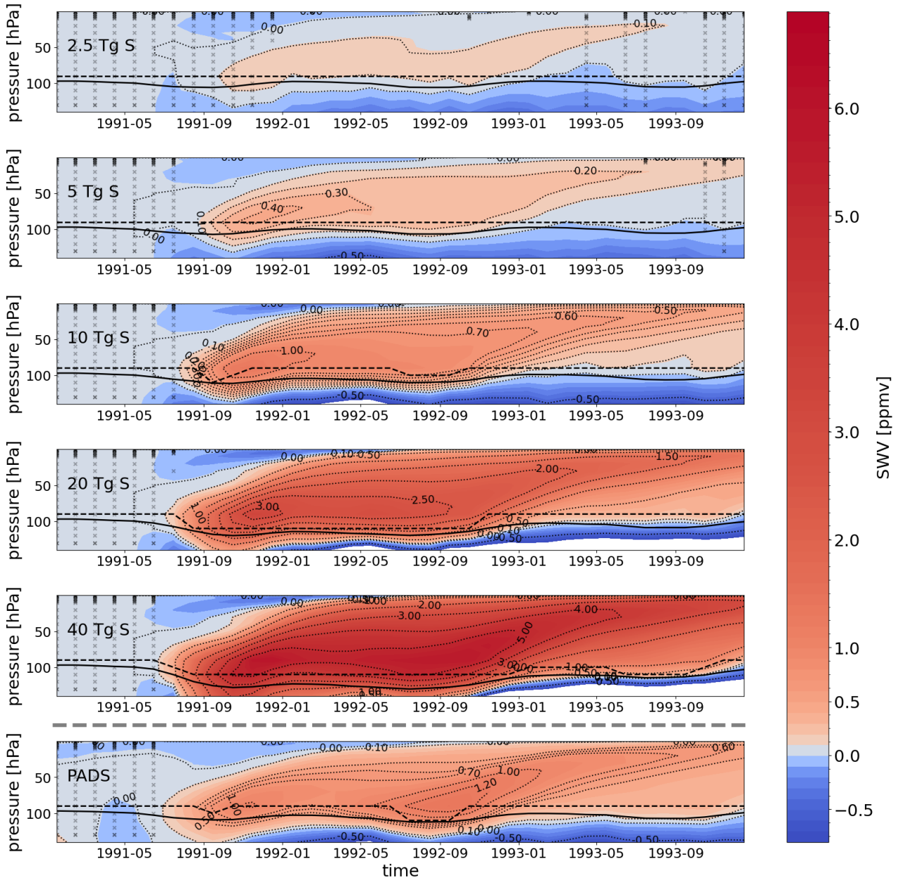
Figure 7. Tropical average in [-23,23]^{\circ} latitude of WV anomalies above 140 hPa for the sulfur injections of 2.5 Tg S, 5 Tg S, 10 Tg S, 20 Tg S and 40 Tg S as well as the PADS dataset. The lowermost panel shows the MPI-GE historical simulations for Mt. Pinatubo using the PADS forcing data set discussed in Sect. 3.5. The WMO-tropopause pressure is indicated by a black line and the cold point pressure is shown as black dashed line. Differences with respect to the 0 Tg S control run are shown. In regions not covered by black crosses statistical significant difference between water vapour values of the perturbed and unperturbed runs (t-test at p=0.05 ) were found.
