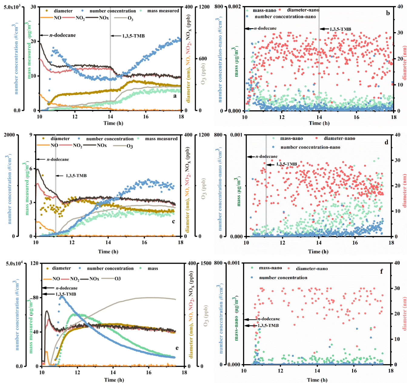
Figure 3. (a) reaction profiles of experiment MIX-6; (b) time series of particles in the size range of 0-40 nm for MIX-6; (c) reaction profiles of experiment MIX-7; (d) time series of particles in the size range of 0-40 nm for MIX-7; (e) reaction profiles of experiment MIX-4; (f) time series of particles in the size range of 0-40 nm for MIX-4. The concentrations of mass and number concentration of particles are shown on the left axes, while the diameter of particles and concentrations of NO, NO 2 , NO x , and O 3 are shown on the right axes. The vertical gray lines in the figures refer to the time that 1,3,5-TMB was added.
