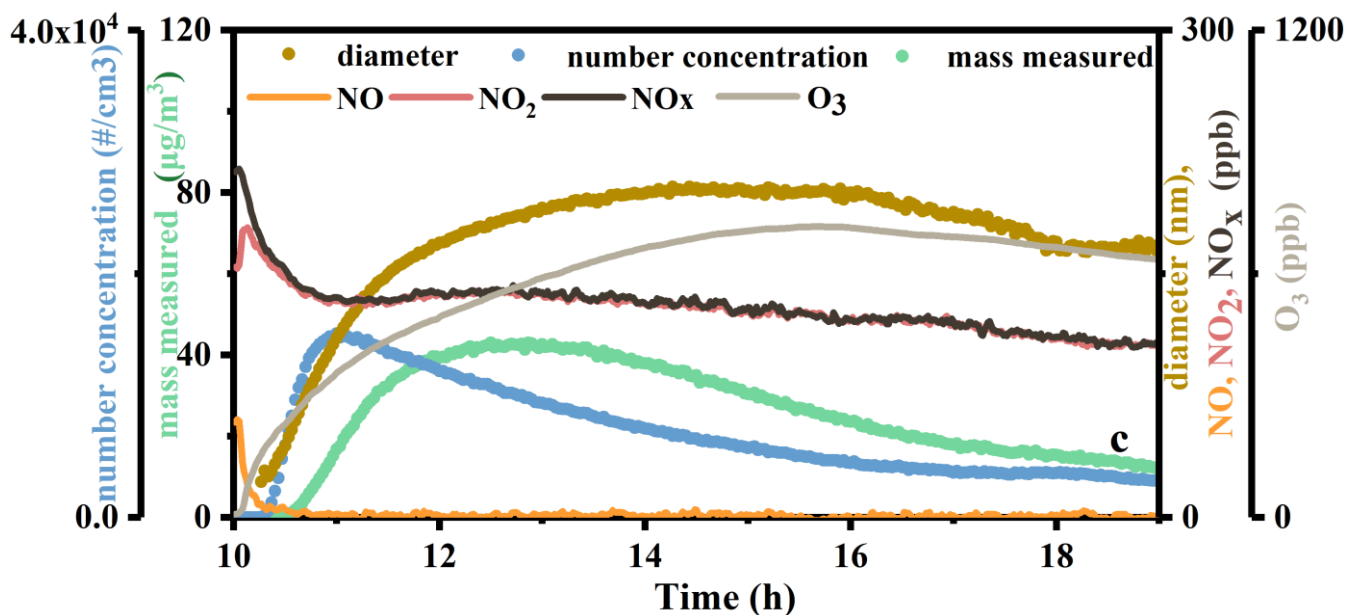
Figure 1. Reaction profiles of photooxidation of n-dodecane (a), 1,3,5-TMB (b), and mixture AVOCs (c) under NO x conditions in summer. The concentrations of mass and number concentration of particles are shown on the left axes, while the diameter of particles and concentrations of NO, NO 2 , NO x , and O 3 are shown on the right axes.
