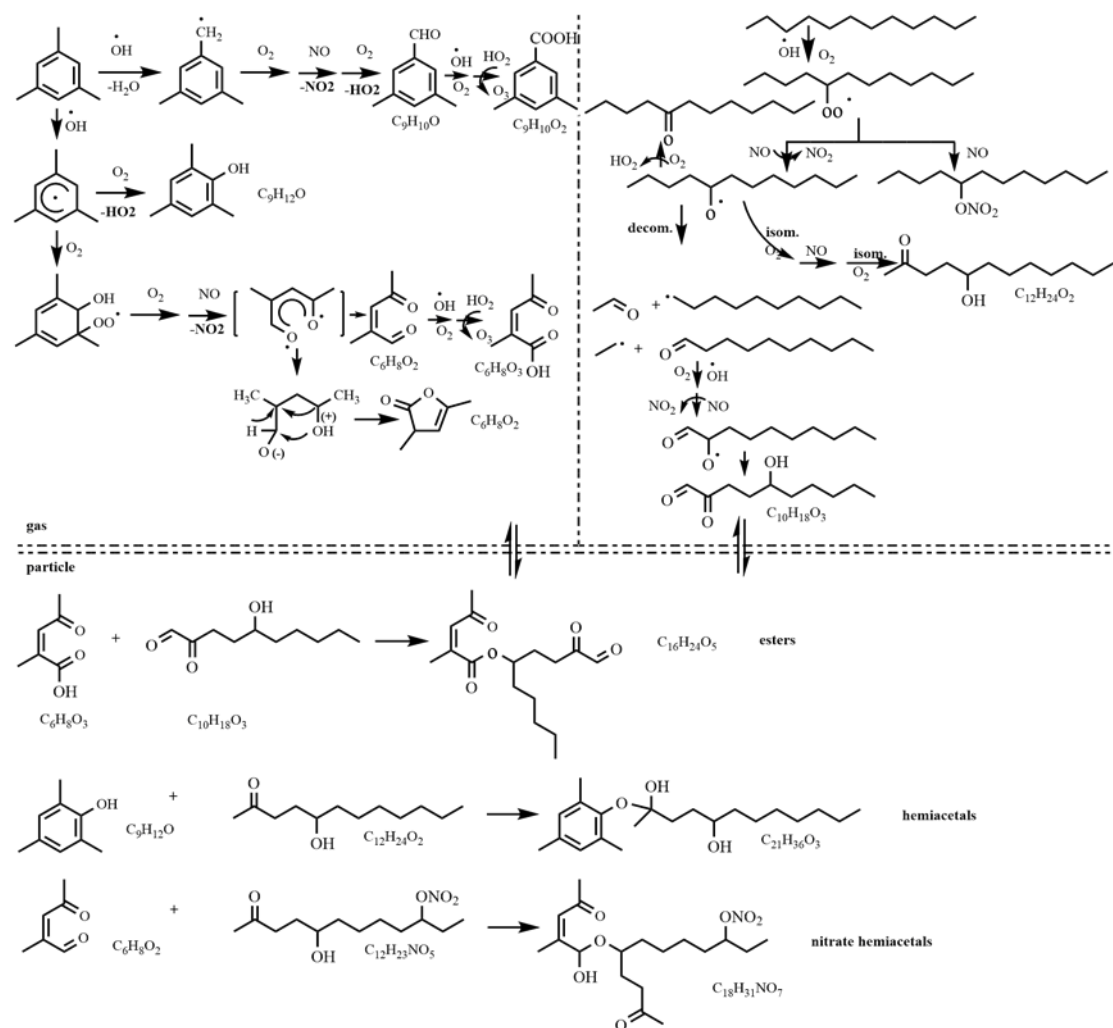
Figure 5. Proposed reaction mechanism of mixture AVOCs system in the presence of \text{NO}_x (R1 and R2 are alkyl groups or aromatic hydrocarbon groups).
