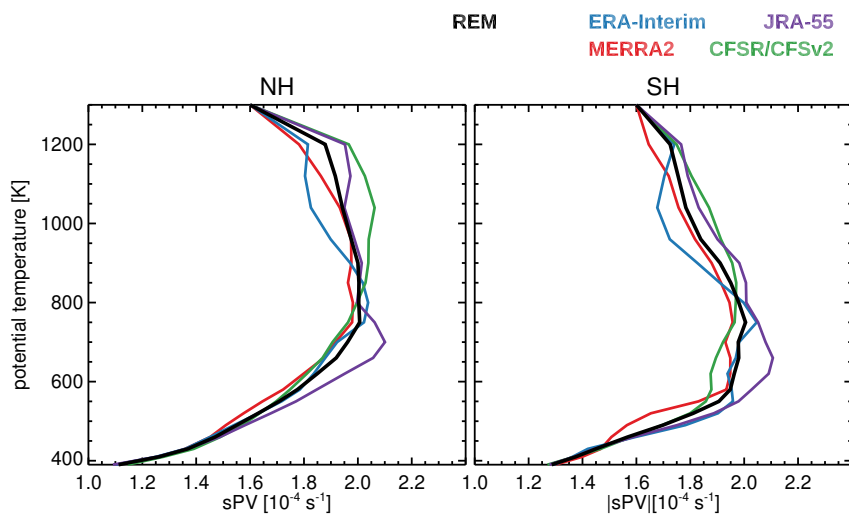
Figure 9. sPV vortex definition for each reanalysis as well as for the REM. These were constructed using climatological values from 1980–2014 data.
