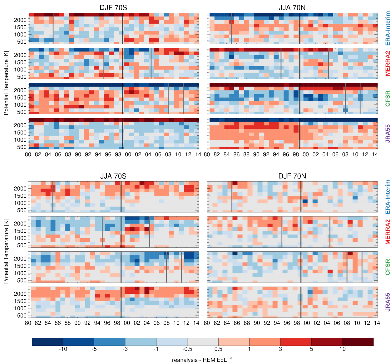
Figure 6. EqL differences for each reanalysis from the REM as a function of year and potential temperature. (top panels) summer hemispheric differences, (bottom panels) winter hemispheric differences at 70°S and 70°N. Vertical lines show the discontinuities associated with changes in assimilated datasets or different processing streams.
