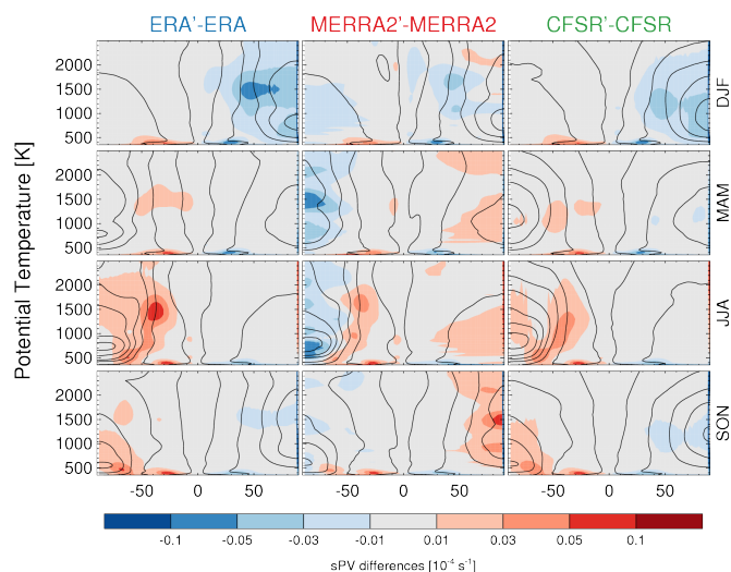
Figure 4. Differences between the sPV from each reanalysis provided vorticity or PV and the sPV computed from that reanalyses' horizontal wind, pressure, and temperature fields. Overlaid contours show each reanalyses' climatology based on that reanalyses' provided vorticity.
