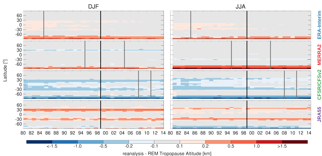
Figure 8. 2PVU tropopause altitude zonal mean differences for each reanalysis from the REM as a function of year. (left) DJF and (right) JJA differences. Vertical lines show the discontinuities associated with changes in assimilated datasets or different processing streams.
