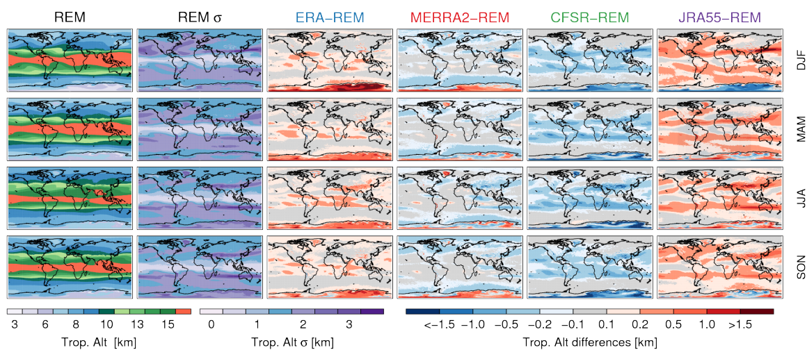
Figure 7. (left columns) Climatological REM 2 PVU tropopause altitudes and standard deviations for different seasons. (right columns) Difference of each reanalysis from the REM.
