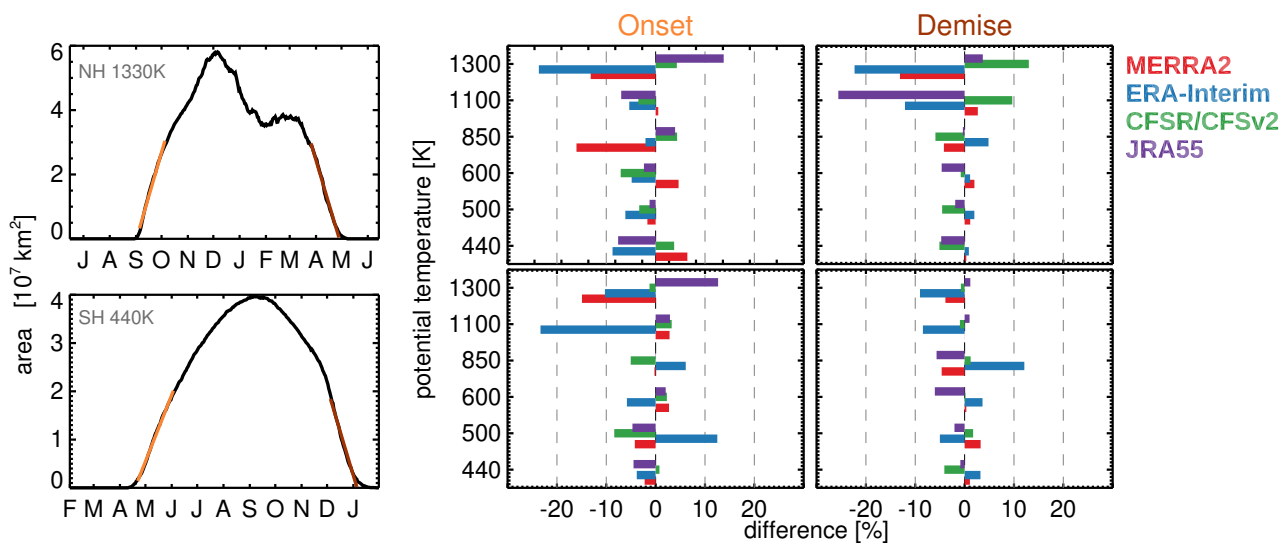
Figure 13. (left) Examples of the linear fits applied during onset and demise of the vortex in the REM (see text). (right) Percent difference between the linear fits' slopes for each reanalysis from the REM; (top) Northern Hemisphere and (bottom) Southern Hemisphere.
