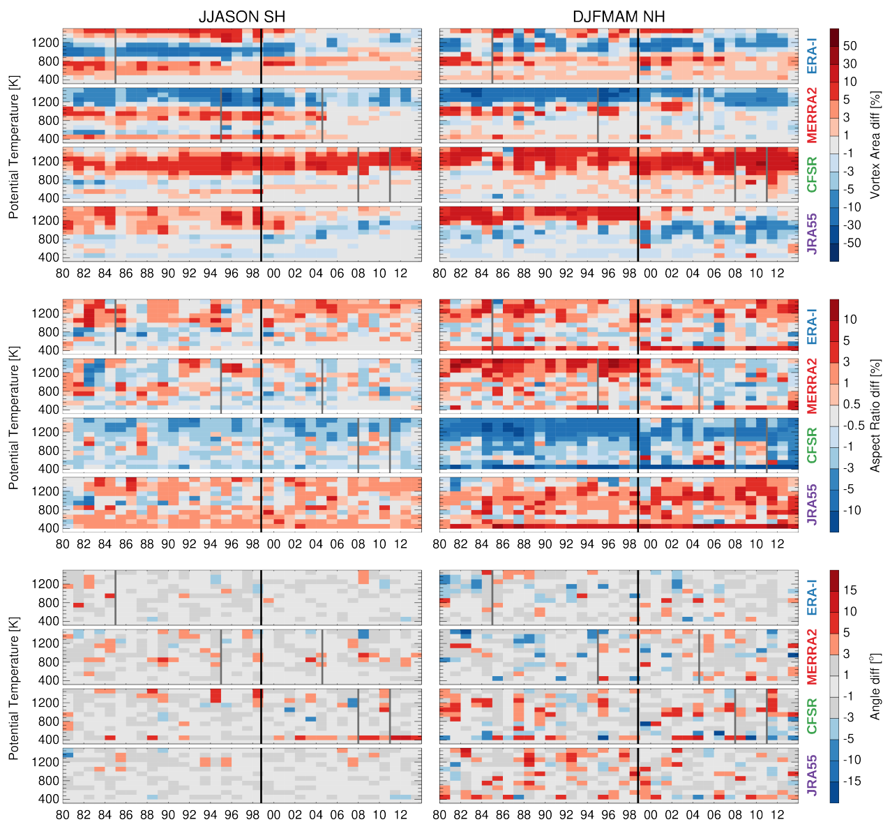
Figure 15. Vortex area, aspect ratio, and angle differences for each reanalysis from the REM as a function of year and potential temperature. Only vortices greater than 0.15 \cdot 10^7 \text{ km}^2 were considered. Vertical lines show the discontinuities associated with changes in assimilated datasets or different processing streams.
