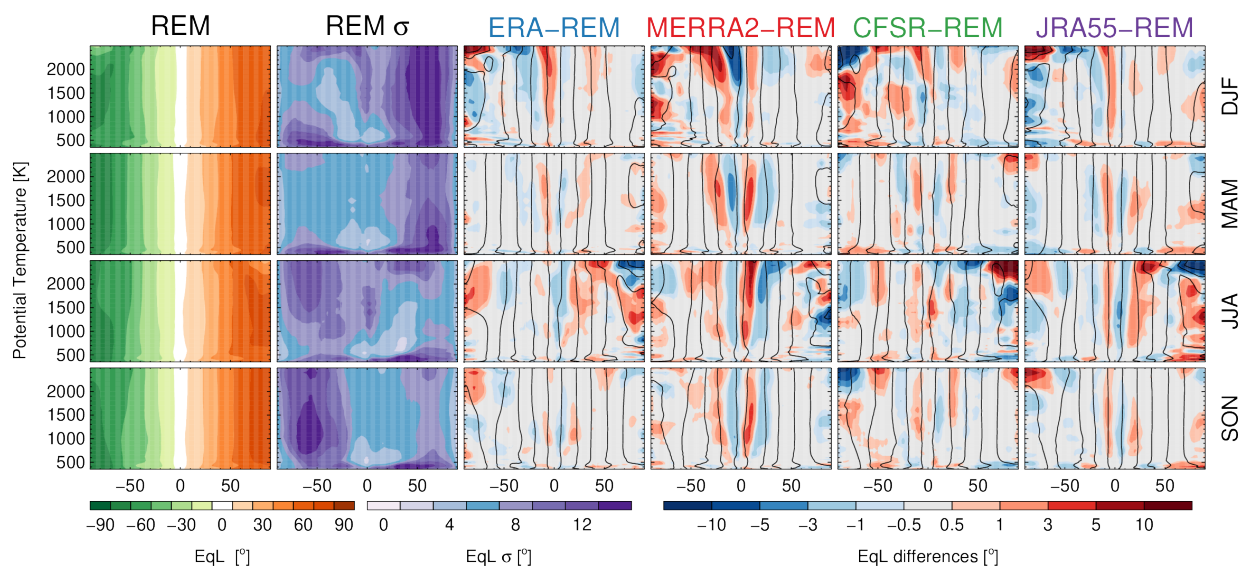
Figure 5. (left columns) Equivalent latitude REM seasonal climatological mean and standard deviation for different seasons. (right columns) Equivalent latitude difference between each reanalysis and the REM. Overlaid contours show each reanalysis fields respective climatology.
