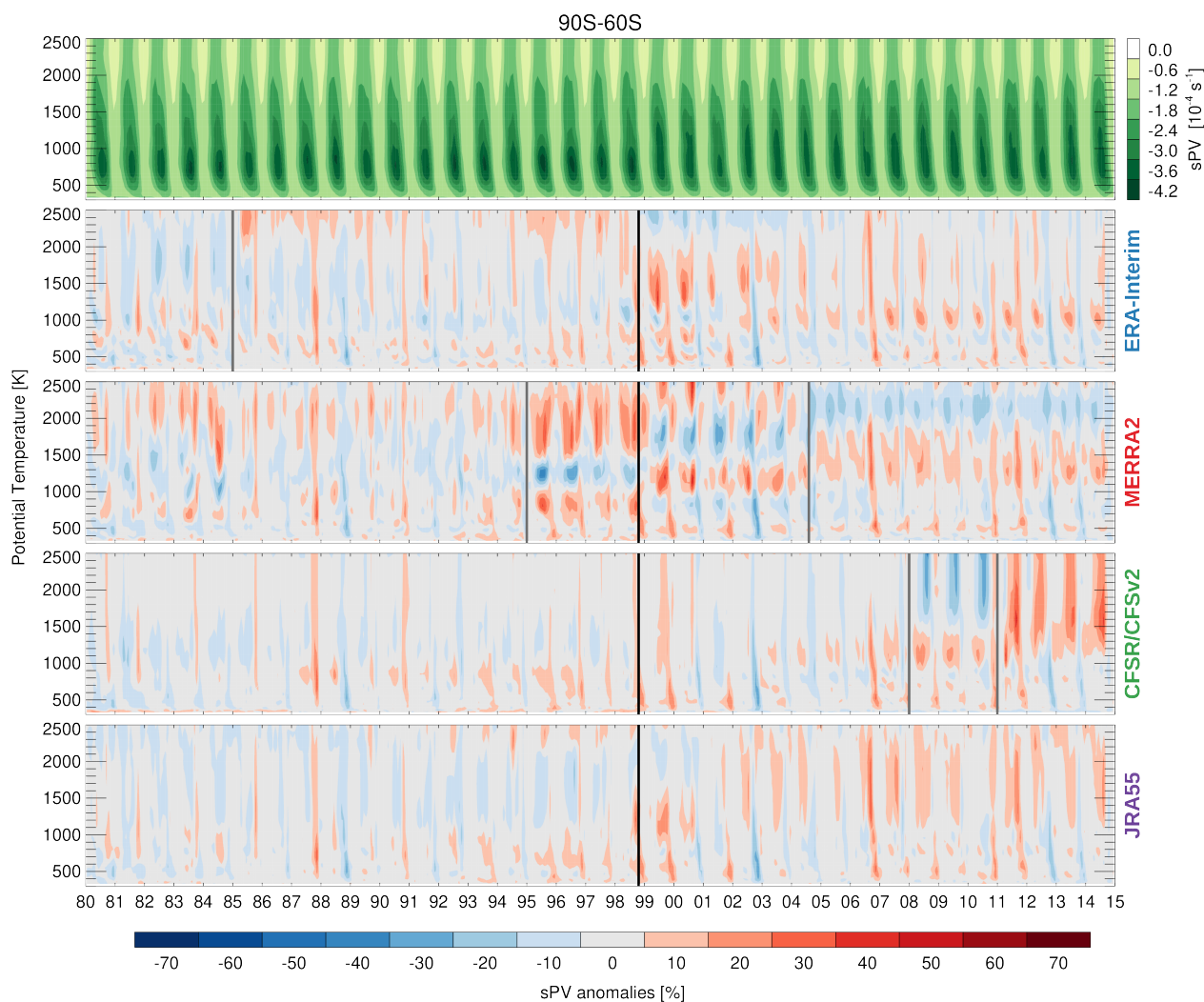
Figure 1. (top panel) sPV REM timeseries. (bottom panels) sPV anomalies with respect to each reanalyses' own monthly climatological values. Vertical lines show the discontinuities described in the text.
