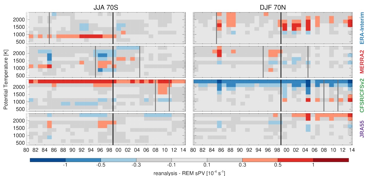
Figure 3. sPV differences for each reanalysis from the REM as a function of year and potential temperature. (left) JJA at 70°S and (right) DJF at 70°N differences. Vertical lines show the discontinuities associated with changes in assimilated datasets or different processing streams.
