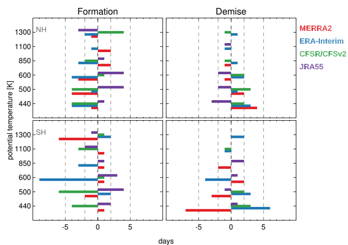
Figure 12. Climatological difference in days between the reanalysis and the REM vortex formation and decay dates.
