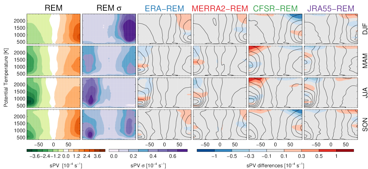
Figure 2. (left columns) sPV REM seasonal climatological mean and standard deviation. (right columns) sPV difference between each reanalysis and the REM, line contours show each reanalyses' seasonal climatology.
