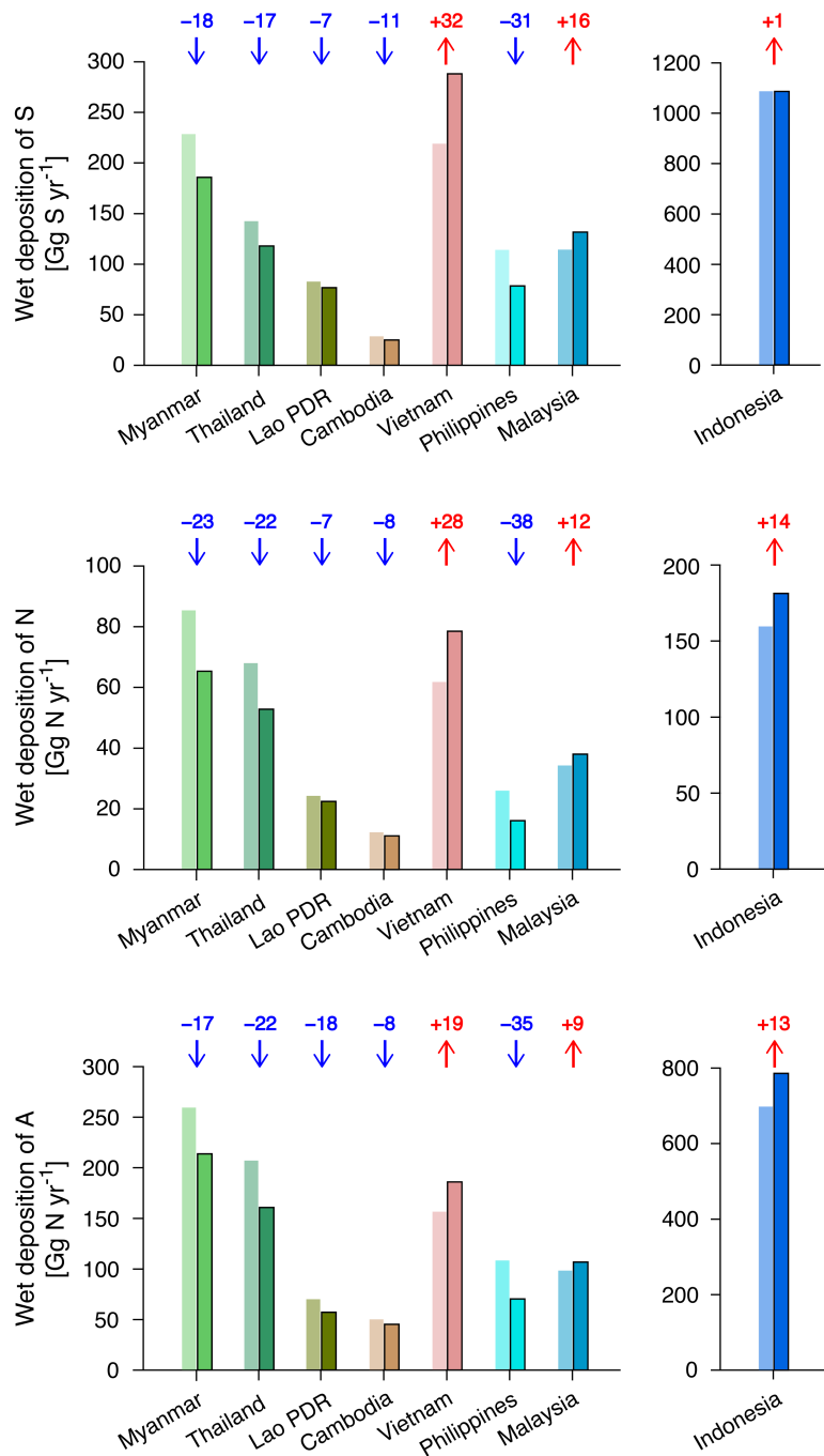
Figure 18: Simulated annual accumulated wet deposition amounts of (top) S, (center) N, and (bottom) A over Southeast Asian countries calculated by ENS (light bars without outlines) and AS (dark bars outlined in black). Blue numbers with down-facing arrows indicate downward revision by AS and red numbers with upward-facing arrows indicate upward revision by AS.
