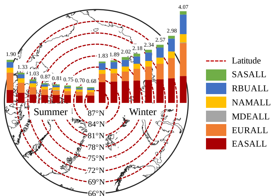
Figure 6. Contributions of 20% emission reductions of different regions to near-surface BC concentrations in each latitudinal band of the Arctic. The results of summer and winter correspond to the left and right panel in the figure.
