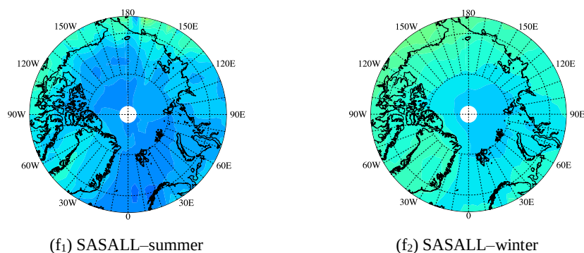
Figure 3. Spatial distribution of contribution of 20% emission reductions of different source regions to Arctic near-surface BC in summer and in winter in 2010.
