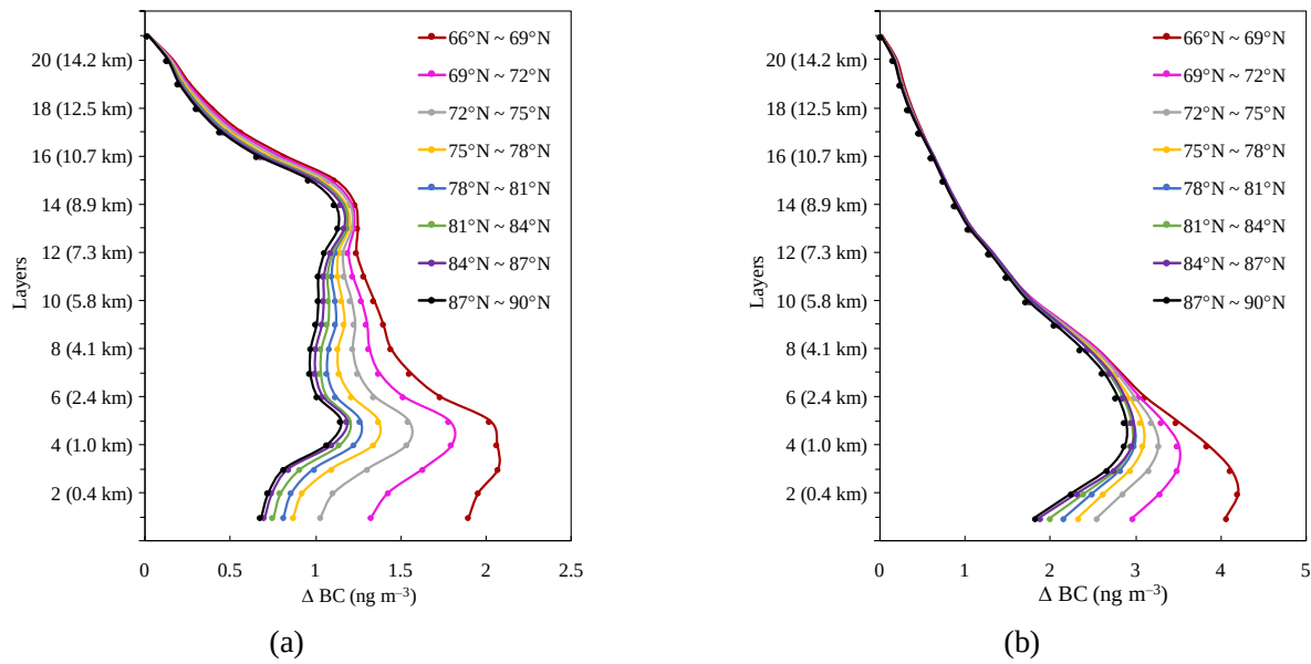
Figure 7. Contributions of 20% emission reductions from all six source regions to the vertical BC concentrations of the Arctic in different latitude bands varies with vertical layers in (a) summer and (b) winter in 2010.
