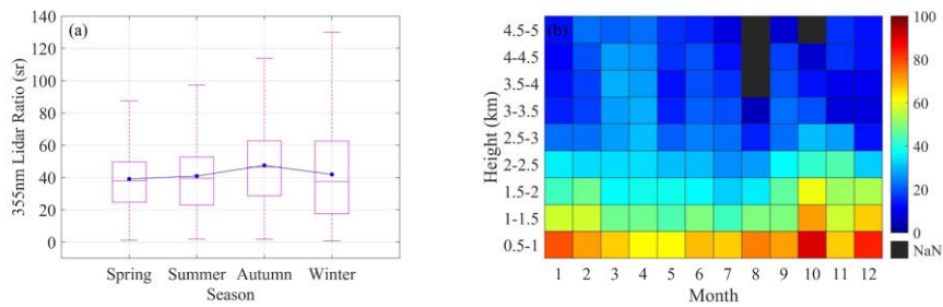
Figure 4: LR temporal variations. (a) Seasonal variations of LR. The blue dots are the average for each season; (b) Average of LR at different altitudes in different months. The black areas indicate invalid value.
