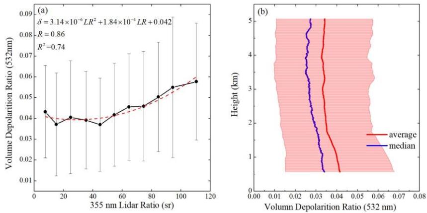
645 Figure 6: Effect of \delta on LR. (a) LR was divided into 11 intervals and the mean value of \delta in each interval was calculated. The dot and error bar represent the mean and standard deviation of \delta in each interval. The red dotted line is the fitting line of LR and \delta ; (b) The red line is the mean profile of \delta , the blue line is the median profile of \delta , and the red shadow is the error bar, meaning the standard deviation.
