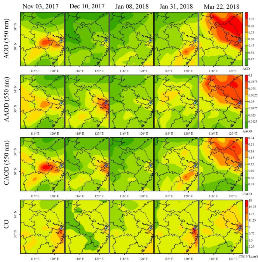
655 Figure 9: Spatial distribution of AOD, AAOD, CAOD and CO column concentrations in 5 cases. From left to right, different cases are represented, and from top to bottom, different tracers are represented. The blue star is the location of the Raman lidar.
