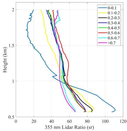
Figure 8: LR profiles in different AOD intervals.
