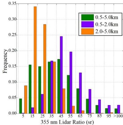
Figure 3: LR frequency distribution.
