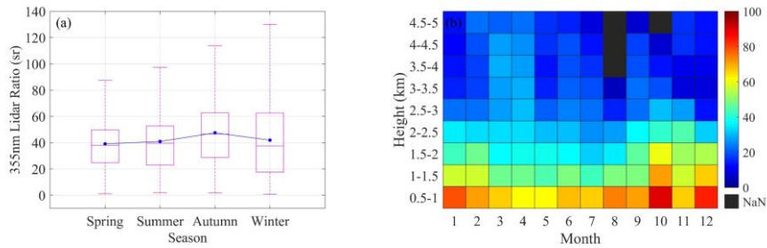
640 Figure 4: LR temporal variations. (a) Seasonal variations of LR. The blue dots are the average for each season; (b) Average of LR at different altitudes in different months. The black areas indicate invalid value.
