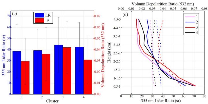
650 Figure 7: (a) 72-h back trajectory cluster analysis; (b) Mean values of LR and \delta corresponding to different air masses; (c) The average of LR and \delta at different heights corresponding to different air masses, the solid line is LR, the dotted line is \delta .
