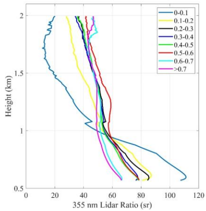
Figure 8: LR profiles in different AOD intervals.
