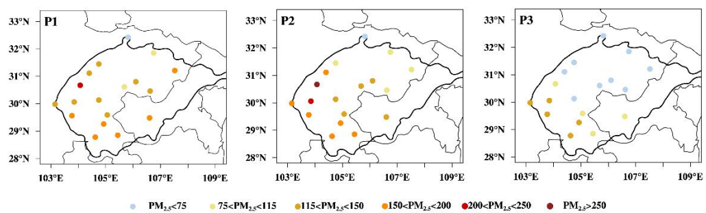
Figure 4. Spatial distributions of observed surface PM 2.5 concentrations in the SCB averaged in the formation, maintenance and dissipation periods, P1, P2 and P3 (Fig. 2b), respectively, of the heavy haze pollution episode over 2–7 January 2017.
