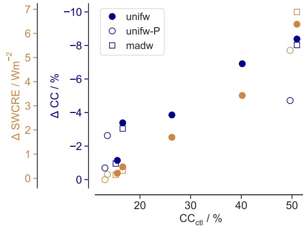
Figure 8. Relationship between cloud cover amount in the control simulation ( CC_{\text{ctl}} ) and cloud cover reduction with warming ( \Delta CC ) as well as the shortwave cloud radiative feedback ( \Delta SWCRE ) across all simulations.
