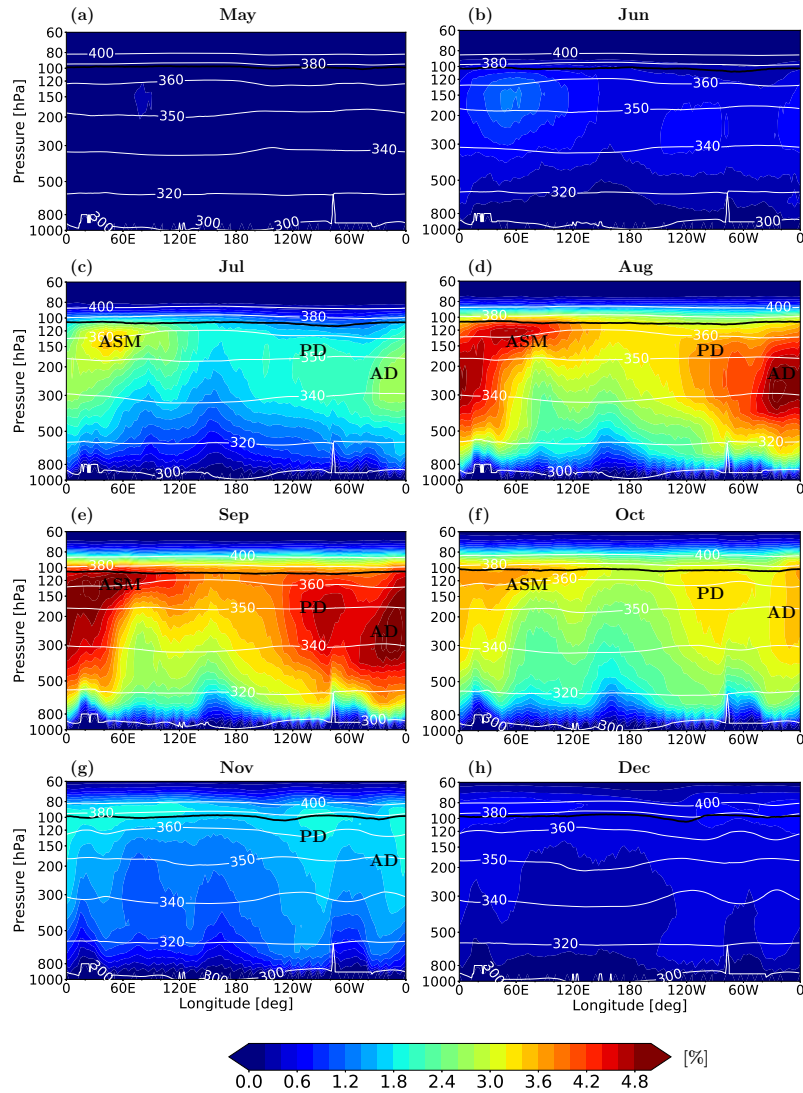
Figure 7. Longitude-pressure cross-section along the latitude of 10^{\circ} S of monthly mean NH extratropical young ( < 3 months) AMF (colour shading) during 1999-2017. White lines show isentropic levels, the black line the WMO tropopause. ASM, PD, and AD respectively indicate the rough locations of the Asian summer monsoon region, Pacific westerly ducts, and the Atlantic westerly ducts.
