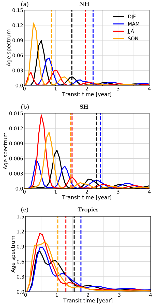
Figure 5. Partial age spectra of the air with the origin in: NH extratropics (a), SH extratropics (b), and tropics (c) calculated at 360 K along 60° N (destination region). Different colours represent different seasons. Vertical dashed lines indicate the mean AoA. Note different ranges of the y-axis (Tropics = 10×NH, NH = 10×SH) which quantify relative differences of the considered source regions.)
