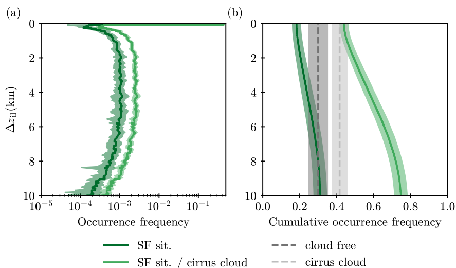
Figure 3. (a) Occurrence frequency of seeder-feeder situations (SF sit.) with respective \Delta z_{i1} as a fraction of measurements (dark green) or cirrus cloud measurements (light green). (b) Cumulative occurrence frequency. For \Delta z_{i1} a vertical resolution of 60 m is used. For comparison, the fraction of measurements with at least one cirrus cloud (light grey) and with a cloud free atmosphere (dark grey) are given. Here and in the following data from all tracks in the study time (2006 to 2017) and within the study domain were used (2210 satellite tracks). The total number of measurements is 1440312, with 853833 measuring \Delta z_{i1} and 355331 measuring cirrus clouds. The shaded areas visualize the standard deviation of interannual variability. Note that \Delta z_{i1} = 0 m is at the base of the lowest cirrus cloud layer with T < -35 °C.
