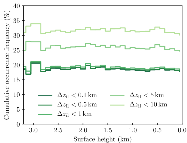
Figure B1. Distribution of \Delta z_{il} with underlying surface topography.
