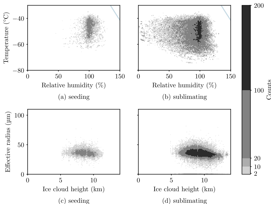
Figure 5. Environmental conditions at cirrus cloud base. Absolute frequency of temperature as a function of relative humidity with respect to ice at cirrus cloud bases with \Delta z_{i1} > 100 m and (a) where spherical ice crystals survive the sedimentation and seed the lower cloud, (b) where spherical ice crystals sublimate before reaching the mixed-phase cloud. The light blue line depicts saturation with respect to water. Absolute frequency of effective ice crystal radius at cirrus cloud base as a function of cirrus cloud height with \Delta z_{i1} > 100 m and (c) where spherical ice crystals survive the sedimentation and seed the lower cloud, (d) where spherical ice crystals sublimate before reaching the mixed-phase cloud. The sum of (c) and (d) is displayed in Fig. 4c. For improved readability the colorbar label for bin 1 is not shown.
