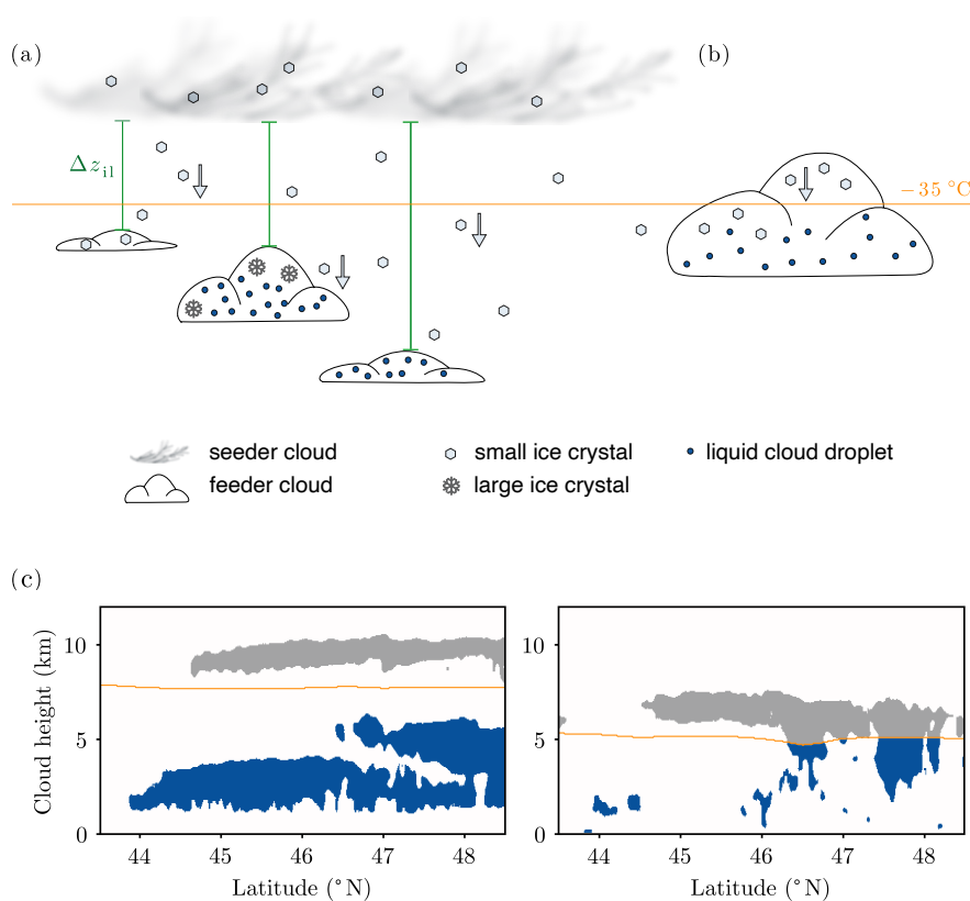
Figure 1. Sketch of the two seeder-feeder situations observed in this study. The orange lines depict the -35^\circ\text{C} isotherm, \Delta z_{il} is the distance between the lowest base of the cirrus cloud and the highest top of the cloud below. (a) Classical external seeder-feeder situation: a cirrus cloud ( T < -35^\circ\text{C} ) is detected at least 100 m above a cloud at T > -35^\circ\text{C} ( \Delta z_{il} > 100\text{ m} ). The latter cloud is termed mixed-phase cloud for simplicity, but could also be liquid or ice phase. (b) In-cloud seeder-feeder situation: the algorithm detects the cloud part above the -35^\circ\text{C} isotherm as a cirrus cloud, and the cloud part below as a mixed-phase cloud ( \Delta z_{il} < 100\text{ m} ). Ice crystal shapes are depicted according to Libbrecht (2005, Fig. 2). (c) Seeder-feeder situations as seen in the DARDAR data. Cirrus clouds above the -35^\circ\text{C} isotherm are depicted in grey, clouds below in blue. Left: exemplary plot of the classical external seeder-feeder situation (data from 29.05.2007), right: exemplary plot of only a mixed-phase or a cirrus cloud present (latitudes equatorwards of 46^\circ\text{N} ) and the in-cloud seeder-feeder situation (polewards of 46^\circ\text{N} , data from 03.12.2010).
