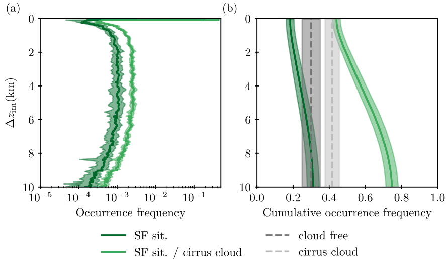
Figure 3. (a) Occurrence frequency of seeder-feeder situations (SF sit.) with respective \Delta z_{im} as a fraction of measurements (dark green) or cirrus cloud measurements (light green). (b) Cumulative occurrence frequency. For \Delta z_{im} a vertical resolution of 60 m is used. For comparison, the fraction of measurements with at least one cirrus cloud (light grey) and with a cloud free atmosphere (dark grey) are given. Here and in the following data from all tracks in the study time (2006 to 2017) and within the study domain were used (2210 satellite tracks). The total number of measurements is 853833, with 267354 measuring \Delta z_{im} and 355331 measuring cirrus clouds. The shaded areas visualize the standard deviation of interannual variability. Note that \Delta z_{im} = 0 m is at the base of the lowest cirrus cloud layer with T < -35 °C.
