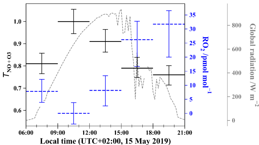
Figure 4. Daytime evolution of T_{NO+O_3} (solid black slots) estimated from Eq.(4) using measured \Delta^{17}O(NO_2) in Grenoble, and of RO 2 mixing ratios (dashed blue slots) estimated from Eq.(6). Error bars for T_{NO+O_3} are derived from standard deviations of \Delta^{17}O(NO_2) and \Delta^{17}O(O_3^*) measured in Grenoble (Vicars and Savarino, 2014). RO 2 error bars are derived from O 3 measurement uncertainties and errors on T_{NO+O_3} (by comparison, errors on reaction constants can be neglected). Global solar radiation flux is represented by dashed lines (measured at 200 meters from the sampling site by the IGE weather station with a Skye SP1110 pyranometer).
