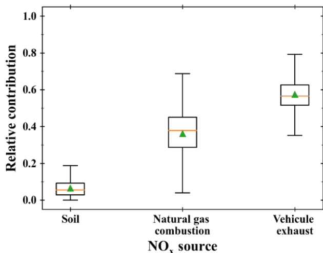
Figure 5. Potential NO x emission source partitioning using the SIAR model based on estimated δ 15 N(NO x ). Reference values for each source were taken from Miller et al. (2017), Walters et al. (2015) and, Zong et al. (2017).
