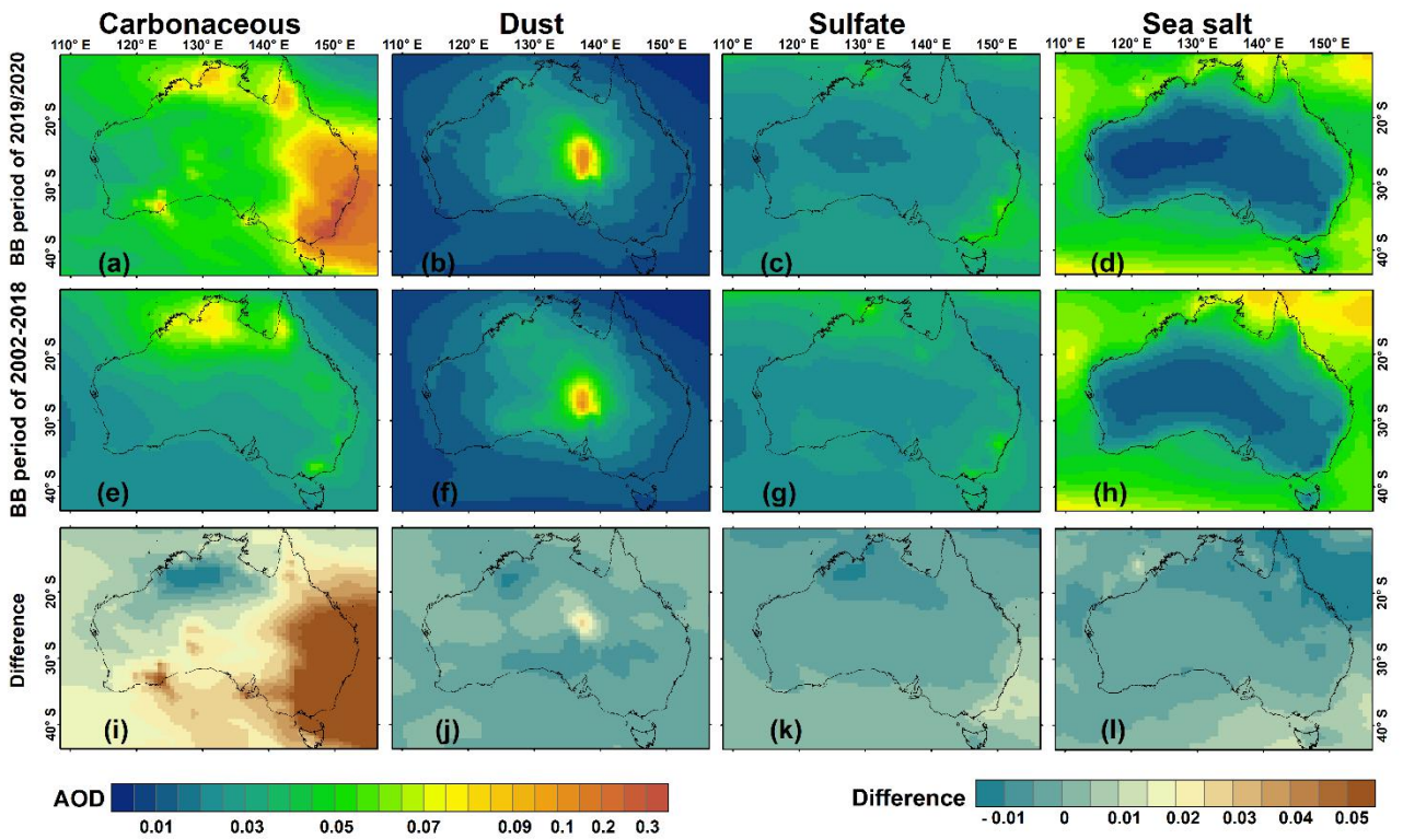
765 Figure 14. Spatial distributions of carbonaceous, dust, sulfate, and sea salt AODs from MERRA-2 during BB period of 2019/2020 (first row), BB period of 2002-2018 (second row), and the differences between the two periods (third row) over Australia.
