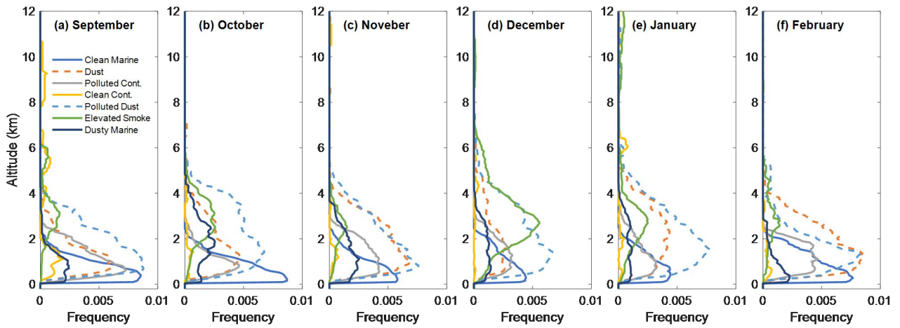
760 Figure 13. Occurrence frequency profile of each aerosol type during the period September 2019-February 2020 from CALIPSO L3 aerosol profile data product in southeastern Australia (the selected domain is the gray shadow area in southeastern Australia in Fig.1(b)).
