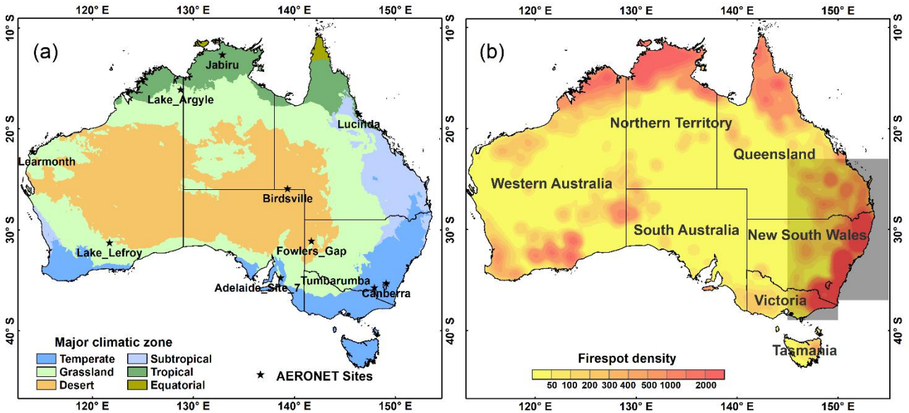
715 Figure 1. (a) Climatic zones of Australia defined by Köppen climate classification system. The black stars represent ten AERONET sites located in Australia. The classified climate zones of Australia were obtained from Bureau of Meteorology of Australian Government ( http://media.bom.gov.au ). (b) Kernel density estimation (KDE) of the number of wildfire events based on MCD14DL with confidence level greater than 50% over Australia from Jun 2019 to May 2020. The Gray shade area is the selected domain for vertical profile analysis in this study.
