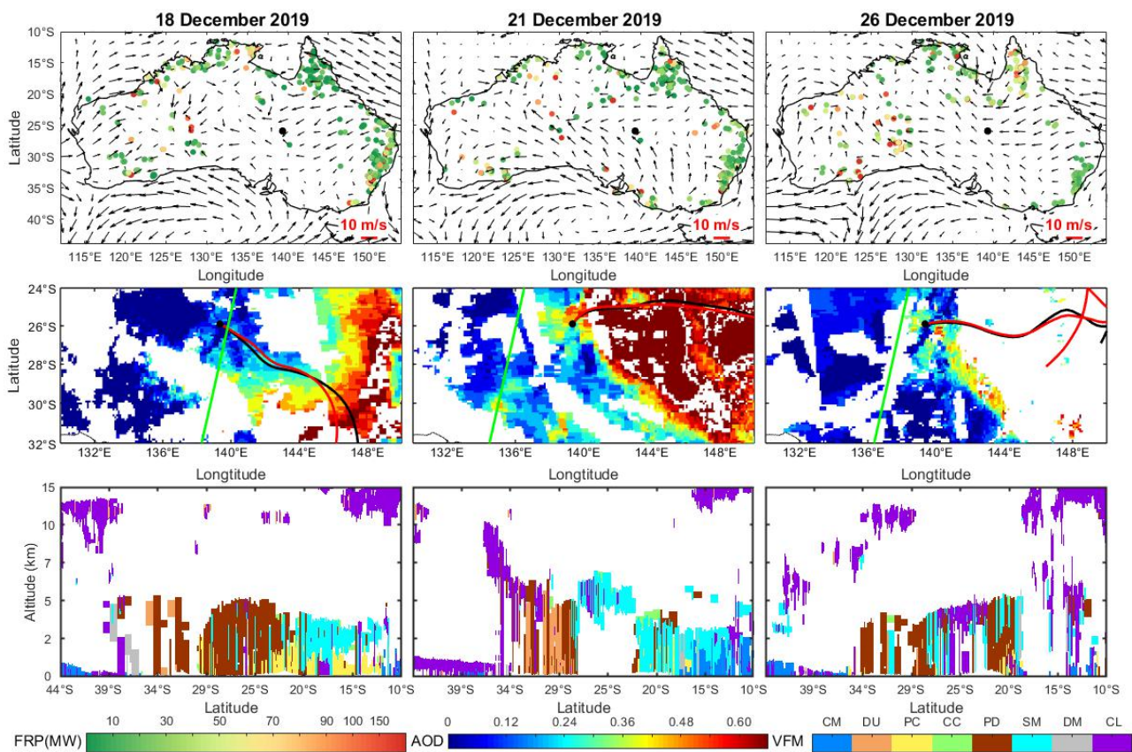
770 Figure 16. Spatial distributions of fire spots (points) from MCD14ML and winds (arrows) from the ERA-5 over Australia (the first row), the Aqua MODIS DB AOD at 550 nm and 72 h back trajectories ending at two heights above the ground level (500 m in red and 200 m in black lines) at Birdsville (the second row), and the vertical feature mask of aerosol on 18, 21 and 26 December 2019 (the third row). (CM: Clean Marine; DU: Dust; PC: Polluted Cont.; CC: Clean Cont.; PD: Polluted Dust; SM: Smoke; DM: Dusty Marine; CL: Cloud). The black dot in in the panels of the first and second rows represent the 775 Birdsville site. The green lines in the panels of the second row represent the scanning orbit path of the CALIPSO satellite.
