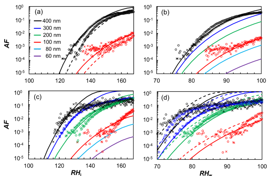
Figure 7. Fraction of soot particles that nucleate ice, termed activated fraction (AF) (Eq. 5) (at temperatures of T = 218 K (circles) and T = 223 K (crosses)), as a function of relative humidity with respect to ice ( RH_i ; a, c) and water ( RH_w ; b, d) (Eq. 14) for (a, b) miniCAST black soot and (c, d) FW200 soot. The different colours denote soot aggregates of different electrical mobility diameters D_m as indicated in the legend. Data are taken from Mahrt et al. (2018) for FW200 and from Mahrt et al. (2020b) for miniCAST black. The solid and dashed lines show the parameterization for 223 and 218 K, respectively. Note that in the case of miniCAST black the curves at 218 and 223 K coincide when plotted as a function of RH_w , while in the case of FW200 the curves coincide when plotted as a function of RH_i . See Appendix E for details.
