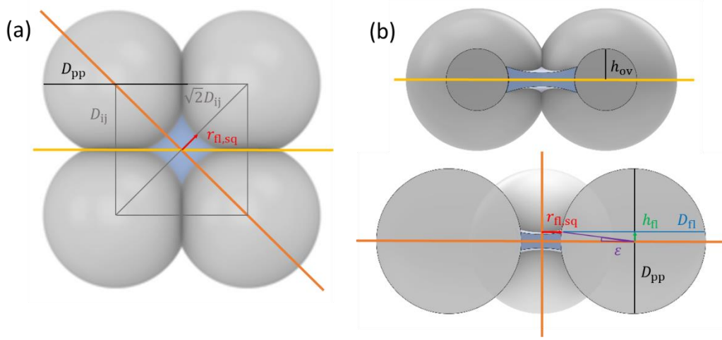
1410 Figure B 6: Illustration of filling of a four-membered ring pore in (a) top view and (b) side views. Bright and dark orange lines indicate the cross sections shown in the side views depicted in panel (b). The pore filling is illustrated for a liquid water filling level to h_{\text{f}} = 1.25 nm, but the same geometry also applies for filling the pore with ice.
