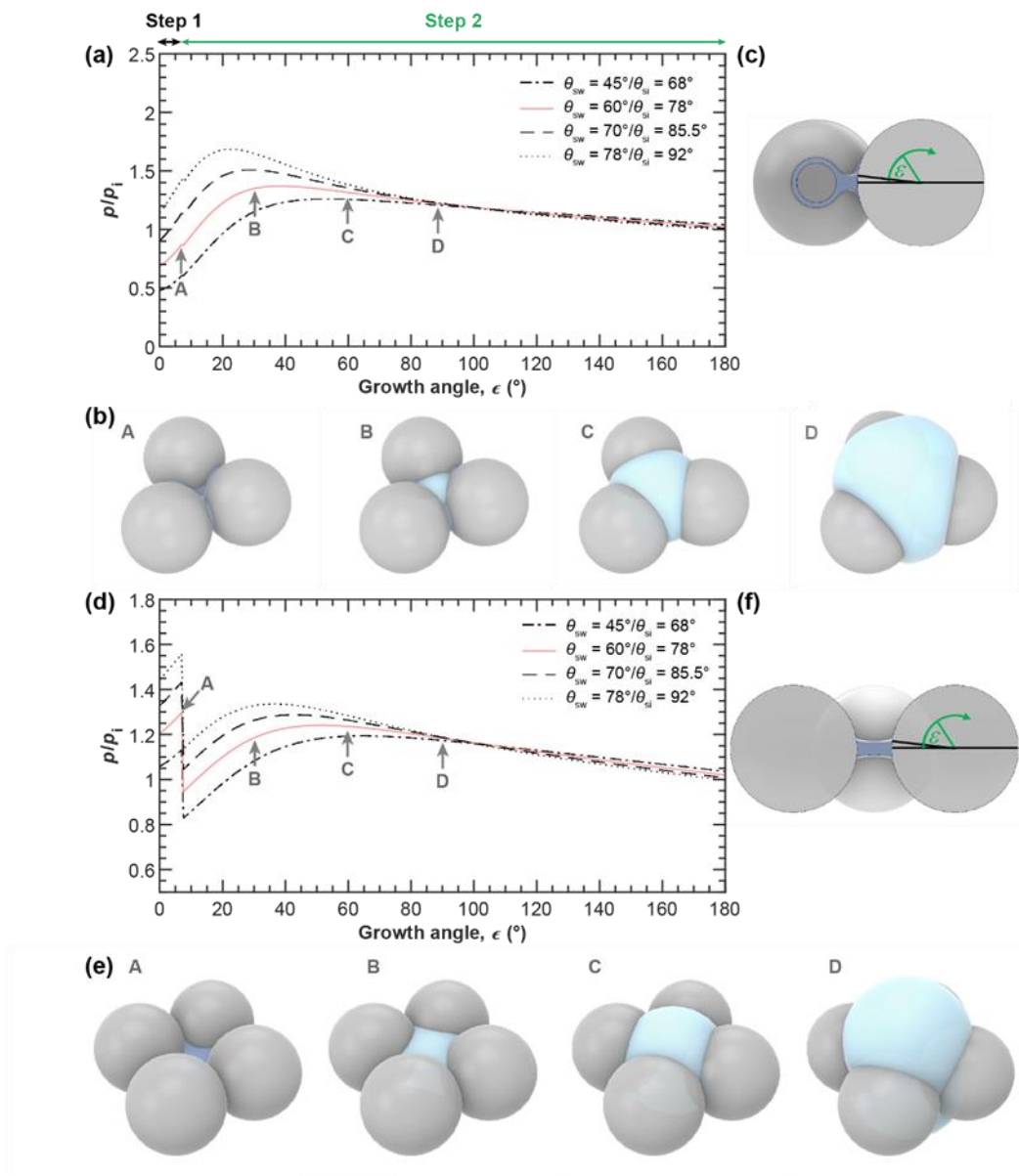
Figure 6: PCF by three-membered (a – c) and four-membered (d – e) ring pores. (a, d) Saturation ratio with respect to ice ( S_i ) required for (step 1) direct filling of the ring pore up to a filling level h_{fl} = h_{fr} = 1.25 nm, followed by (step 2) growth of pore ice as a function of the growth angle \varepsilon , as illustrated in the side views (panels c and f). The 3D renderings illustrate the water growth up to h_{fr} = 1.25 nm (A: darker blue, \varepsilon = 7.18^\circ ) and ice growth (light blue, \varepsilon = 30^\circ (B), 60^\circ (C), and 90^\circ (D)) for a three-membered ring pore with D_{pp} = 20 nm, C_{ov} = 0.05 , and \theta_{sw}(\theta_{si}) = 60^\circ (78^\circ) , panel b) and a four-membered ring pore with D_{pp} = 20 nm, C_{ov} = 0.1 , and \theta_{sw}(\theta_{si}) = 60^\circ (78^\circ) , panel e). All soot-PCF curves were calculated for T = 220 K, D_{pp} = 20 nm, and different contact angles as indicated in the legend. See Figure D 1 and Figure D 2 for soot-PCF curves encompassing different primary particle sizes and overlaps.
