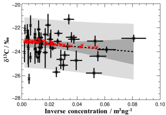
465 Figure 7 Keeling plot depicting the observed levoglucosan \delta^{13}\text{C} vs the inverse concentration (black symbols). Model results are given (red symbols) as well as the line fitted to the experimental data (dashed). The light and dark grey shaded areas represent the 95% prediction and confidence intervals, respectively.
