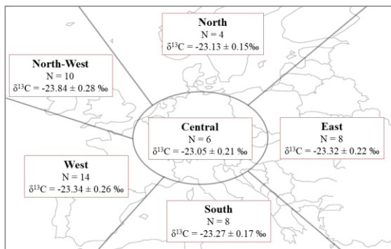
460 Figure 6: Isotopic signatures for different source regions, including corresponding sample number as well as the average \delta^{13}\text{C} . The source regions for the sampled aerosol were designated based on the the main wind direction (see text).
