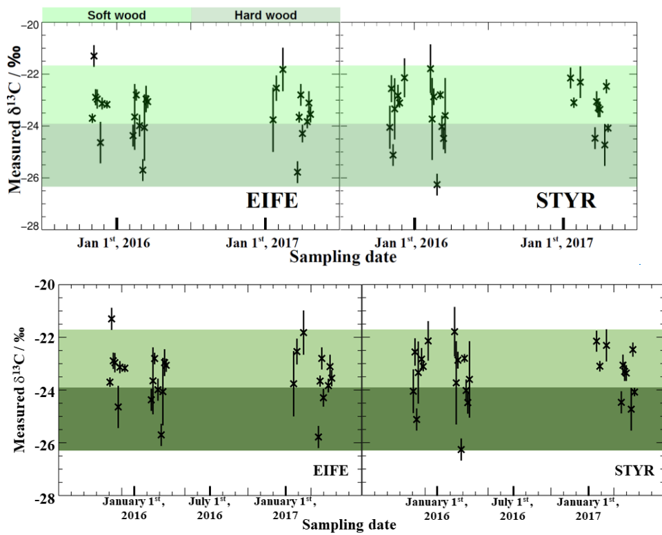
455 Figure 5: \delta^{13}\text{C} of the sampled levoglucosan at EIFE and STYR sites. The shaded areas represent ranges of observed levoglucosan source specific isotope ratios in aerosol formed during the combustion of soft (light green) and hard wood (dark green) (Sang et al., 2012).
