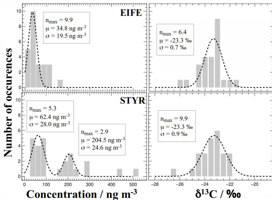
440 Figure 3: Distribution frequency of the observed levoglucosan concentration and δ 13 C.
