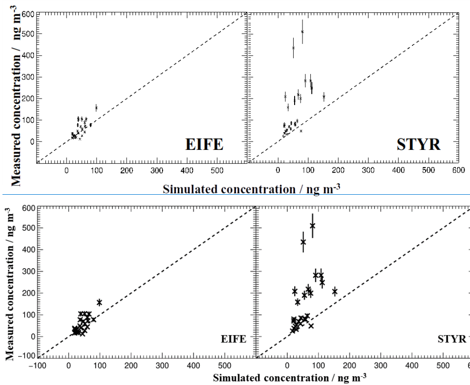
Figure 4: Comparison between observed and simulated levoglucosan concentration at the EIFE and STYR sites. Also the 1:1 line is given (dashed line).
