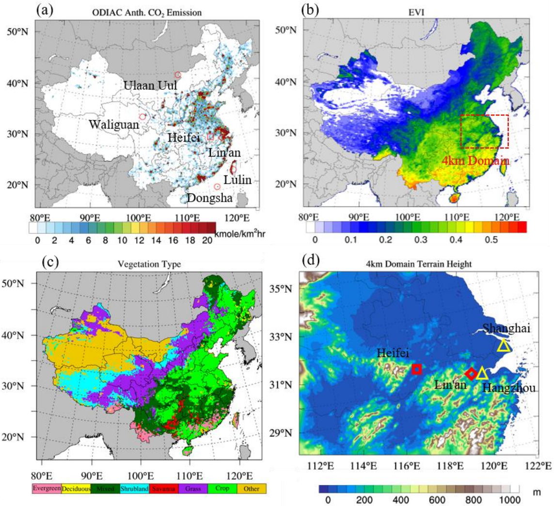
605 Figure 1: Annual averages of (a) ODIAC emission, (b) MODIS EVI, and (c) dominant vegetation type in the 20km simulation domain, and (d) terrain height of the 4km simulation domain. The locations of the ESRL sites, TCCON Hefei site, and Lin'an tower site are indicated with red circles, rectangles, and diamonds respectively in (a). The 4km domain is indicated with the red dash rectangle in (b), and the locations of Hangzhou and Shanghai are indicated with yellow triangles in (d).
