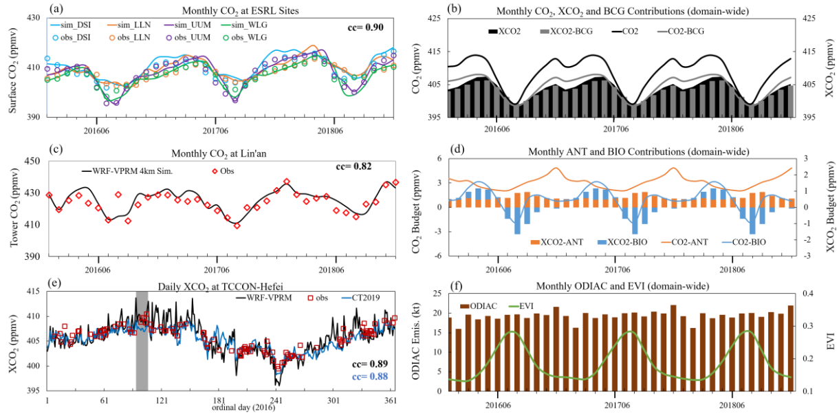
Figure 5: Monthly variations of (a) CO 2 at ESRL sites, (b) total (black) and background (BCG, grey) CO 2 (line) and XCO 2 (area and bar), (c) CO 2 at Lin'an station (averaged for daytime 21m and 55m data); (d) contributions from anthropogenic (ANT, orange) and biogenic (BIO, blue) for CO 2 (lines) and XCO 2 (bars); (f) ODIAC emission and MODIS EVI; and (e) Daily variation of XCO 2 at TCCON-Hefei site.
