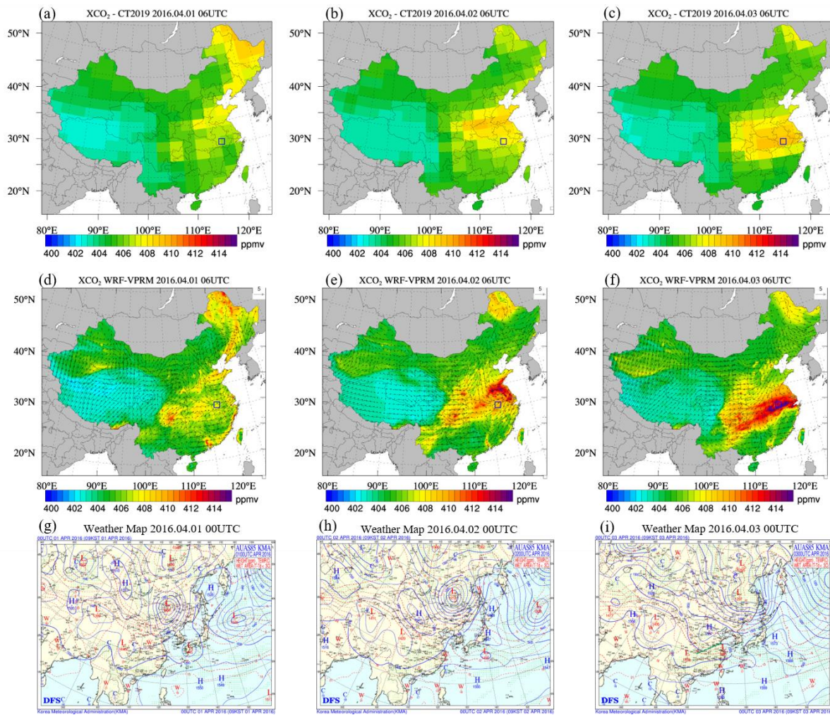
Figure 6: Daily XCO 2 from CT2019 (a-c) and WRF-VPRMChem (d-f), weather map from Korea Meteorological Administration (g-i). The blue box represents location of Hefei.
