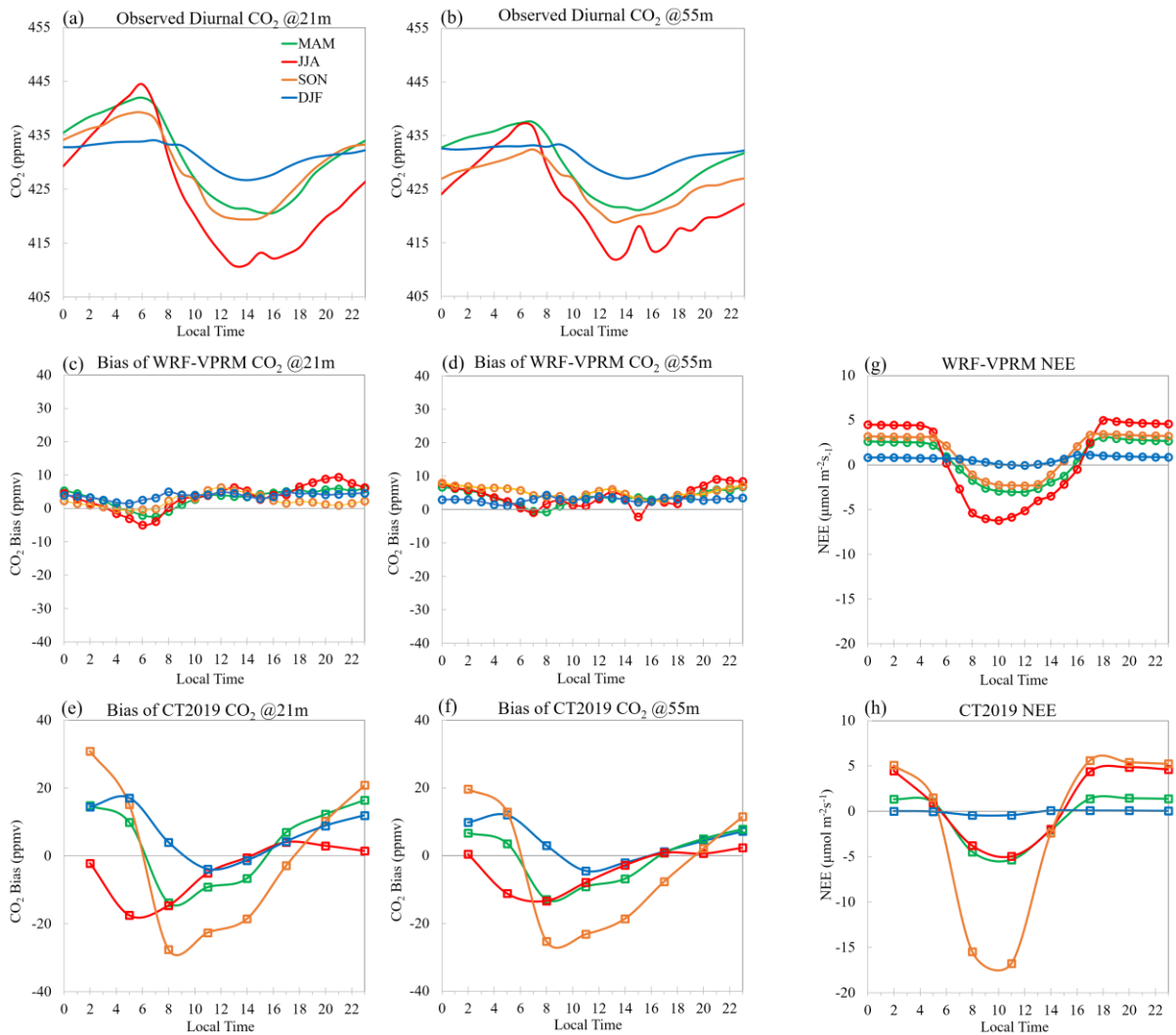
635 Figure 7: Seasonal mean diurnal variations of observed CO 2 at (a) 21m and (b) 55m; WRF-VPRMChem simulation biases of CO 2 at (c) 21m and (d) 55m; CT2019 simulated biases at (e) 21m and (f) 55m; Simulated NEE from (g) WRF-VPRMChem and (h) CT2019.
