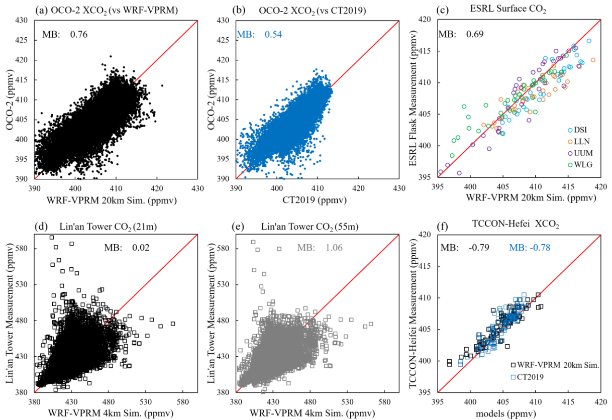
Figure 4: Data pairs for OCO-2 against (a) WRF-VPRM Chem and (b) CT2019; (c) ESRL against WRF-VPRM Chem ; Lin'an tower against WRF-VPRM Chem 4km-grid simulation at (d) 21m and (e) 55m; and (f) TCCON-Hefei against WRF-VPRM Chem and CT2019.
