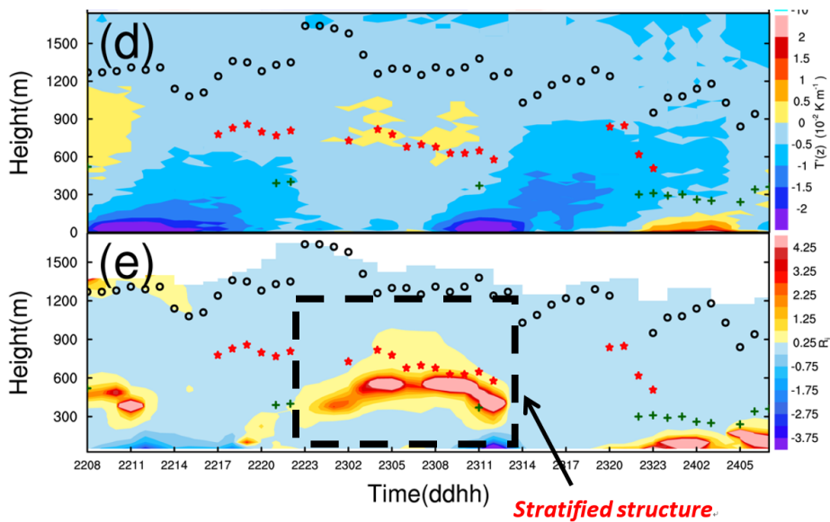
Fig. 3. Fig. 6 The gradient of temperature T'(z) (shaded, units: K km -1 ) measured by MWR (d), and Richardson number (shaded) (e) for type C
