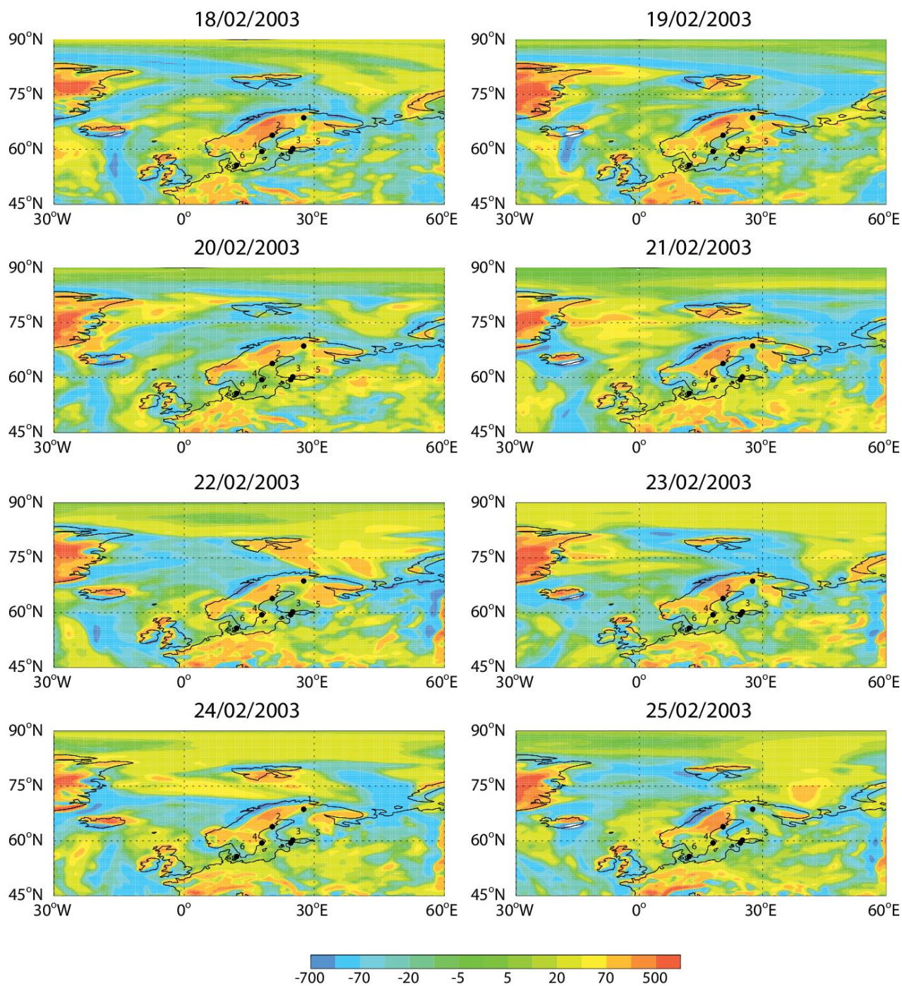
Figure 13. MERRA-2 daily mean pressure vertical velocity (omega) at 940 hPa during February 18-25, 2003. The dots indicate the locations of the sampling sites: 1=Ivalo, 2=Umeå, 3=Helsinki, 4=Kista, 5=Harku, 6=Risø.
