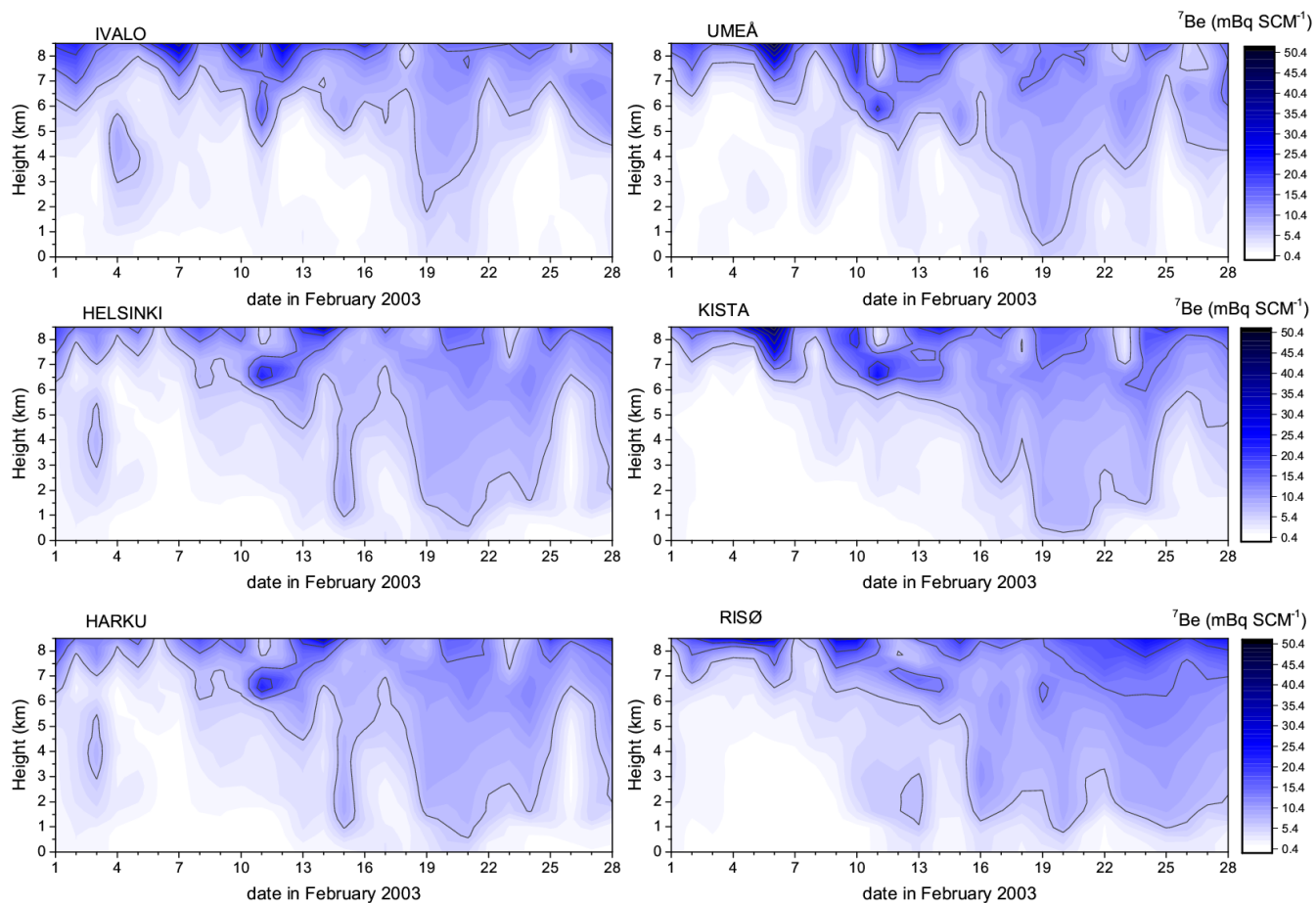
Figure 11. Time-height cross-sections of simulated hourly ^7\text{Be} concentrations (mBq SCM ^{-1} where SCM stands for Standard Cubic Meter) during the month of February 2003 at the six sampling sites.
