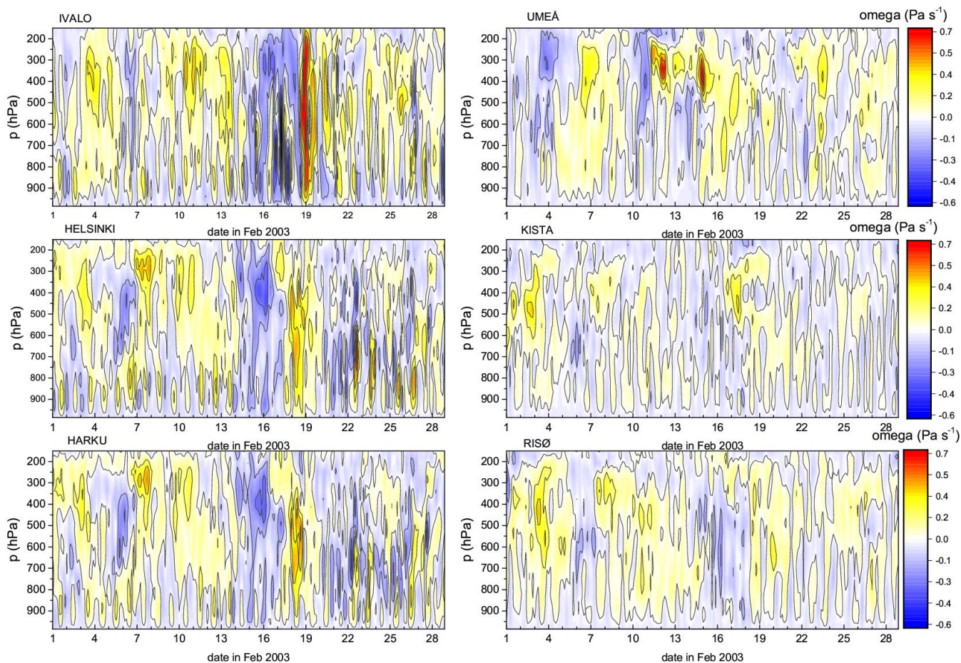
935 Figure 12. Time-height cross-sections of MERRA-2 3-hourly average vertical pressure velocity ( \omega , in \text{Pa s}^{-1} ) during the month of February 2003 sampled at the six sampling sites. Red color indicates large positive \omega values, corresponding to a descending motion, whereas blue color stands for large negative \omega values, corresponding to a rising motion.
