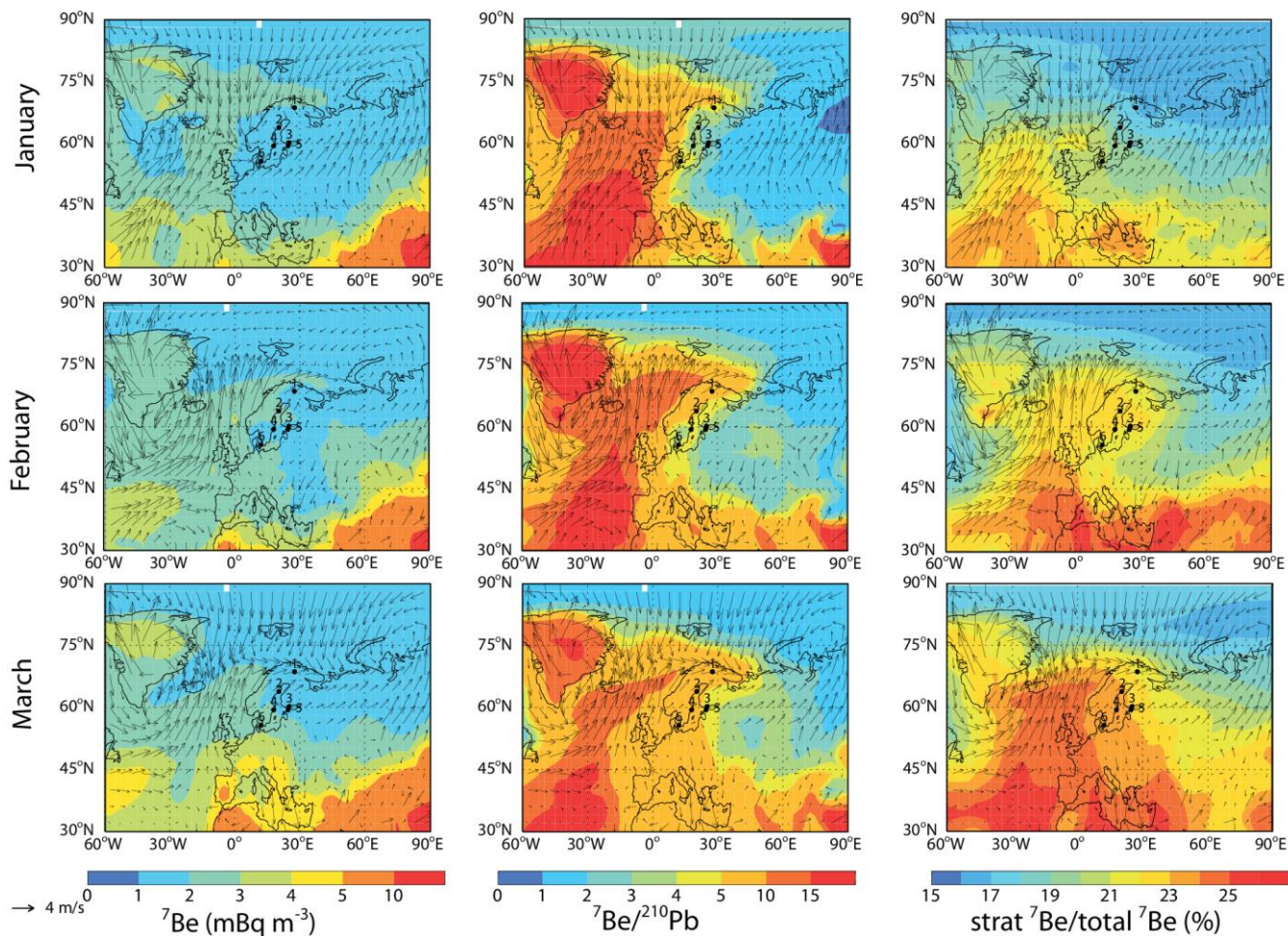
880 Figure 3. Simulated monthly mean ^7\text{Be} surface concentrations ( \text{mBq m}^{-3} ), ^7\text{Be}/^{210}\text{Pb} ratio and fraction of stratospheric ^7\text{Be} . Arrows represent winds in the MERRA-2 reanalysis. The dots indicate the locations of the sampling sites: 1=Ivalo, 2=Umeå, 3=Helsinki, 4=Kista, 5=Harku, 6=Risø.
