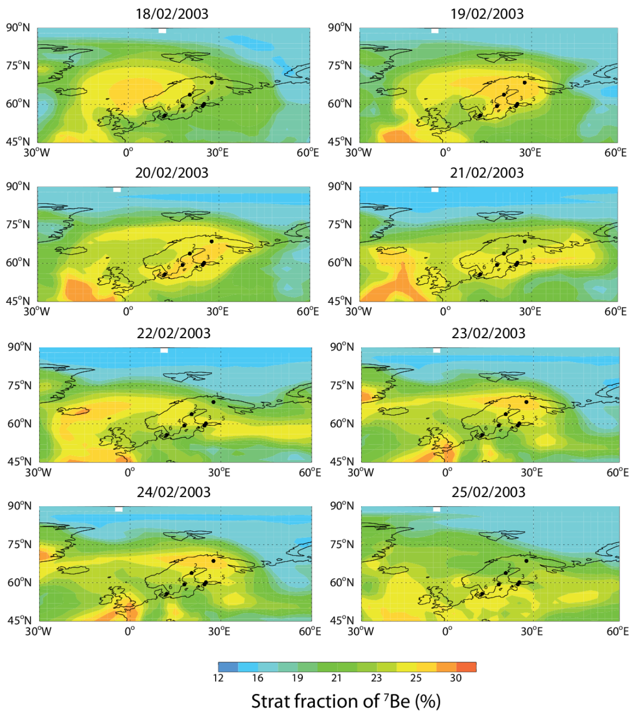
945 Figure 14. Simulated daily mean fraction of ^7\text{Be} originating in the stratosphere (%) at 940 hPa. The dots indicate the locations of the sampling sites: 1=Ivalo, 2=Umeå, 3=Helsinki, 4=Kista, 5=Harku, 6=Risø.
