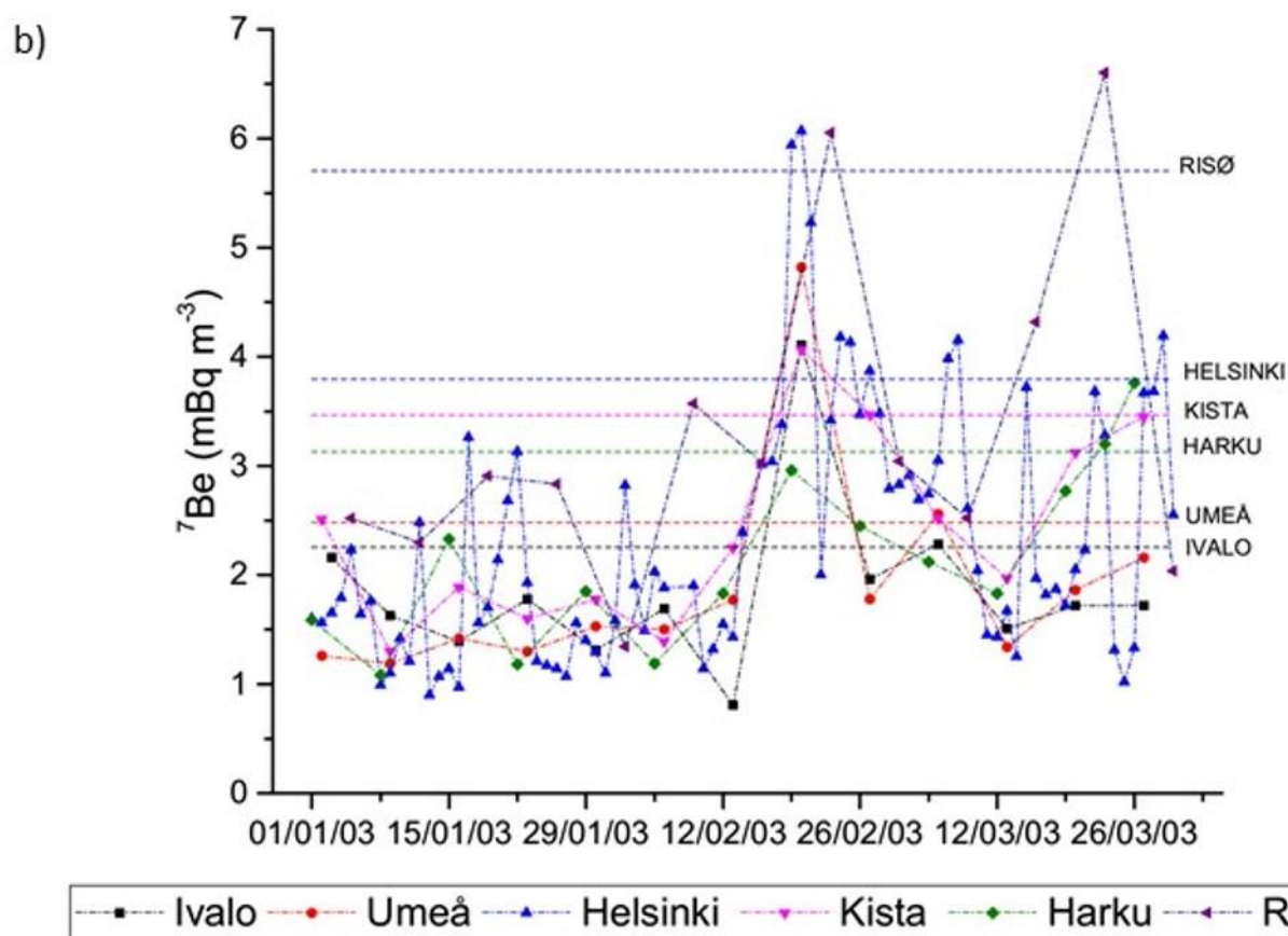
Figure 1. a) Location of the ^7\text{Be} sampling sites in Northern Europe (source: https://mapamundiparaimprimir.com/europa/ ); b) ^7\text{Be} concentrations measured at six surface sampling sites in Northern Europe during the 2002/2003 boreal winter. Dashed lines indicate the 90 th percentile reference line for each sampling site.
