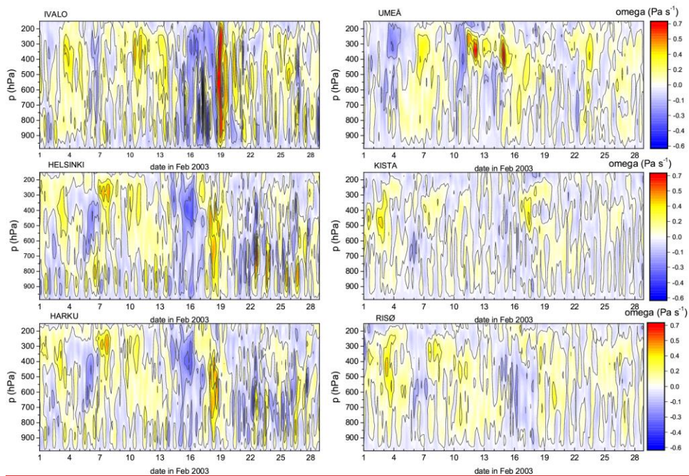
Figure 12. Time-height cross-sections of MERRA-2 3-hourly average vertical pressure vertical-velocity ( \omega , in \text{Pa s}^{-1} ) during the month of February 2003 sampled at the six sampling sites. Red color indicates large positive omega values, corresponding to a descending motion, whereas blue color stands for large negative omega values, corresponding to a rising motion.
