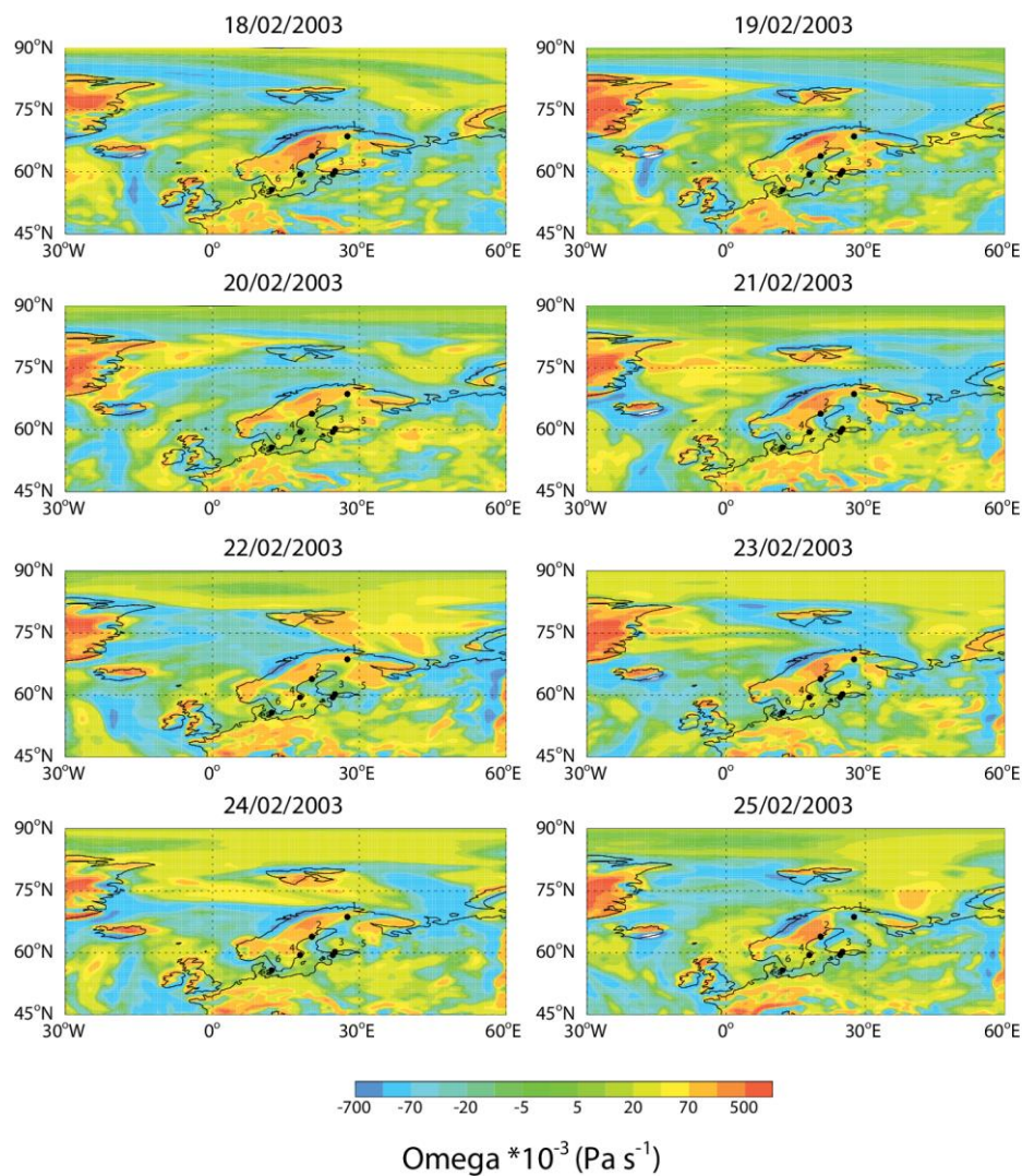
970 Figure 13. MERRA-2 daily mean pressure vertical velocity (omega) at 940 hPa during February 18-25, 2003. The dots indicate the locations of the sampling sites: 1=Ivalo, 2=Umeå, 3=Helsinki, 4=Kista, 5=Harku, 6=Risö.
