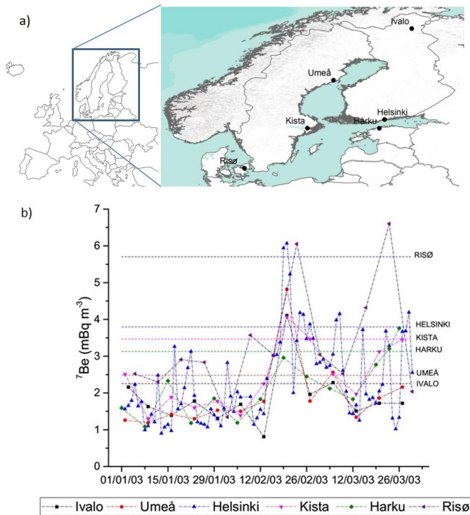
Figure 1. a) Location of the ^7\text{Be} sampling sites in Northern Europe (source: https://mapamundiparaimprimir.com/europa/ ); b) ^7\text{Be} concentrations measured at six surface sampling sites in Northern Europe during the 2002/2003 boreal winter. Dashed lines indicate the 90 th percentile reference line for each sampling site.
