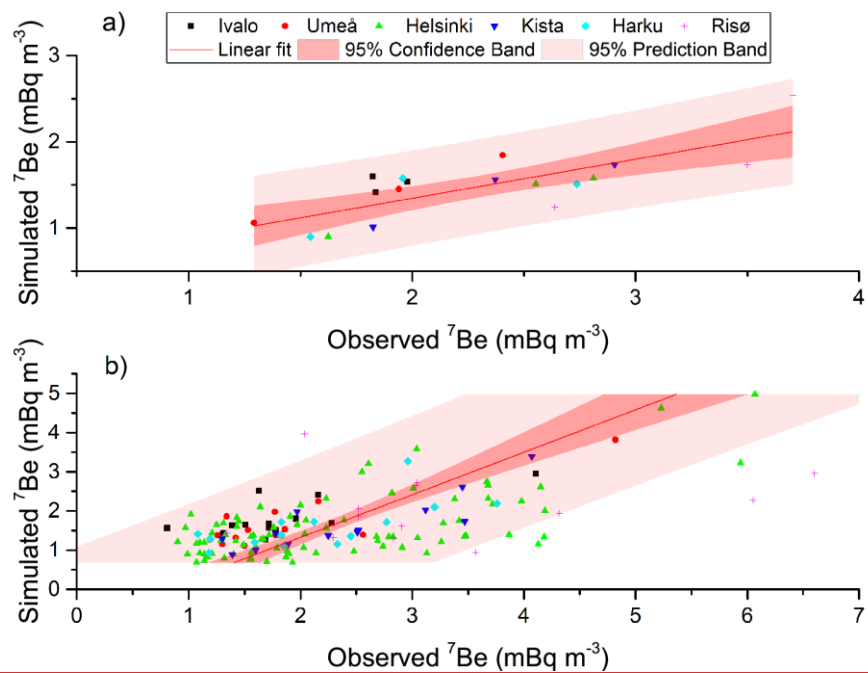
Figure 4. Scatter plots of: a) simulated vs. observed ^7\text{Be} monthly means at the six sampling sites; b) simulated vs. observed ^7\text{Be} weekly (daily in the case of Helsinki) means at the six sampling sites. Also shown are the linear regression line and the 95% confidence and prediction bands around the linear fit.
