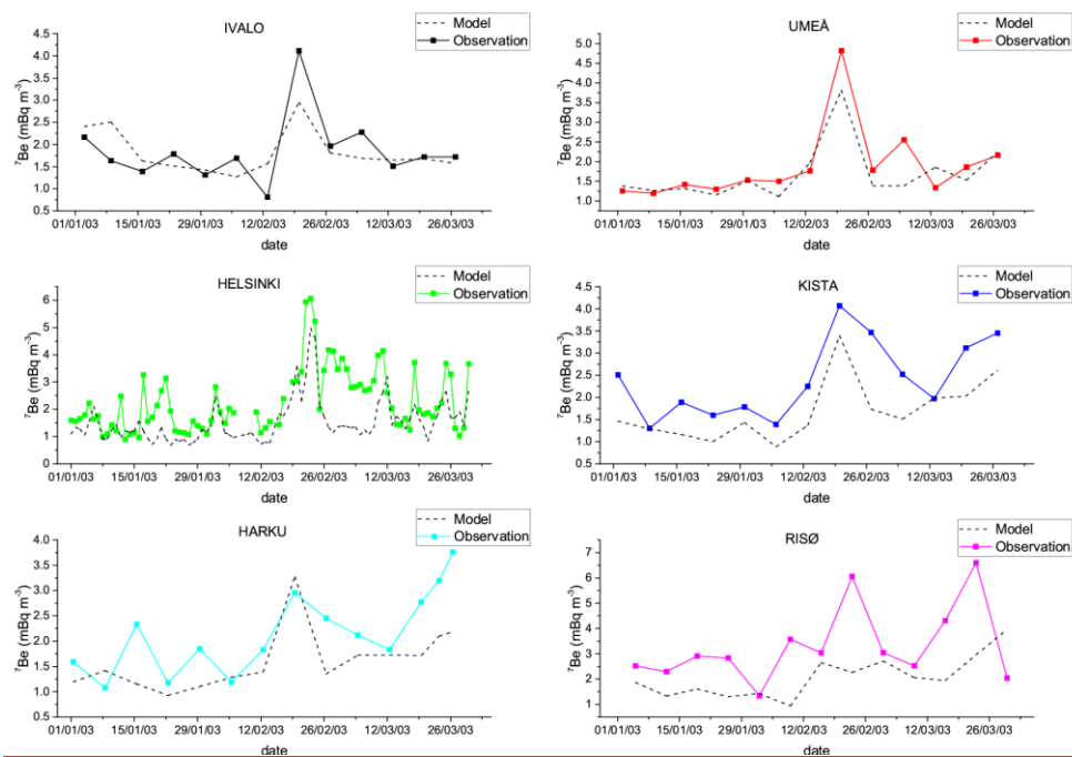
920 Figure 5. Temporal evolution of simulated and observed ^7\text{Be} surface concentrations at the six sampling sites. Values are weekly (daily in the case of Helsinki) means.
