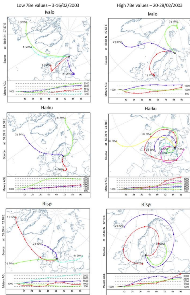
Figure 15. Average trajectory cluster results (centroids) in Ivalo, Harku and Risø Risø at 1000 m for low ^7\text{Be} values (left: 3-16 February 2003) and high ^7\text{Be} values (right: 20-28 February 2003), respectively. The stations are ordered by latitude from top to bottom (coordinates of the receptor site are provided on the left of each plot). The right numbers between brackets in
