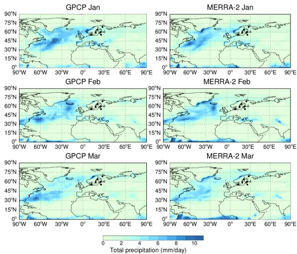
Figure 2. Comparison of the MERRA-2 total precipitation during January-March 2003 with the GPCP observations. The black dots indicate the locations of the sampling sites: 1=Ivalo, 2=Umeå, 3=Helsinki, 4=Kista, 5=Harku, 6=Risö.
