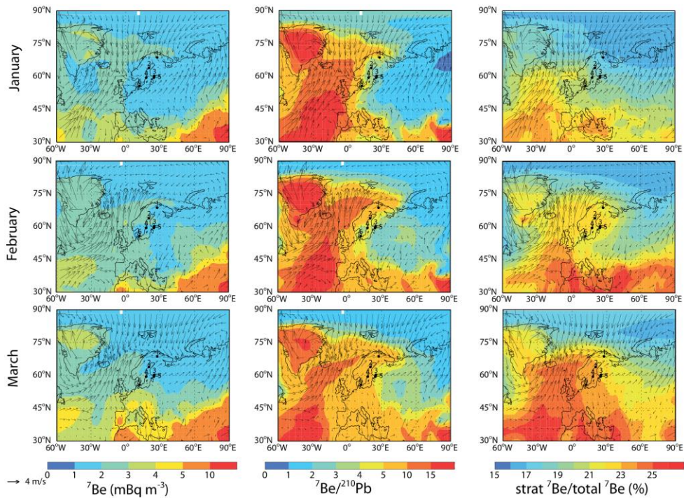
Figure 3. Simulated monthly mean ^7\text{Be} surface concentrations ( \text{mBq m}^{-3} ), ^7\text{Be}/^{210}\text{Pb} ratio and fraction of stratospheric ^7\text{Be} . Arrows represent winds in the MERRA-2 reanalysis. The dots indicate the locations of the sampling sites: 1=Ivalo, 2=Umeå, 3=Helsinki, 4=Kista, 5=Harku, 6=Riise.
