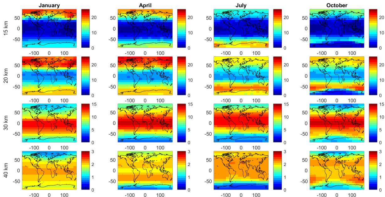
220 Figure 9. Climatological ozone distributions (in DU/km), for January, April, July, and October, for selected altitude levels (15, 20, 30, and 40 km).
