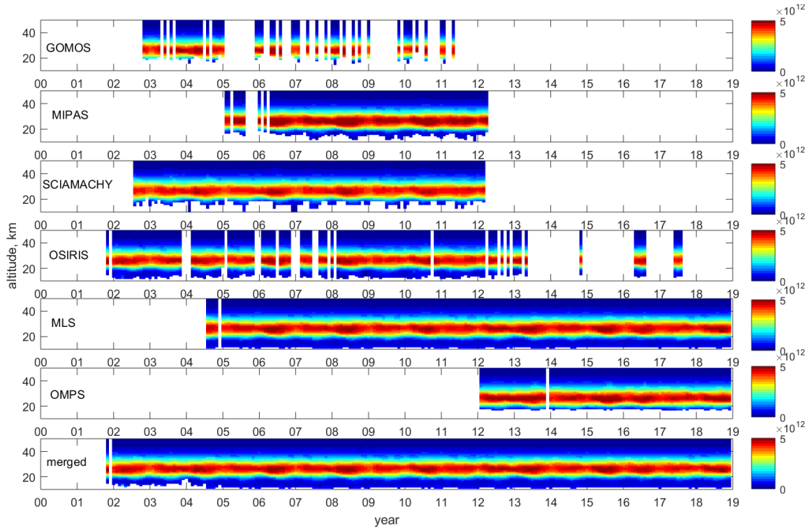
Figure 8. An example of number density ozone profiles (in \text{cm}^{-3} ) for individual instruments and the merged dataset in the spatial bin 0-10° N, 0-20° E.
