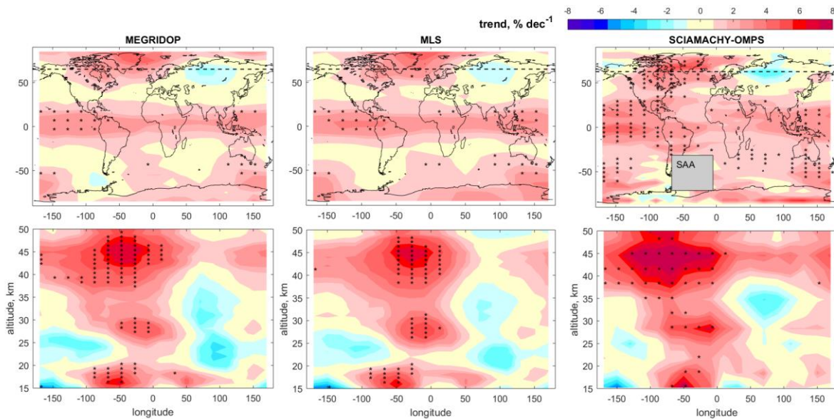
270 Figure 12. Top: ozone trends in late 2004- 2018 (% decade -1 ) at 35 km, bottom: longitude –altitude cross section of the ozone trends at ~ 65 °N (the latitude is indicated by dashed line on top panels). Ozone trends are estimated using the MEGRIDOP (left), MLS (center), and SCIAMACHY-OMPS datasets (right). For the SCIAMACHY-OMPS dataset, ozone trends in the Southern Atlantic Anomaly (SAA) region are not shown, because SCIAMACHY data are flagged in this region.
