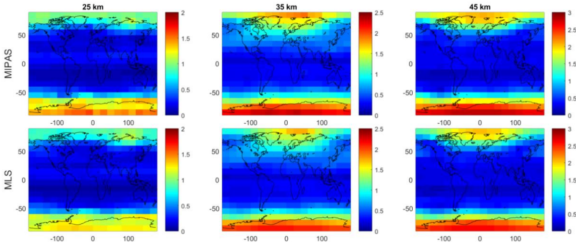
140 Figure 4. Relative amplitude of seasonal cycle at 25 km (left), 35 km(center) and 45 km(right) for MIPAS (top) and MLS (bottom).
