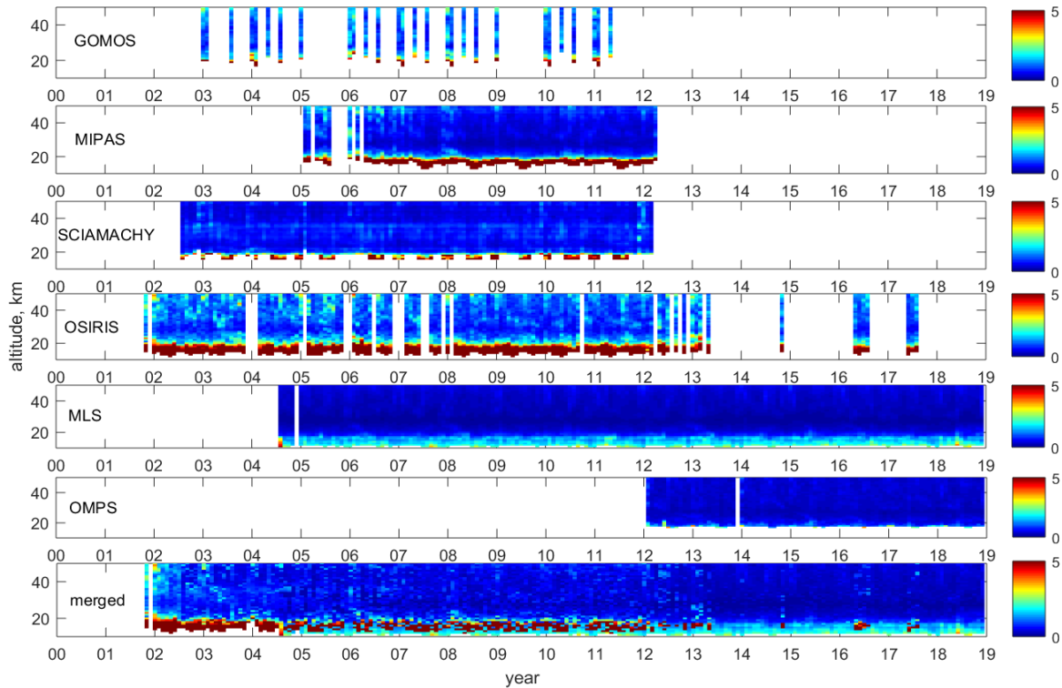
Figure 7. An example of uncertainties in deseasonalized anomalies (in %) for individual instruments and the merged dataset in the spatial bin 0-10° N, 0-20° E
