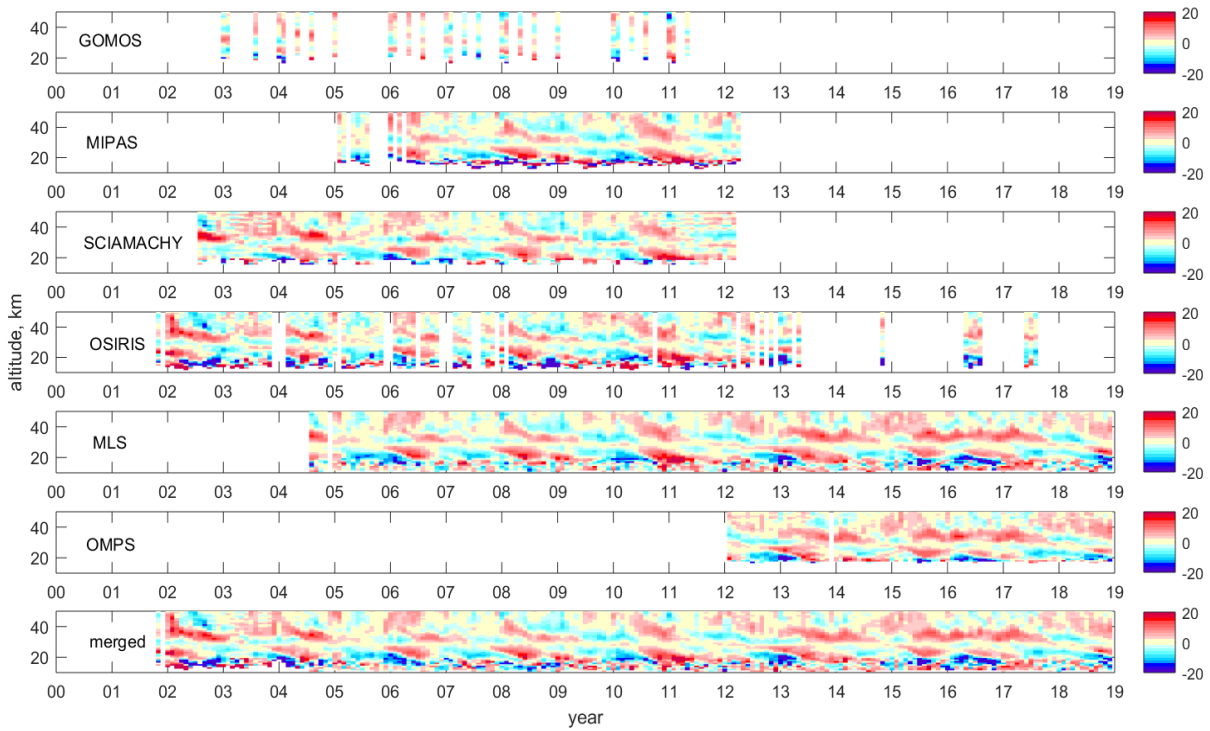
190 Figure 6 . An example of deseasonalized anomalies (in %) for individual instruments and the merged dataset in the spatial bin 0-10° N, 0-20° E.
