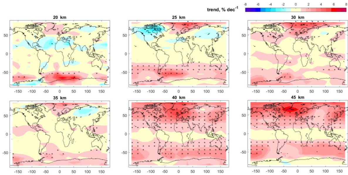
265 Figure 10. Ozone trends ( \% \text{ decade}^{-1} ) in 2003-2018, for several altitudes. Statistically significant trends are indicated by stars.
