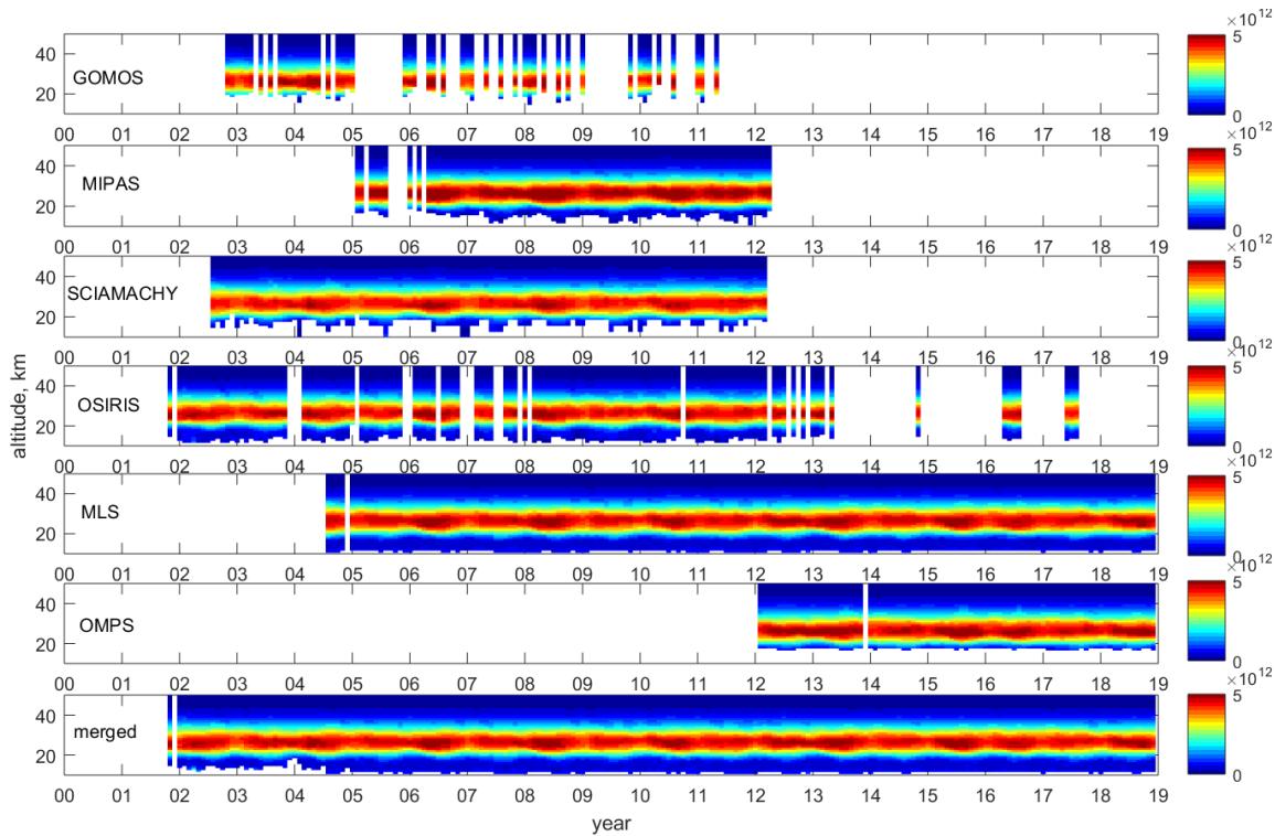
215 Figure 8. An example of number density ozone profiles (in \text{cm}^{-3} ) for individual instruments and the merged dataset in the spatial bin 0\text{-}10^\circ \text{ N} , 0\text{-}20^\circ \text{ E} .
