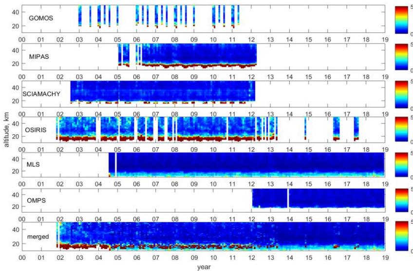
Figure 7. An example of uncertainties in deseasonalized anomalies (in %) for individual instruments and the merged dataset in the spatial bin 0-10° N, 0-20° E
