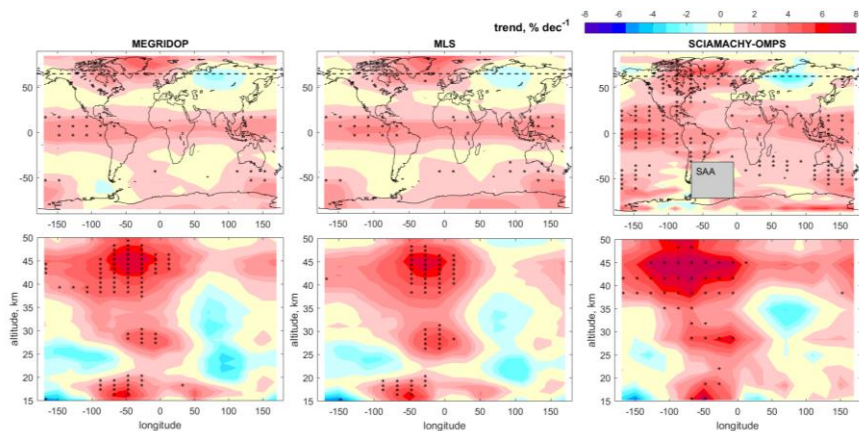
Figure 12. Top: ozone trends in late 2004- 2018 (% decade -1 ) at 35 km, bottom: longitude –altitude cross section of the ozone trends at ~ 65 °N (the latitude is indicated by dashed line on top panels). Ozone trends are estimated using the MEGRIDOP (left), MLS (center), and SCIAMACHY-OMPS datasets (right). For the SCIAMACHY-OMPS dataset, ozone trends in the Southern Atlantic Anomaly (SAA) region are not shown, because SCIAMACHY data are flagged in this region.
