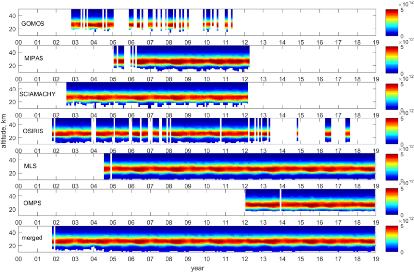
Figure 8. An example of number density ozone profiles (in \text{cm}^{-3} ) for individual instruments and the merged dataset in the spatial bin 0-10° N, 0-20° E.
