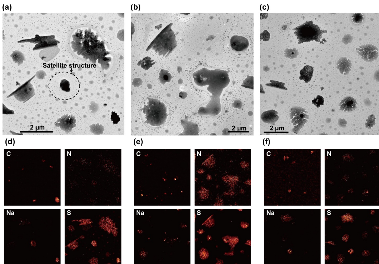
Figure 11. TEM and elemental mapping images of the sulfate particles. Top (a)-(c): TEM images.
