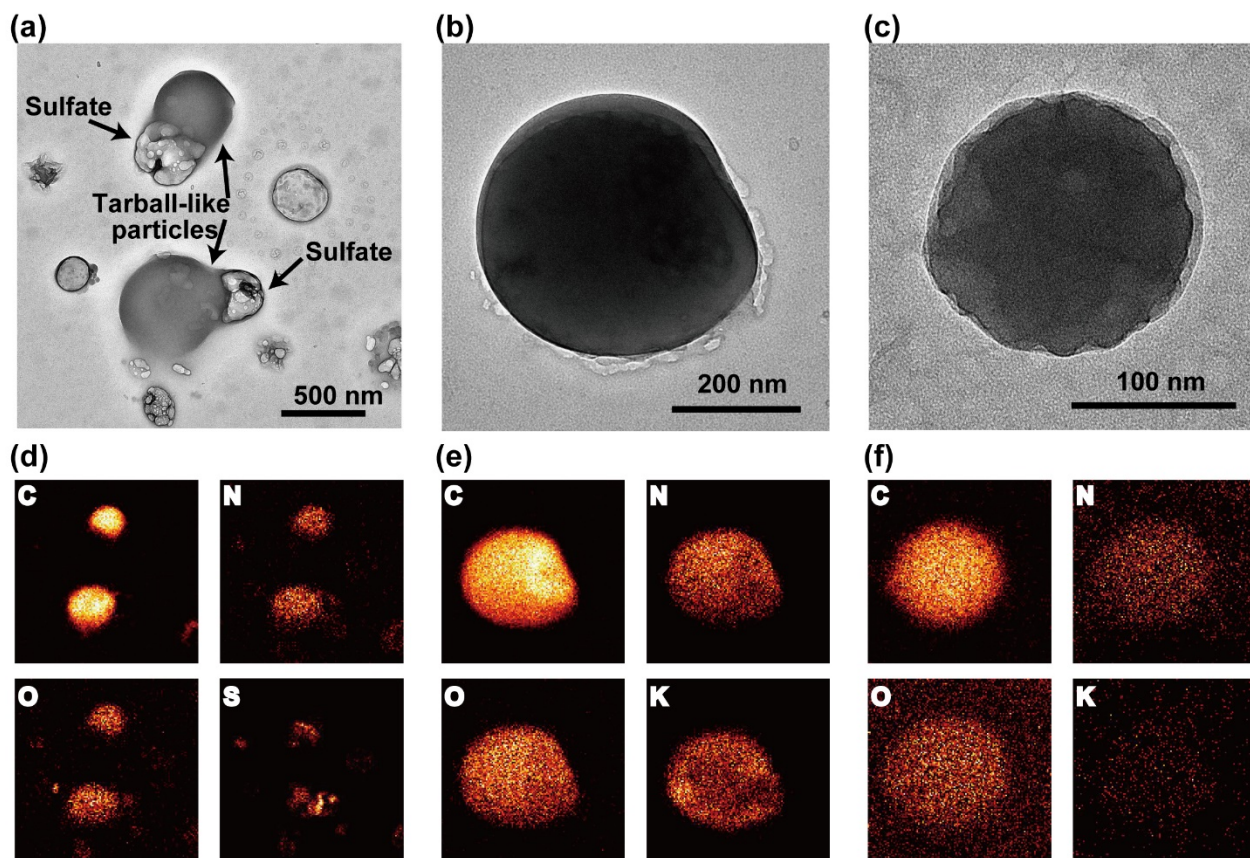
Figure 12. TEM and elemental mapping images of the tarball and tarball-like particles in a BB sample (10:30-10:59, 2 April 2018). (a) TEM image of the tarball-like particles containing sulfate. As they exhibit deformed spherical shapes and the characteristic elements of tarballs (e.g., C, N, O, and K), we label them tarball-like particles. Other examples of tarballs are shown in (b) and (c). (d)-(f): Elemental mapping images of the TEM areas.
