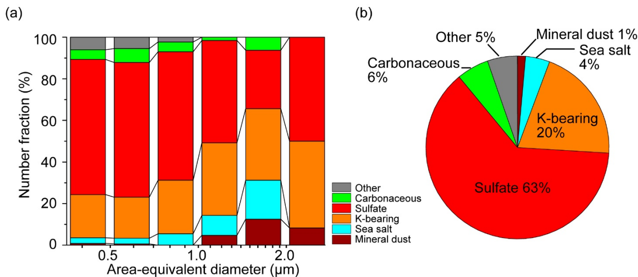
965 Figure 5. Number fractions of the aerosol particles in the BB samples. (a) Size-dependent and (b) total number fractions. Three BB samples were collected on 2, 3, and 4 April. The size bins are shown on a log-scale and are 0.35-0.5, 0.5-0.71, 0.71-1.00, 1.00-1.41, 1.41-2.00, and > 2.00 \mu\text{m} . (b) Number fractions of the total particles of the BB samples. The particle number of the BB samples is 1041.
