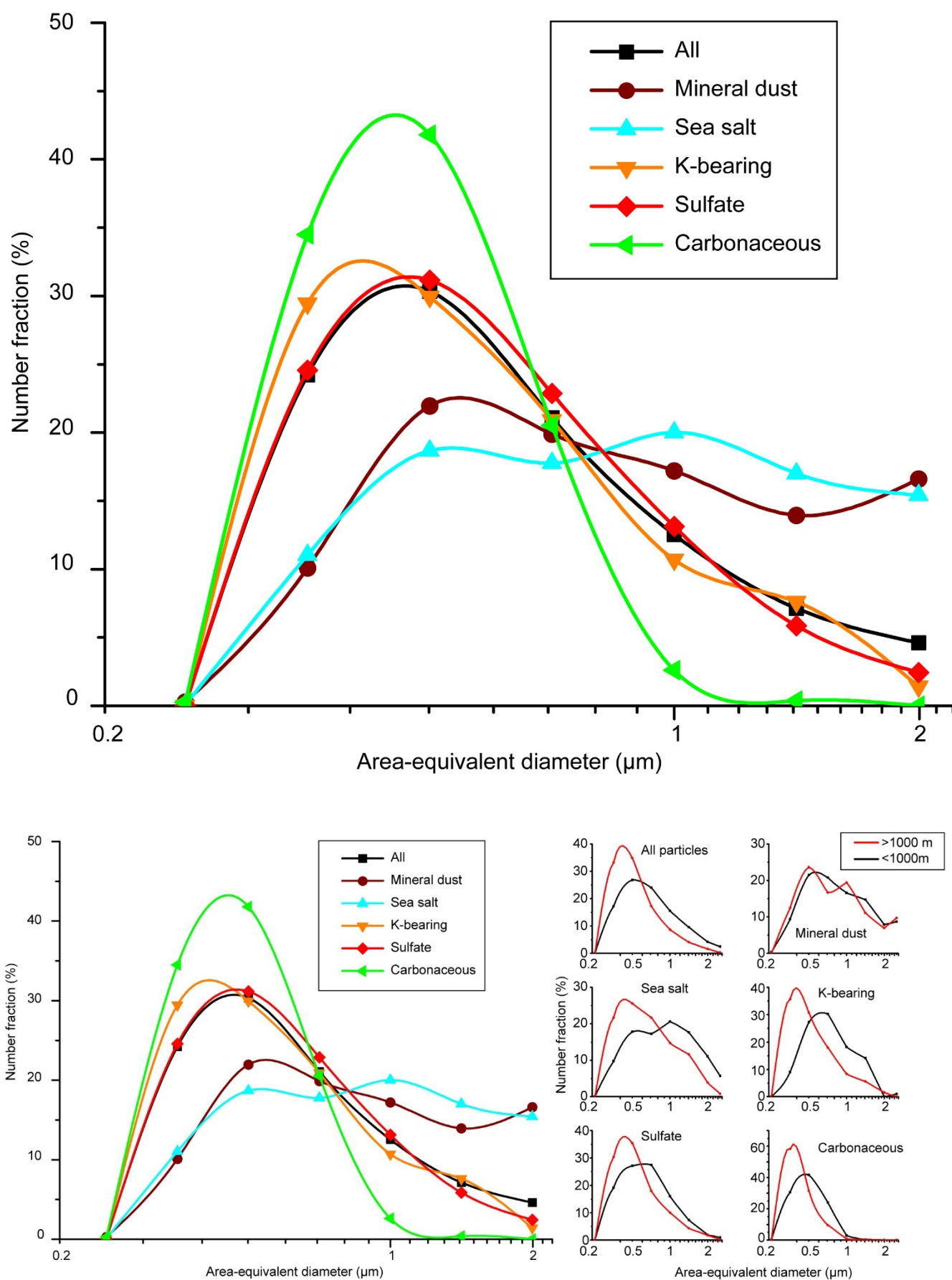
945 Figure 2. Normalized size distributions of each particle type for all samples (left) and for samples at altitudes above and below 1000 m (right). The particle sizes were determined from the area-equivalent
