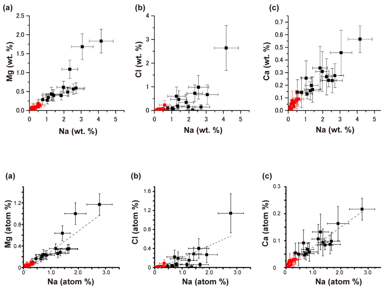
Figure 9. Relations of Na with Mg, Cl, and Ca among all particles. The plots show the average atomicweight percent values of all particles within each sample. The black and red plots are the samples < 1000 m and > 1000 m, respectively. R^2 values are 0.84, 0.61, and 0.89 for (a), (b), and (c), respectively. Approximated curves are shown in the gray dashed lines. The error bars indicate the 95% confidential intervals.
