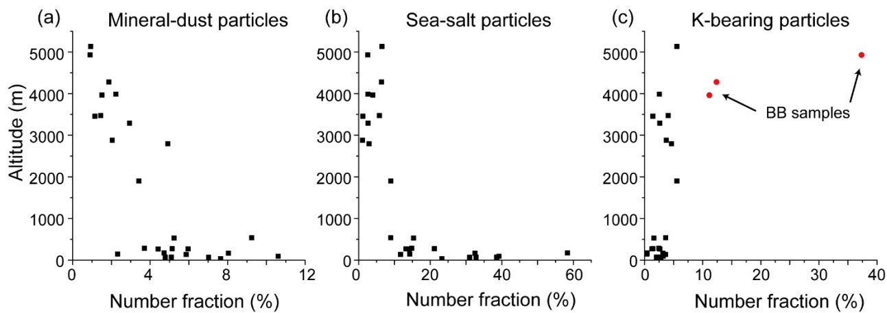
Figure 4. Vertical changes in the number fractions (%) of (a) mineral-dust, (b) sea-salt, and (c) K-
