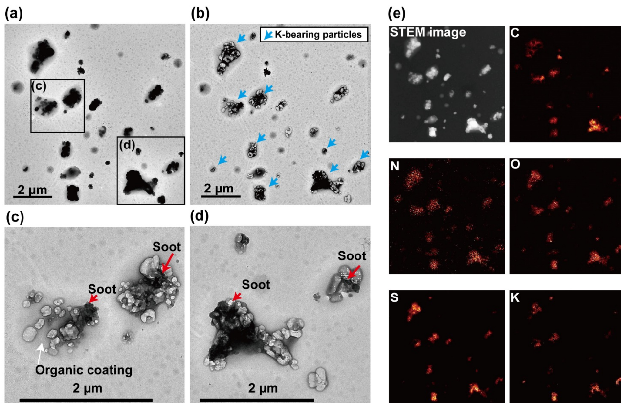
Figure 6. TEM and elemental mapping images of a BB sample (10:40-10:59, 2 April 2018). (a) TEM image of K-bearing particles. (b) The same area of the TEM image (a) but after the STEM-EDS analysis. Beam-sensitive materials are removed, and soot inclusions are more apparent. (c) and (d): Examples of K-bearing particles containing soot inclusions and organic coatings, which appear in gray in the TEM image. (e) STEM and elemental mapping images for C, N, O, S, and K in the TEM image. The distributions of K, S, and O correspond to the K-bearing particles, and that of C represents the soot and organic particles.
