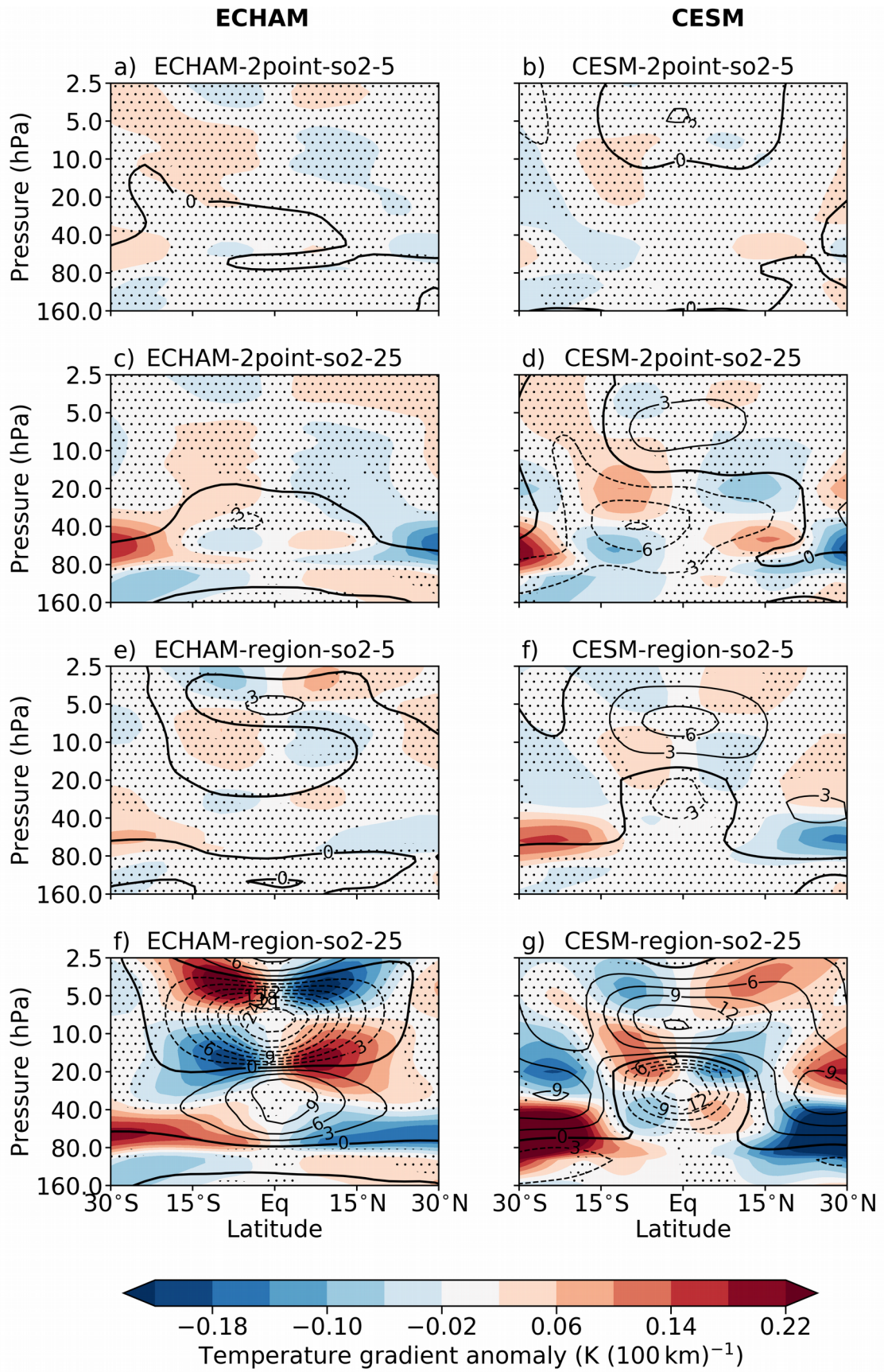
Figure S6: As Figure 12, but for the corresponding injection of \text{SO}_2 .
