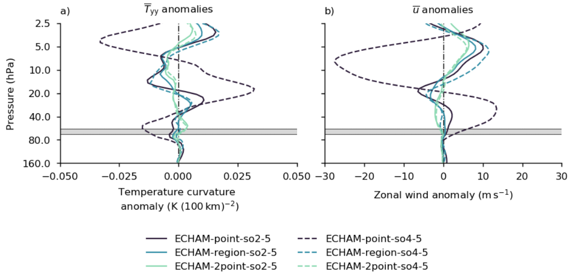
Figure S4: As Figure 8, but for the corresponding injection with an injection rate of 5 \text{ Tg(S)yr}^{-1} .
