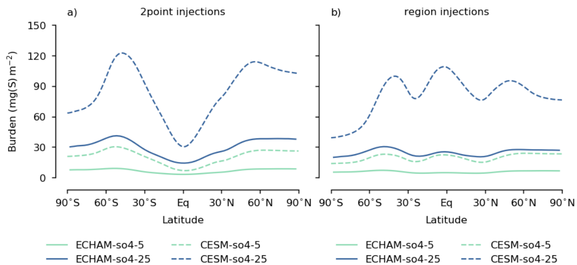
Figure S7: As Figure 13, but for the corresponding injection of SO 2 .
