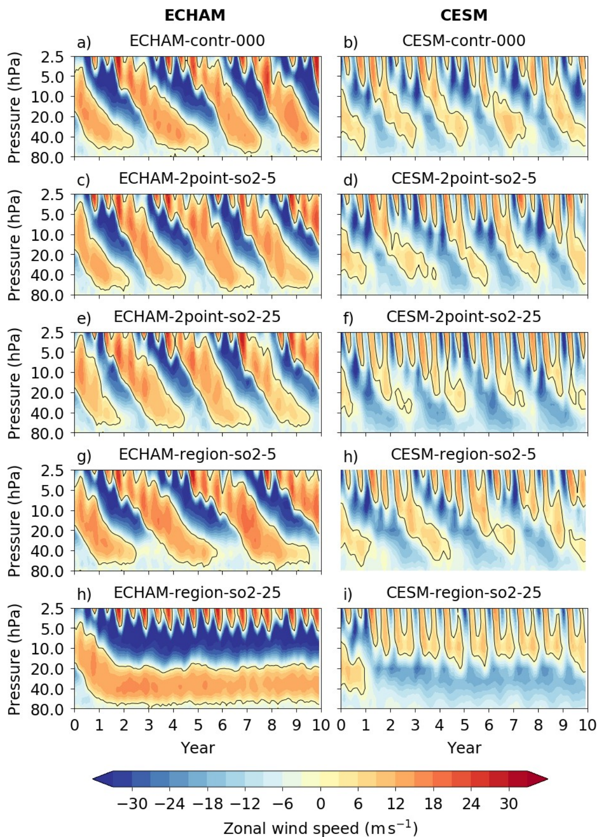
Figure S5: As Figure 11, but for the corresponding injection of SO 2 .
