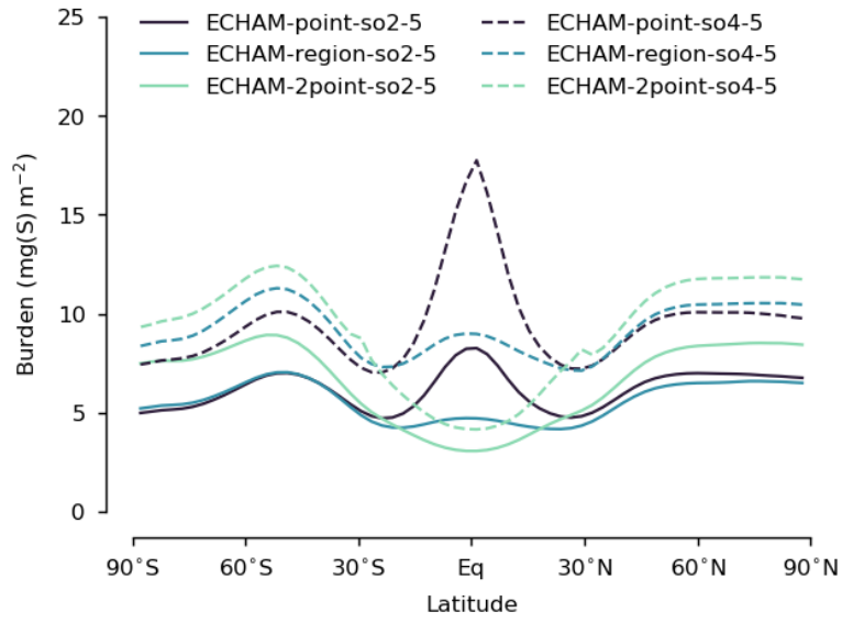
Figure S3: As Figure 7, but for the corresponding injection with an injection rate of 5 \text{ Tg(S)yr}^{-1} .
