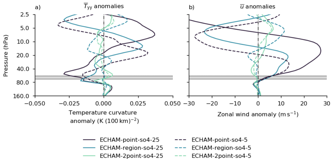
Figure S2: As Figure 6, but for the corresponding injection of SO 2 .
