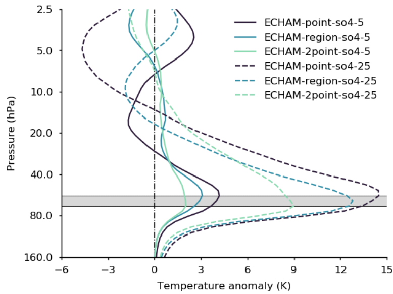
Figure S1: As Figure 4, but for the corresponding injection of AM-SO 4 .
