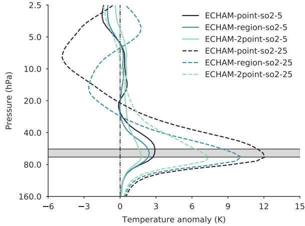
Figure 6. Vertical profile of the 5^{\circ} N to 5^{\circ} S mean temperature anomaly for the 5 and 25 Tg(S) \text{yr}^{-1} injections simulated with ECHAM. The horizontal grey bar marks the injection layer. The vertical dashed-dotted line marks a temperature anomaly of 0 K.
