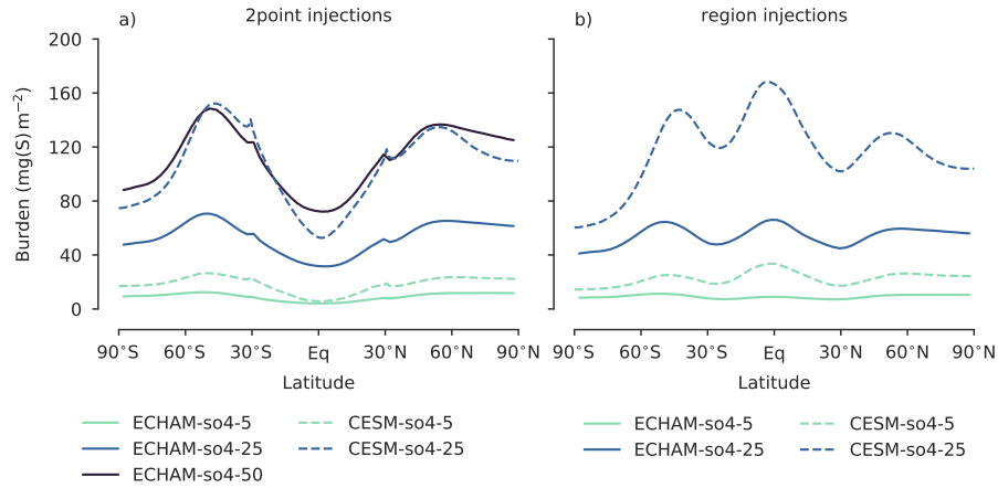
Figure 14. Zonal mean artificial sulfate burden for the 2point injections (a) and the region injections (b) of \text{AM-SO}_4 as a function of latitude. Solid lines indicate the ECHAM simulations, dashed lines indicate the CESM simulations. The artificial sulfate burden can be used as a very basic proxy for the amount of heating due to absorption of OTLR and NIRr.
