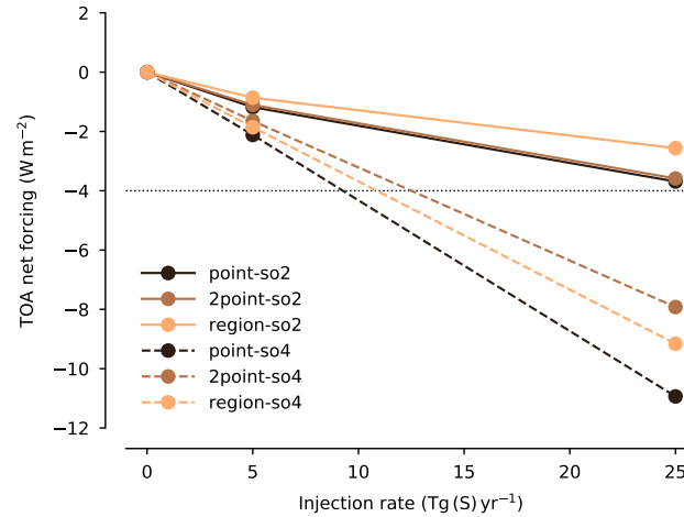
Figure 11. Global mean TOA all-sky net RF exerted by artificial sulfate aerosols as a function of injection rate. The dashed-dotted black line marks a RF of -4 \text{ W m}^{-2} .
