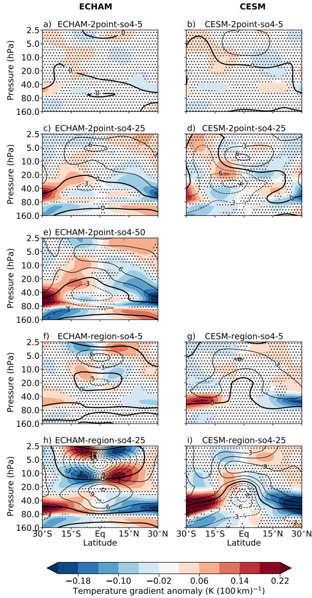
Figure 13. Latitude-height cross sections of the anomaly of the meridional zonal mean temperature gradient \overline{T}_y for the AM-SO 4 injection scenarios in ECHAM (left column) and in CESM (right column). Stippling indicates areas where anomalies are not significant at the 95 % level in a student's t -test. Black contour lines indicate the anomaly of the zonal mean zonal wind speed \overline{u} in intervals of 3 \text{ m s}^{-1} , with the thick black line denoting \overline{u}=0 \text{ m s}^{-1} . Solid lines denote a westerly anomaly, while dashed lines denote an easterly anomaly. The 1 st row shows the 2point injections of 5 \text{ Tg(S) yr}^{-1} , the 2 nd row shows the 2point injections of 25 \text{ Tg(S) yr}^{-1} , the 4 th row shows the region injections of 5 \text{ Tg(S) yr}^{-1} , and the 5 th row shows the region injections of 25 \text{ Tg(S) yr}^{-1} . The 2point injection of 50 \text{ Tg(S) yr}^{-1} was only performed with ECHAM and is shown in the 3 rd row.
