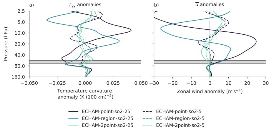
Figure 7. Vertical profile of the 5^{\circ} N to 5^{\circ} S mean anomaly of the temperature curvature \overline{T}_{yy} (a) and the tropical mean anomaly of the zonal wind \overline{u} (b) for the ECHAM simulations of a \text{SO}_2 injection with an injection rate of 5 \text{ Tg(S) yr}^{-1} (dashed) and 25 \text{ Tg(S) yr}^{-1} (solid). The horizontal grey bar marks the injection layer. The vertical dashed-dotted line marks an anomaly of 0 \text{ K (100 km)}^{-2} (a) and 0 \text{ m s}^{-1} (b).
