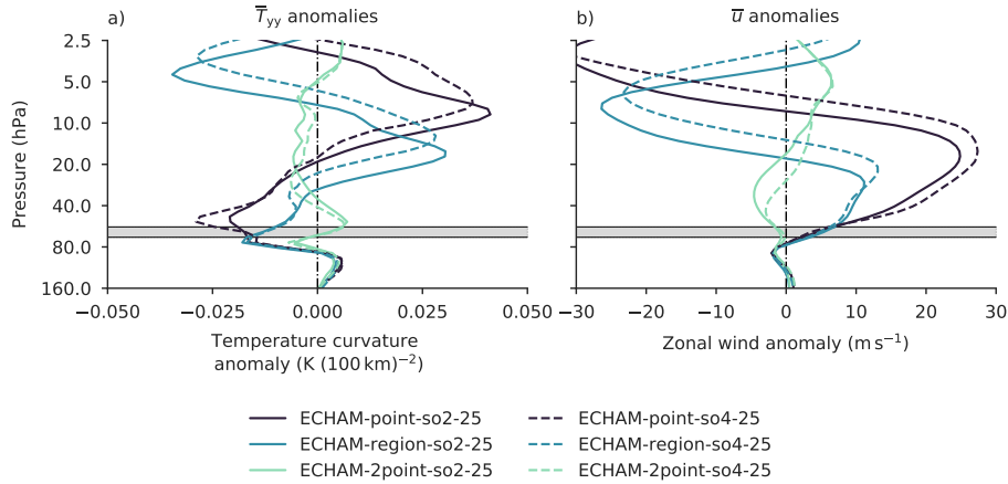
Figure 9. Vertical profile of the 5^\circ \text{ N} to 5^\circ \text{ S} mean anomaly of the temperature curvature \bar{T}_{yy} (a) and the tropical mean anomaly of the zonal wind \bar{u} (b) for the ECHAM simulations of injections with an injection rate of 25 \text{ Tg(S) yr}^{-1} . The horizontal grey bar marks the injection layer. The vertical dashed-dotted line marks an anomaly of 0 \text{ K (100 km)}^{-2} (a) and 0 \text{ m s}^{-1} (b).
